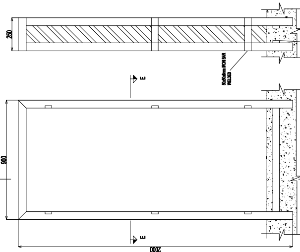
DOOR FRAME DETAIL scale:1/20
