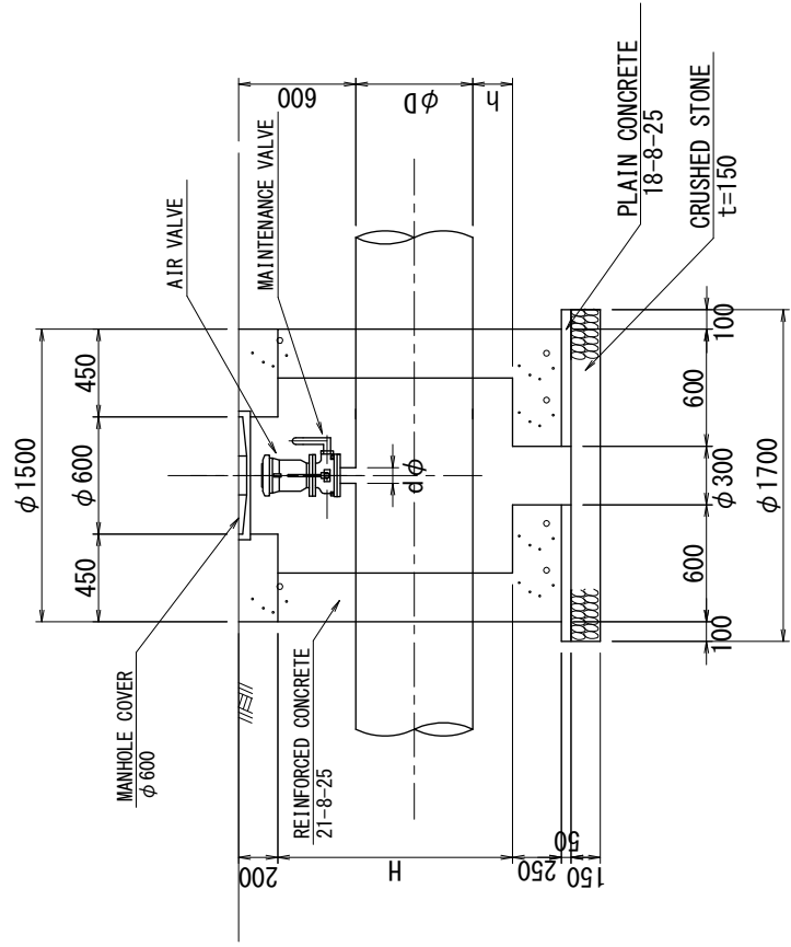
Cross Section
