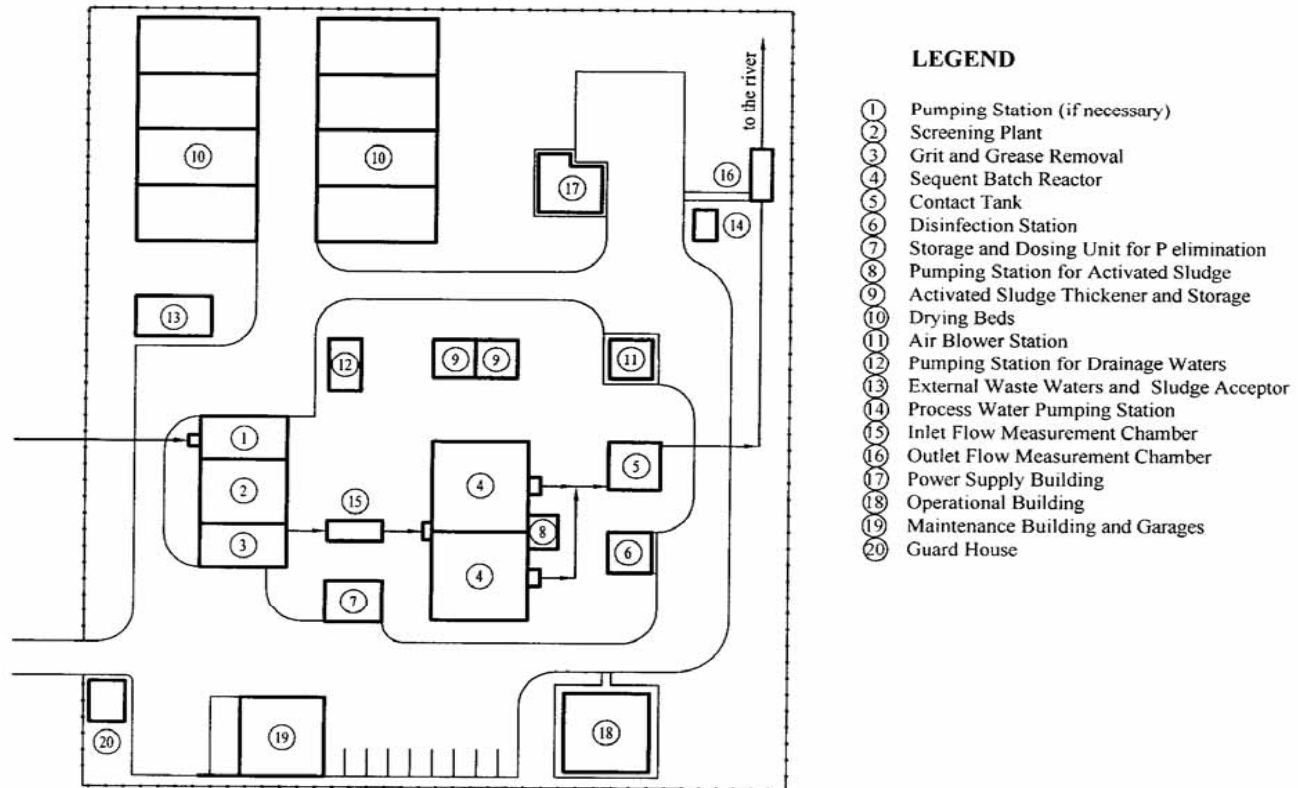
Annex C.2.6 Typical Layout for WWTP with less than 5,000 PE
