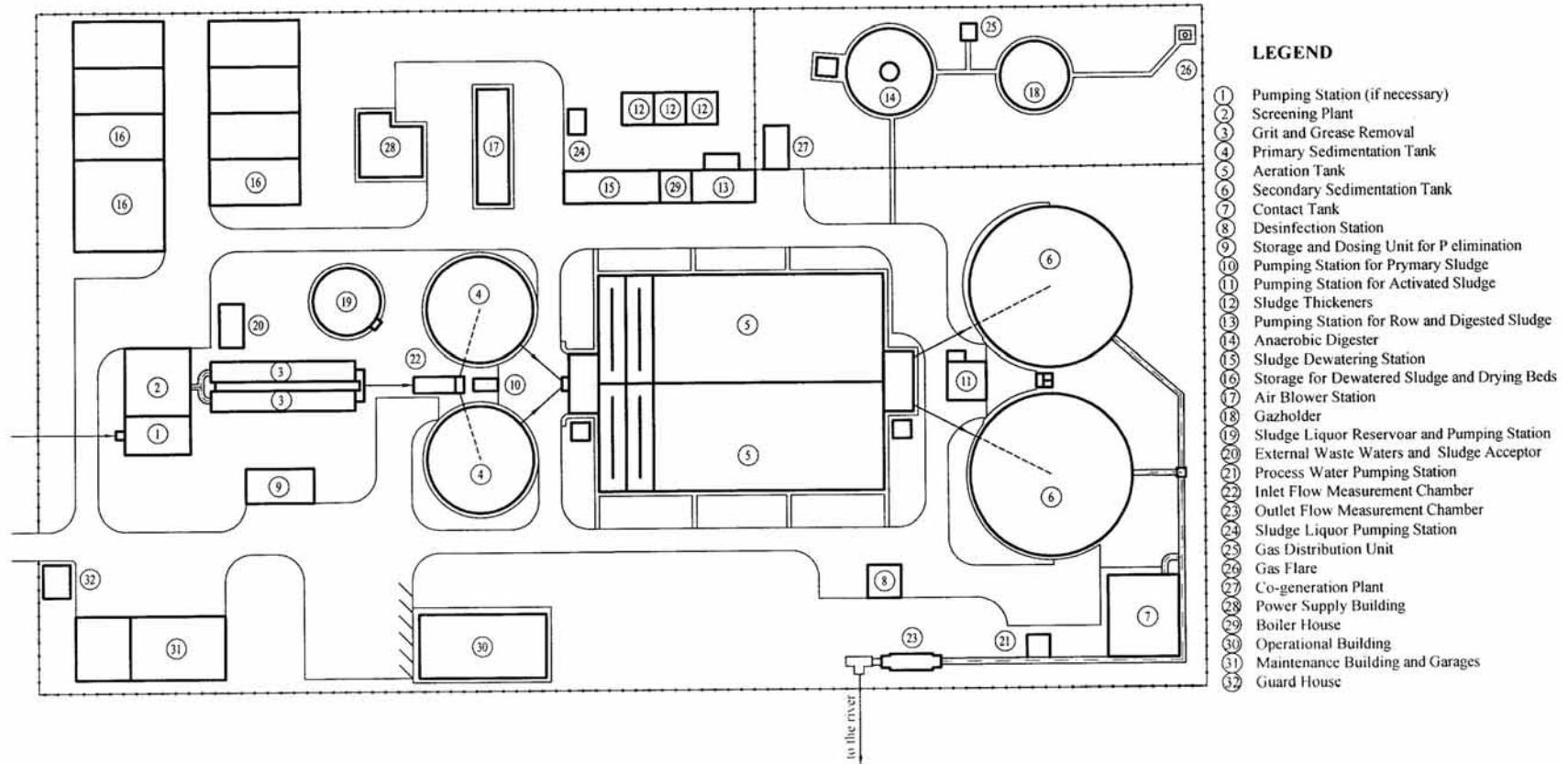
Layout (example for towns with more than 50000 PE)
