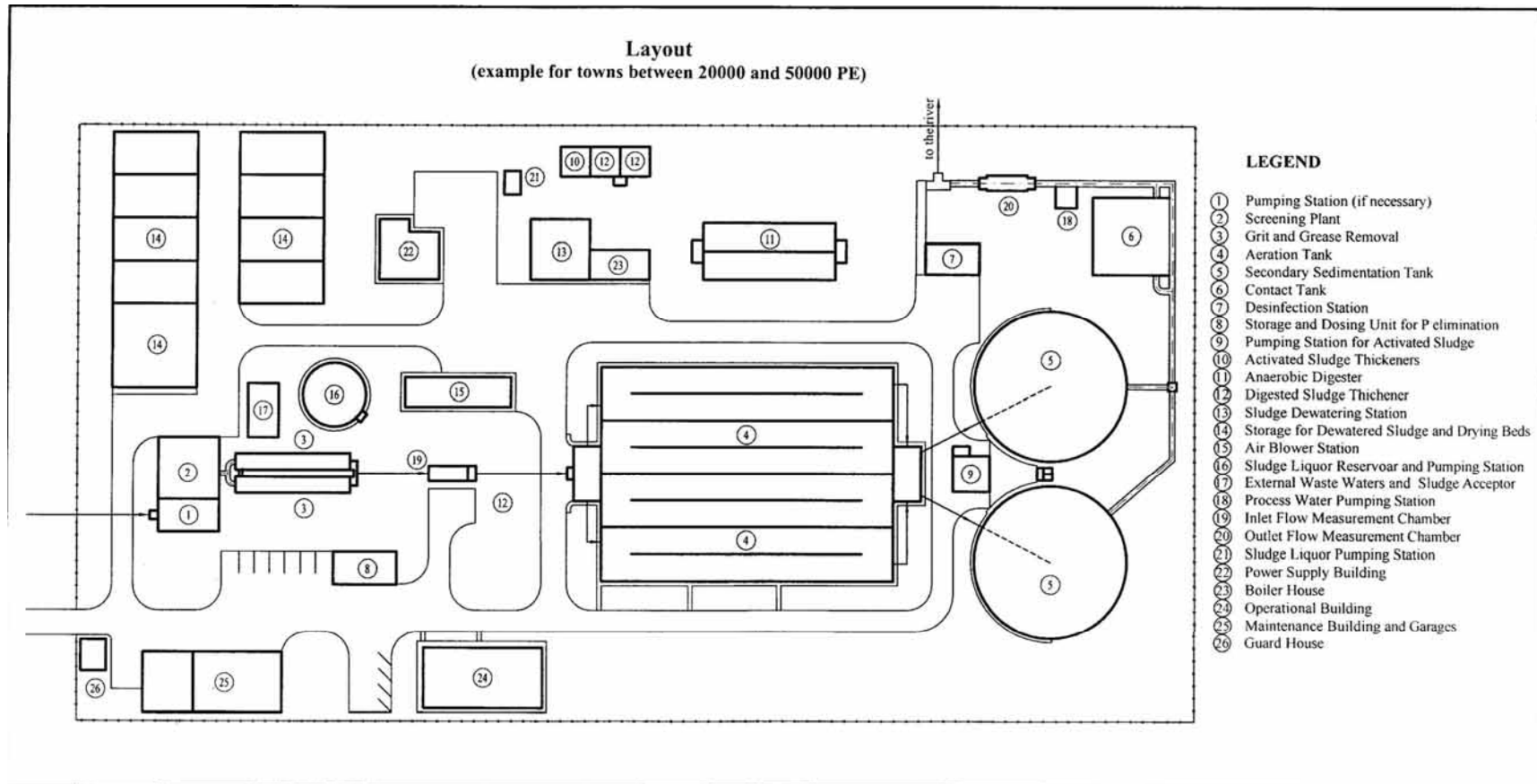
Annex C.2.4 Typical Layout for WWTP with 20,000 to 50,000 PE
