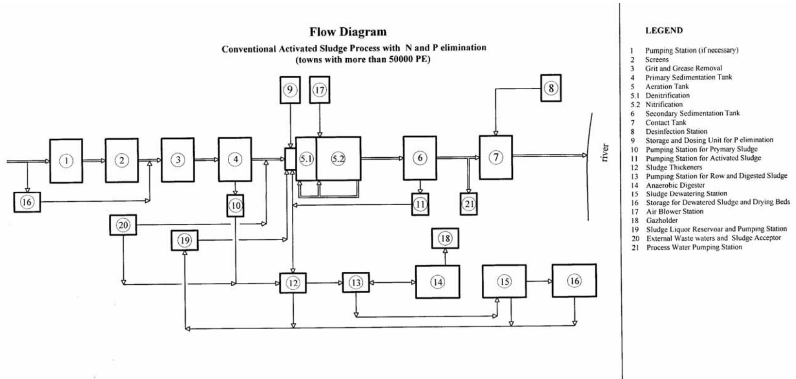
Annex C.2.1 Flow Diagram for WWTP with more than 50,000 PE
