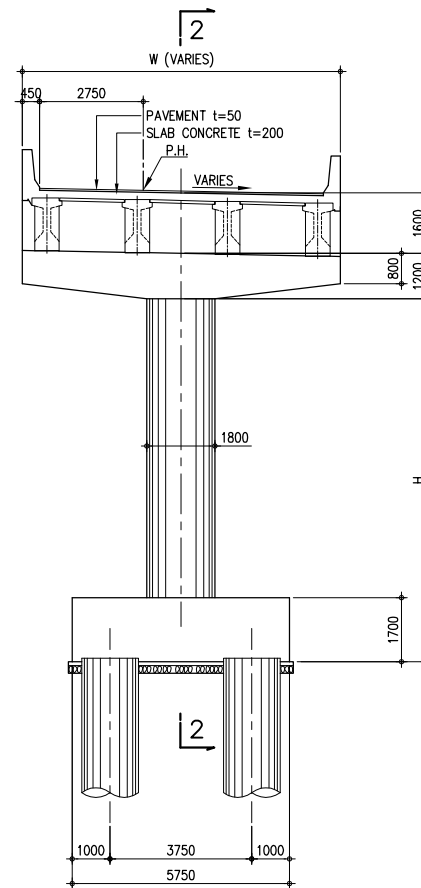
2 TYPICAL CROSS SECTION OF PIER SCALE 1:100
