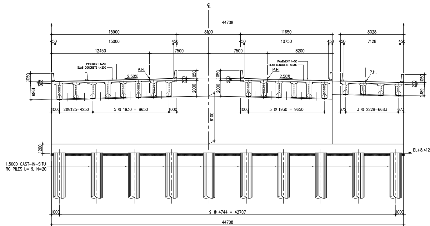
3 CROSS SECTION OF ABUTMENT 2 SCALE 1:150
