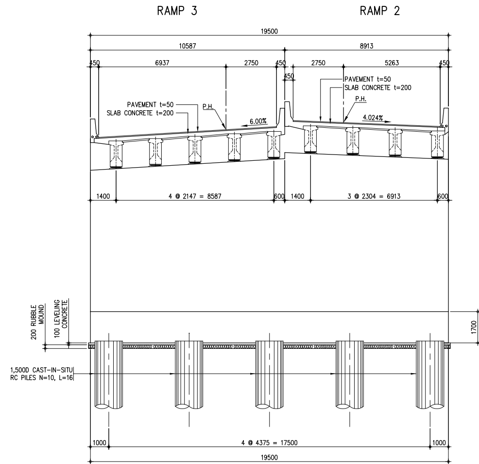
1 CROSS SECTION OF ABUTMENT SCALE 1:100
