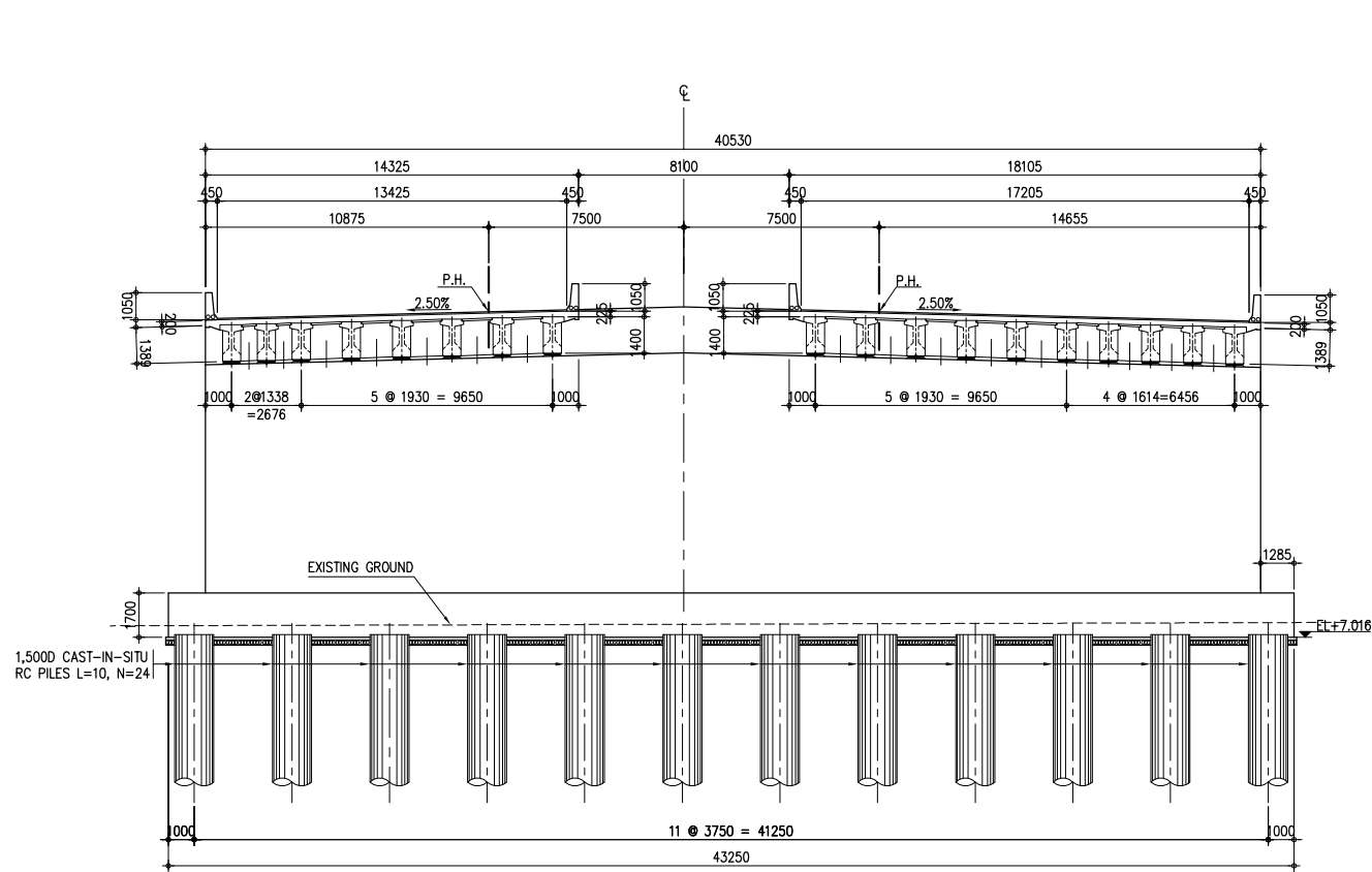
1 TYPICAL CROSS SECTION OF ABUTMENT SCALE 1:150
