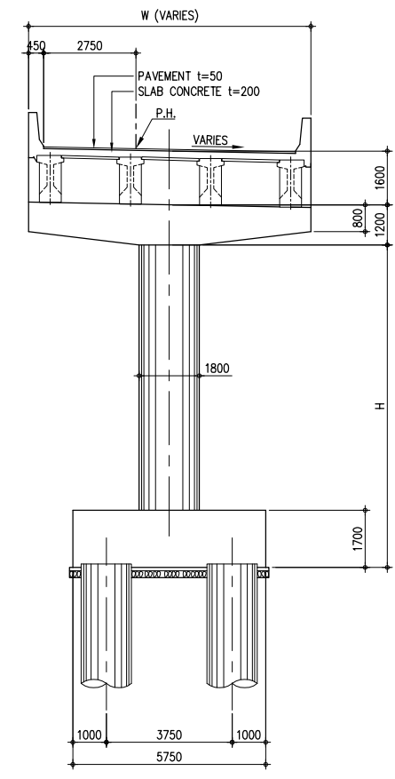
2 TYPICAL CROSS SECTION OF PIER SCALE 1:100
