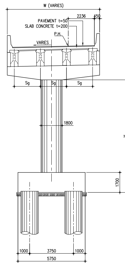
2 TYPICAL CROSS SECTION OF PIER SCALE 1:100
