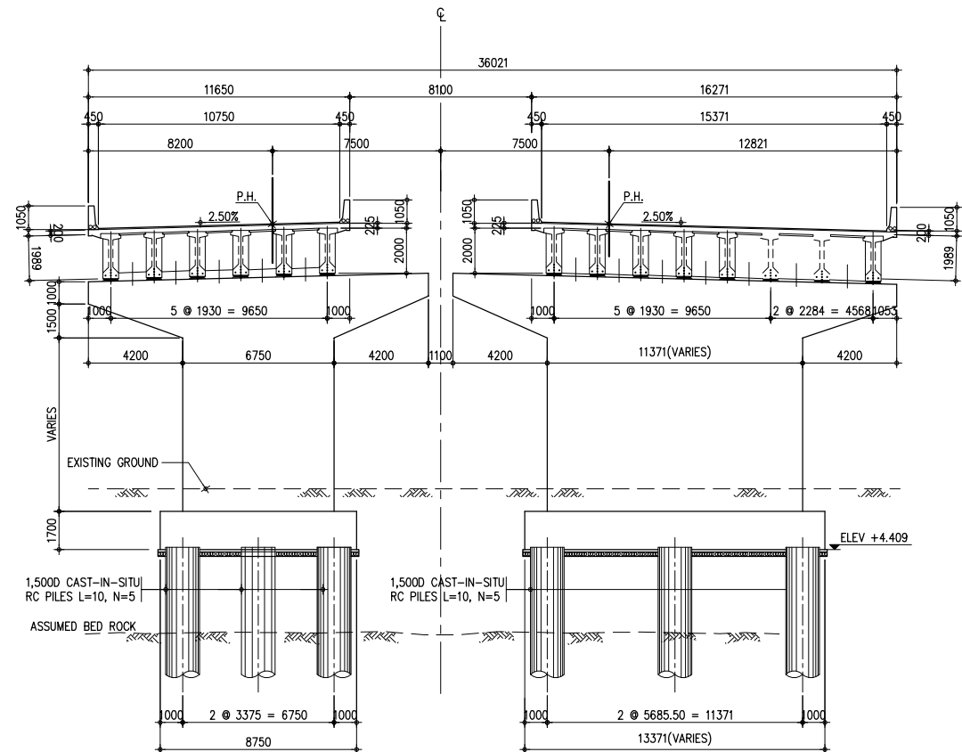
2 TYPICAL CROSS SECTION OF PIER SCALE 1:150
