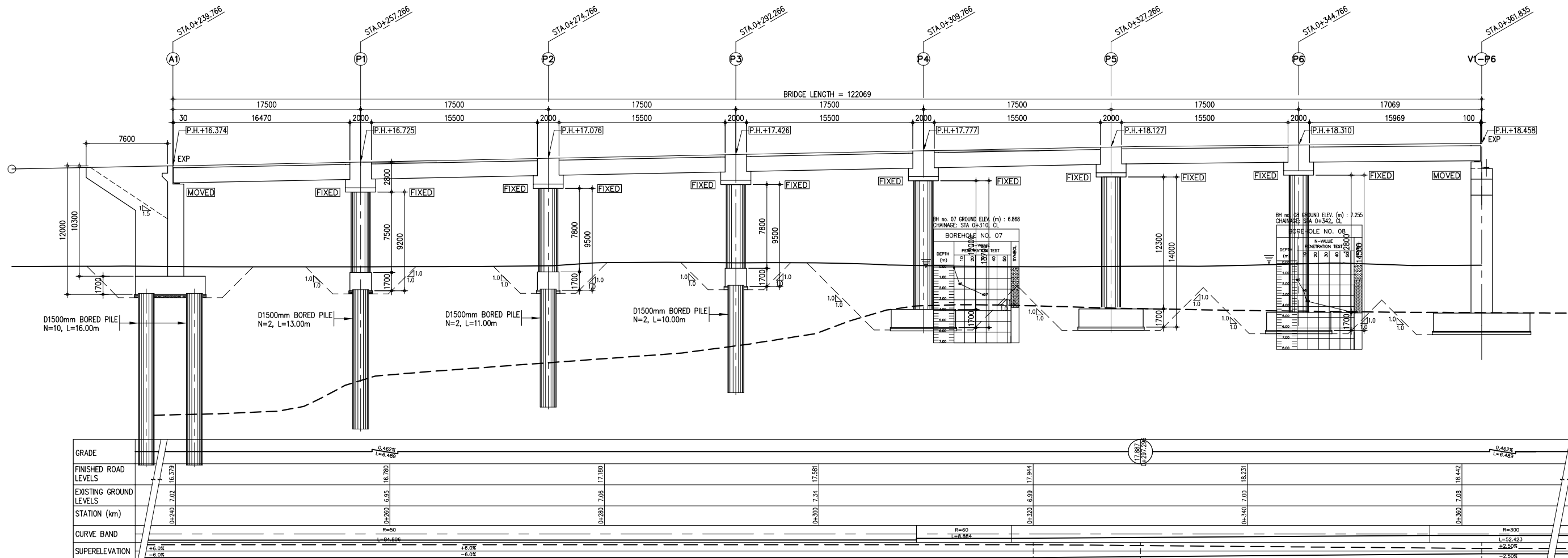
2 PROFILE SCALE 1:200
