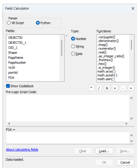
Figure 7-2 Field Calculator and equation to calculate PGA using constant/uniform PGA on the engineering bedrock
