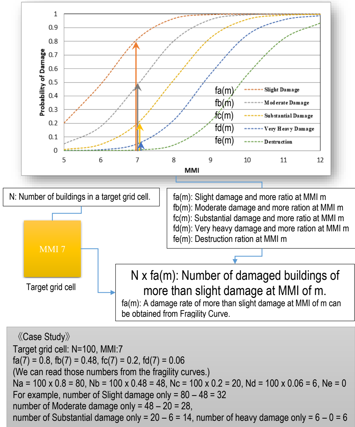
Figure 3-4 Procedure to calculate number of building damage using Fragility Curve (Fragility Curve: NED University)
