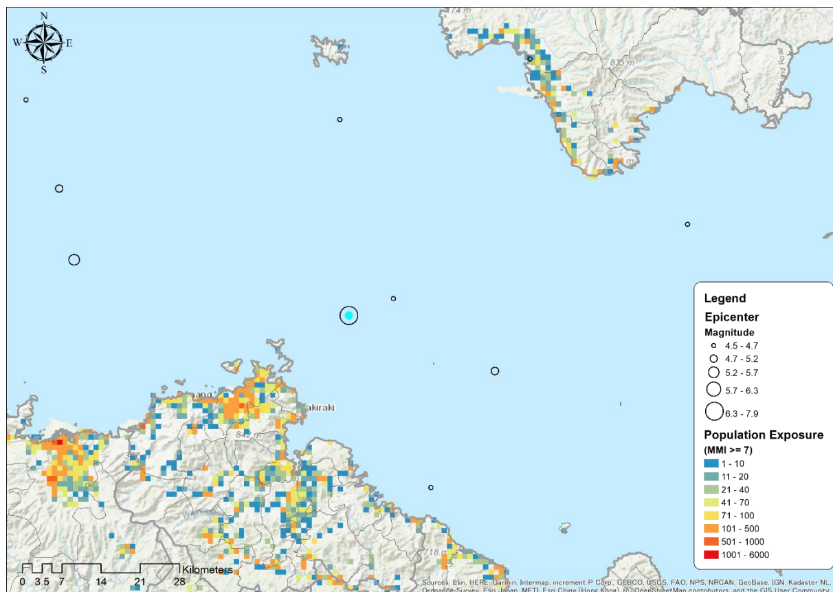
Figure 5-8 Population Exposure (larger than MMI 7) Map due to Rakiraki Scenario (M 6.5)
