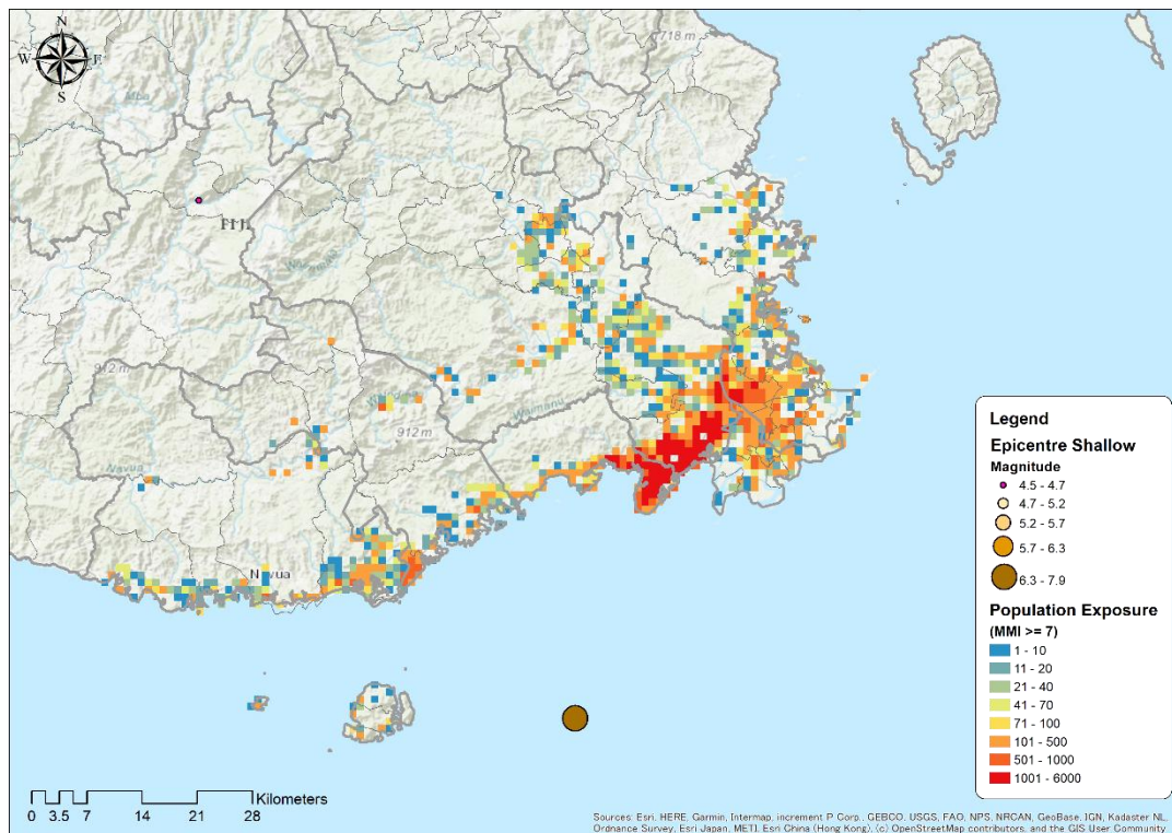
Figure 5-12 Population Exposure (larger thann MMI 7) Map due to Suva Scenario (M 6.4)
