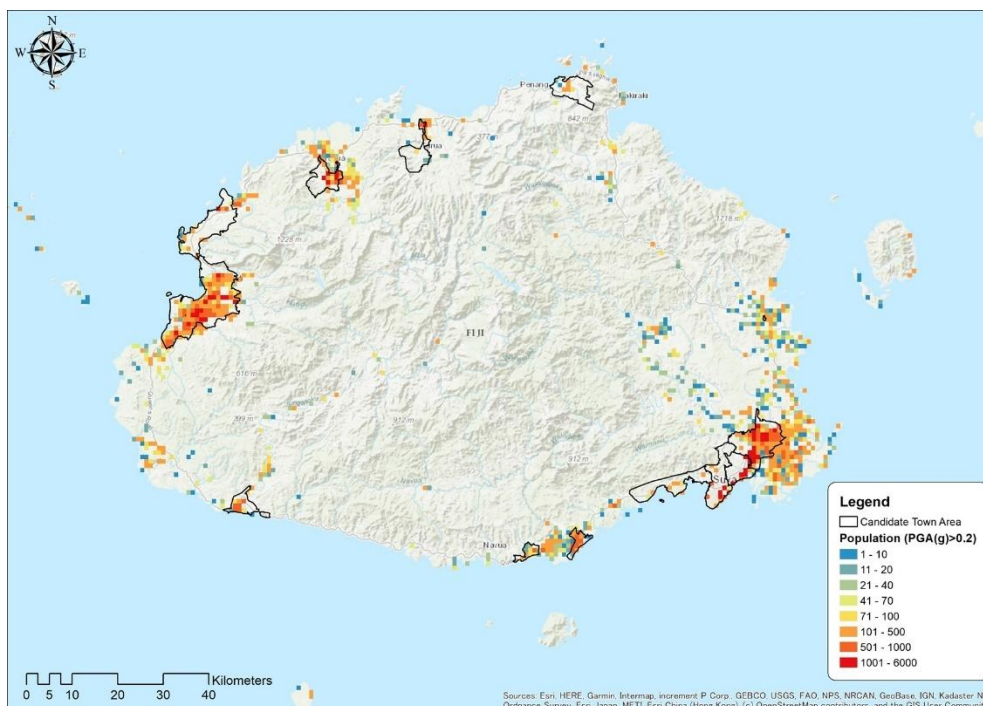
Figure 7-3 Population Exposure ( PGA > 0.2(g) ) and candidate Town Area
