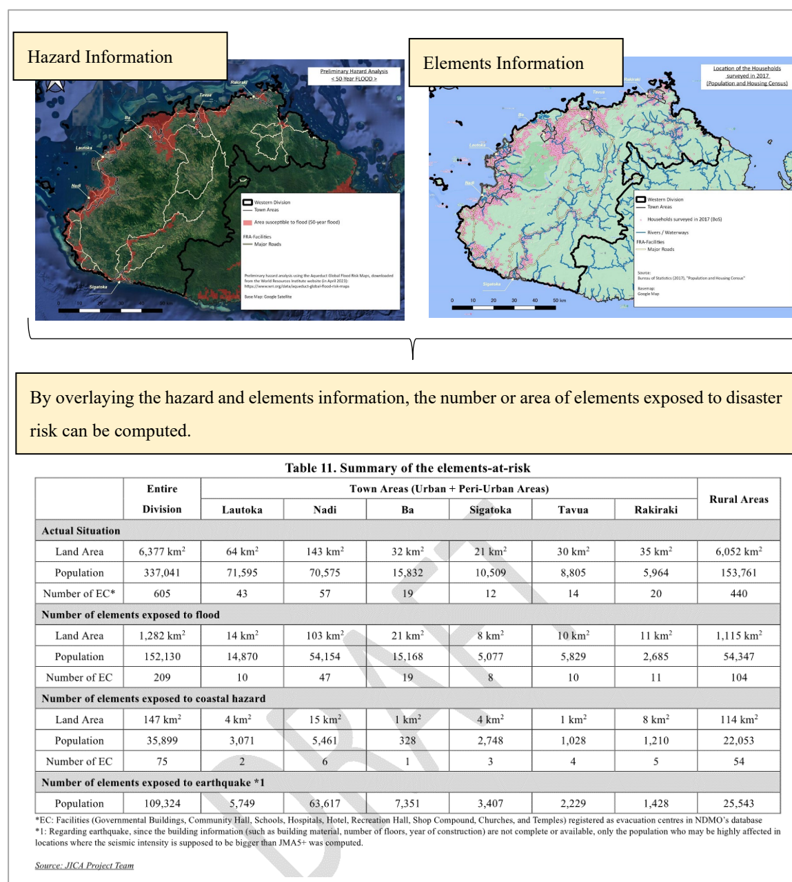
Figure 11. Image of the estimation of elements-at-risk
