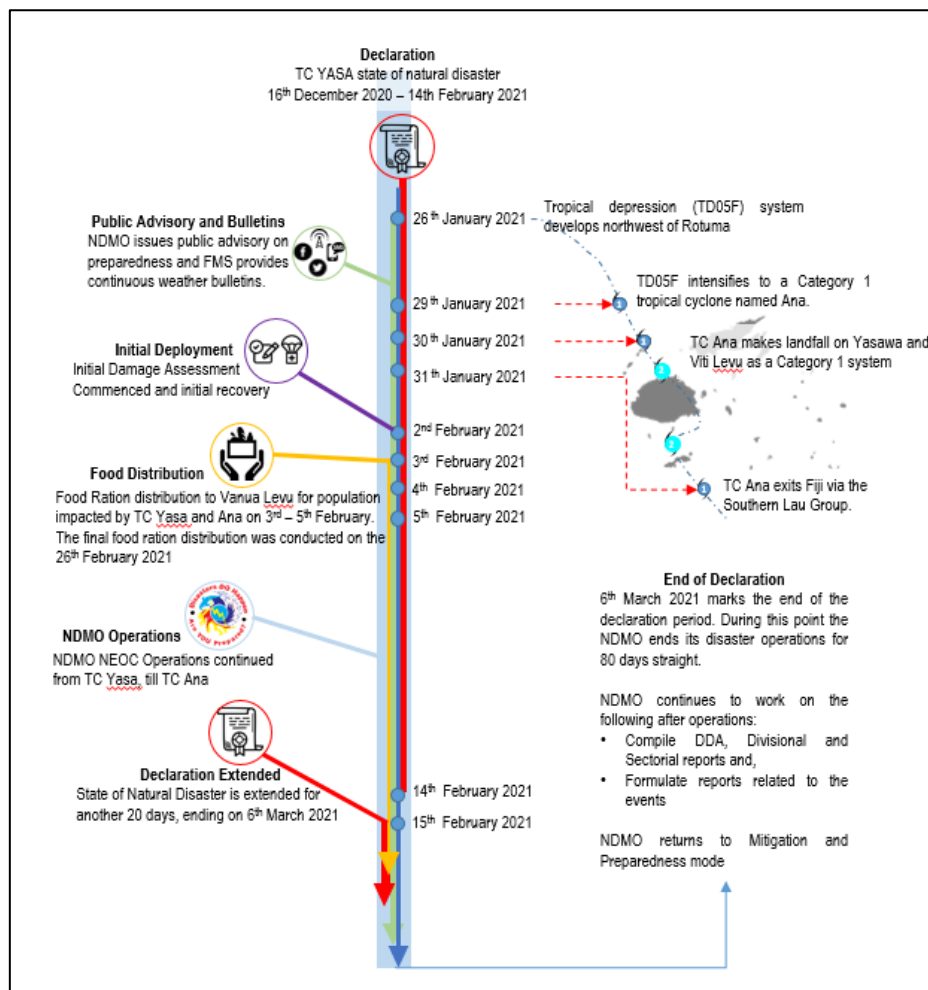
Fig. 10 TC Ana Sequence of Events and Cyclone Track Map.
