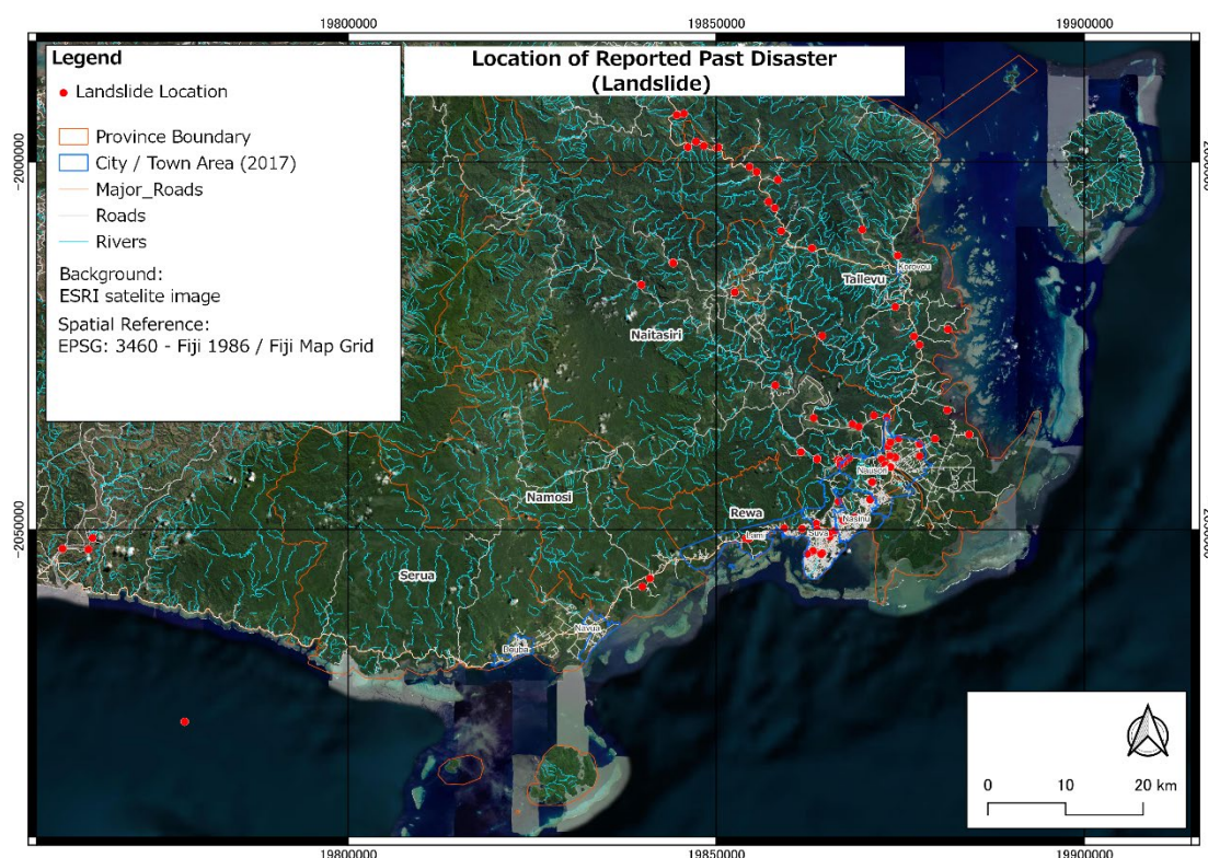
Figure XX. Location of Landslide for the recent years (2022-2024)
