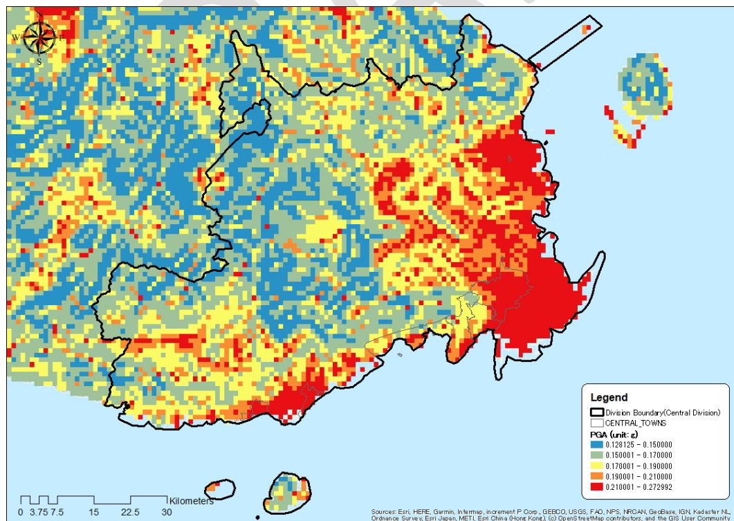
Figure 20. Ground Motion Map
