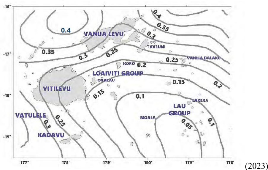
Figure 6-1 Comparison of Zone Factor Map between 1990 and 2023
