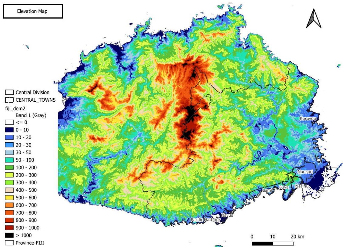
Figure 11. Elevation Map
