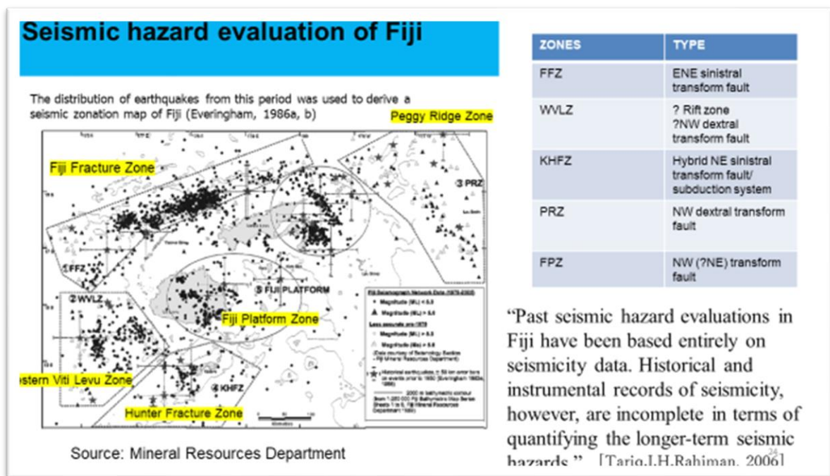
Figure 2-4 Seismic Zones in and around Fiji Islands (source: MRD)
