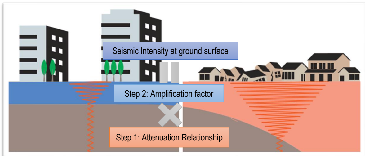
Figure 2-9 Image of calculation of seismic ground motion at surface of the earth [ including Cases of low hazard site and high hazard ] (editing Your Community's Earthquake Risk of Tokyo Metropolitan Government, 2022)
