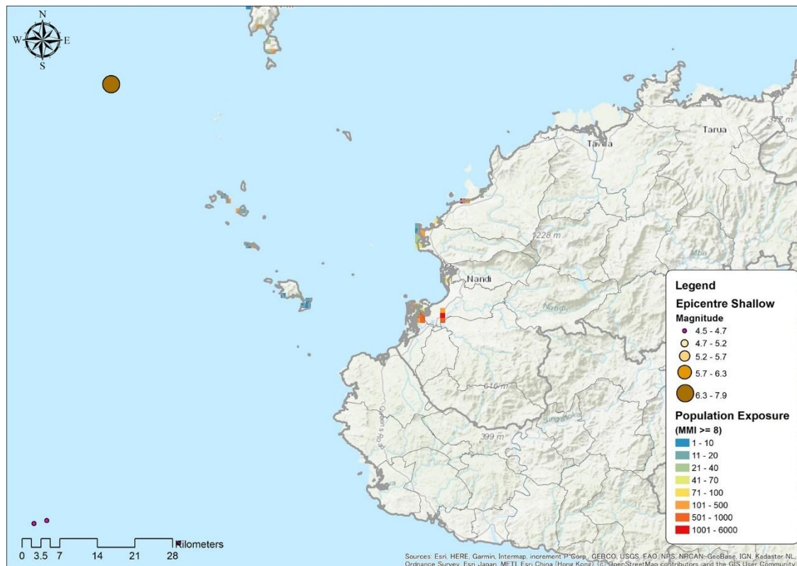
Figure 5-4 Distribution of Population exposed to MMI seismic intensity level 8 and above
