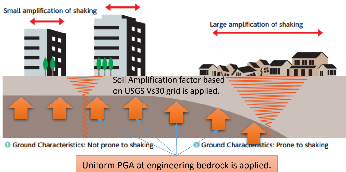
Figure 7-1 Basic Idea of setting Uniform PGA based on Tokyo Metropolitan Government ( https://www.funenka.metro.tokyo.lg.jp/2024/02/kikendo_english.pdf ) ( https://www.funenka.metro.tokyo.lg.jp/assets/pdf/archive/kikendo_all.pdf )
