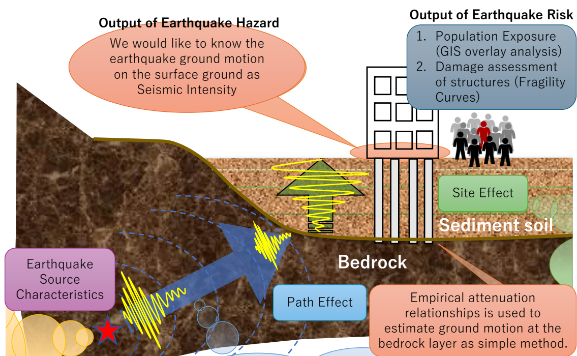
Figure 1-1 Schematic diagram of outbreak mechanism of earthquake
