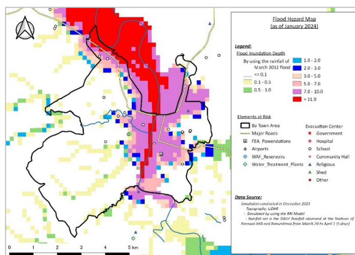
Figure 7. Flood Hazard Map prepared based on simulation results
