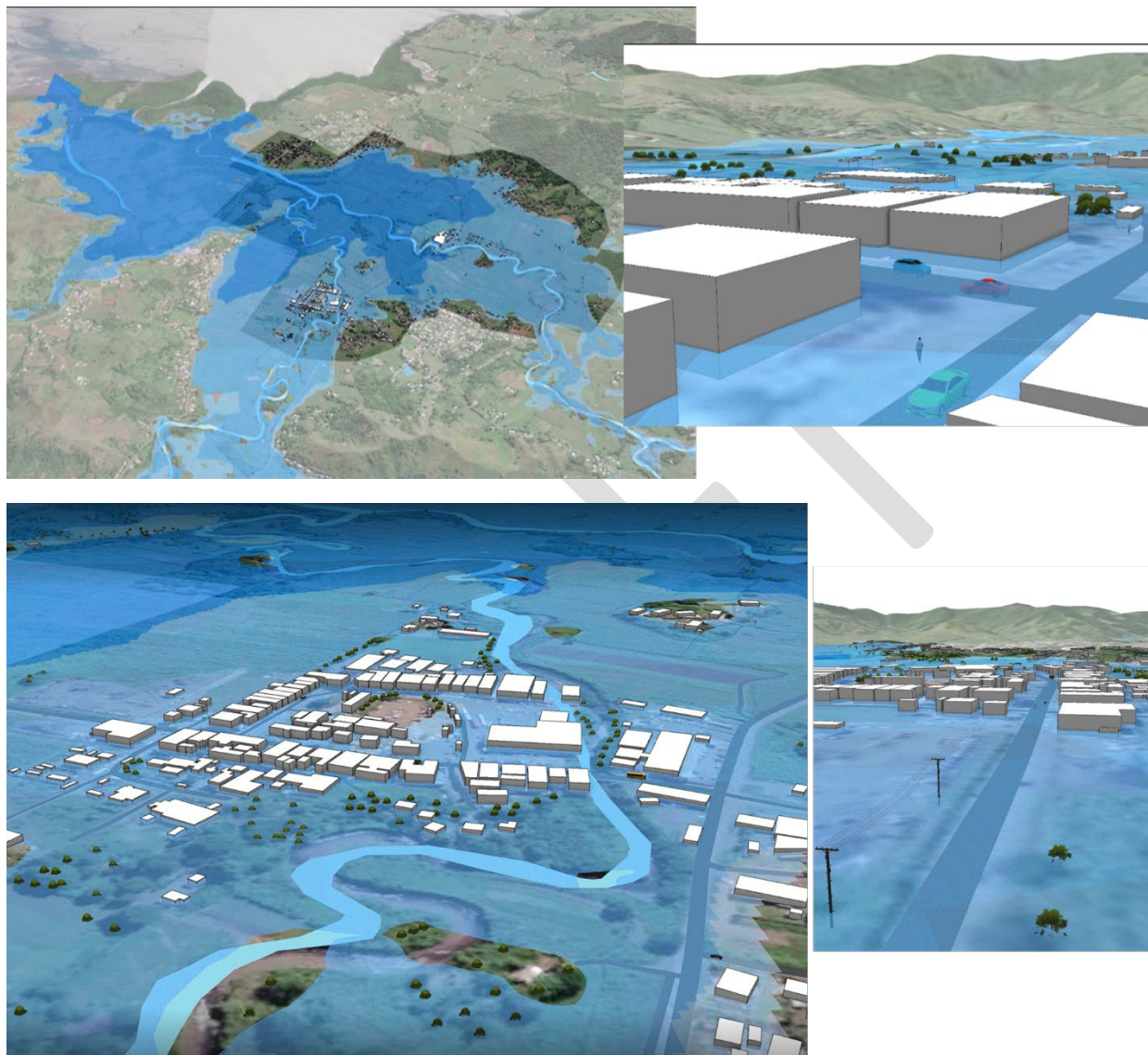
Figure 3-8 3D Model to Enhance the Understanding of Flood Risk in Rakiraki Town
