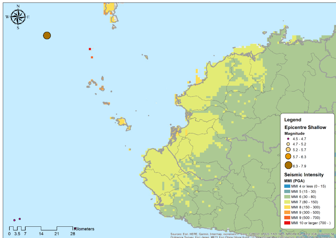
Figure 5-2 MMI seismic intensity Map in and around Nadi
