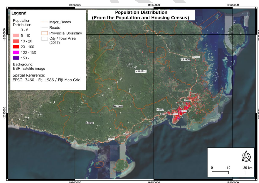
Figure 21. Population Distribution from the Census 2017
