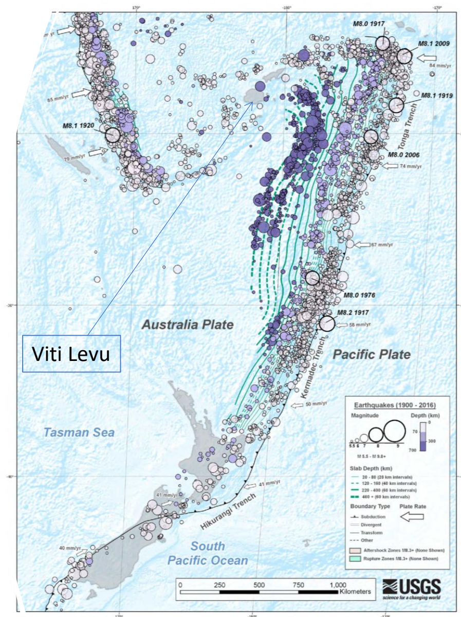
Figure 2-3 Seismic Activity (M 5.5 – 9.0) in a wide area during 1900 – 2016 (source: USGS)
