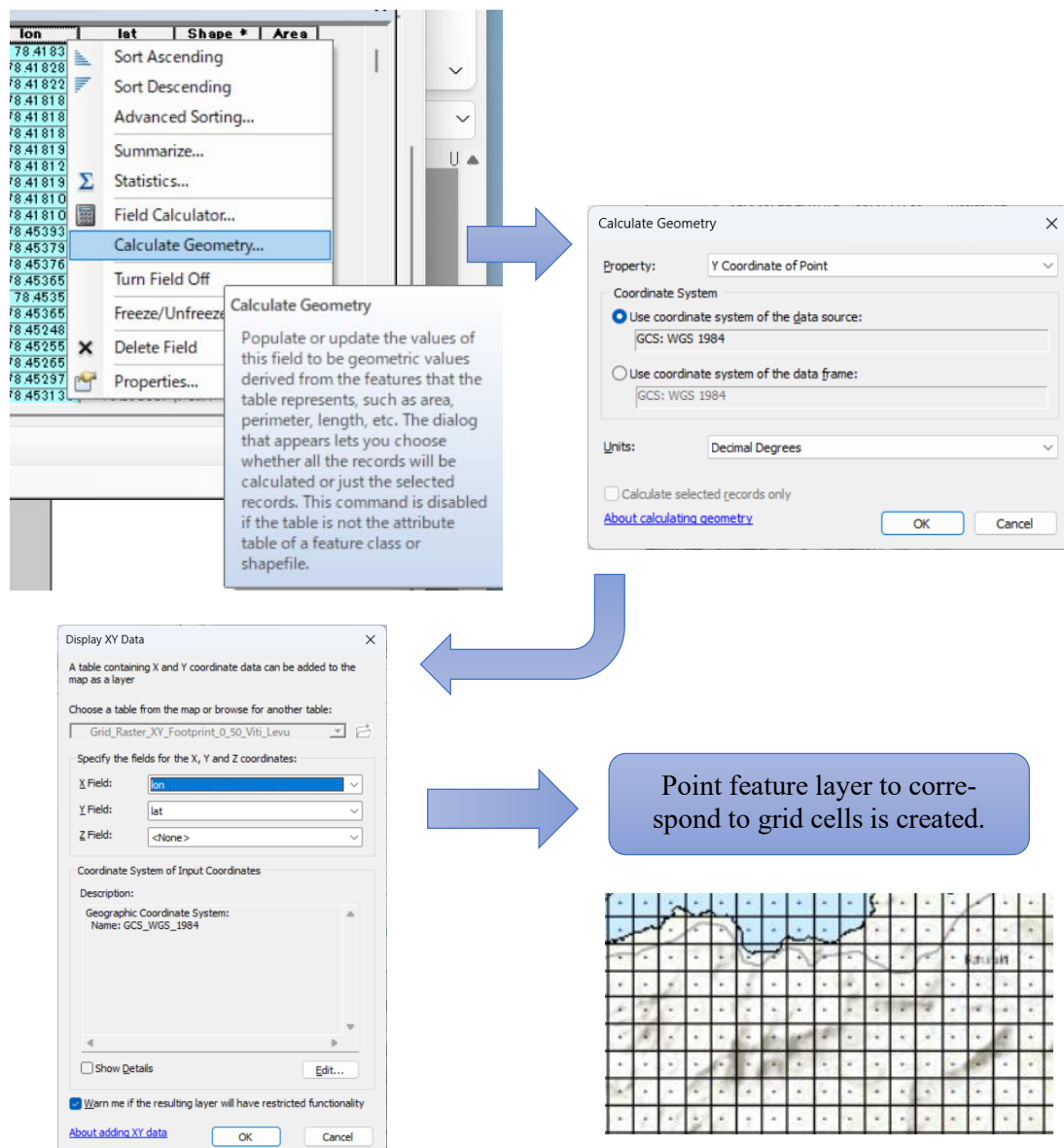
Figure 4-2 Procedure to create grid point feature to store Vs30
