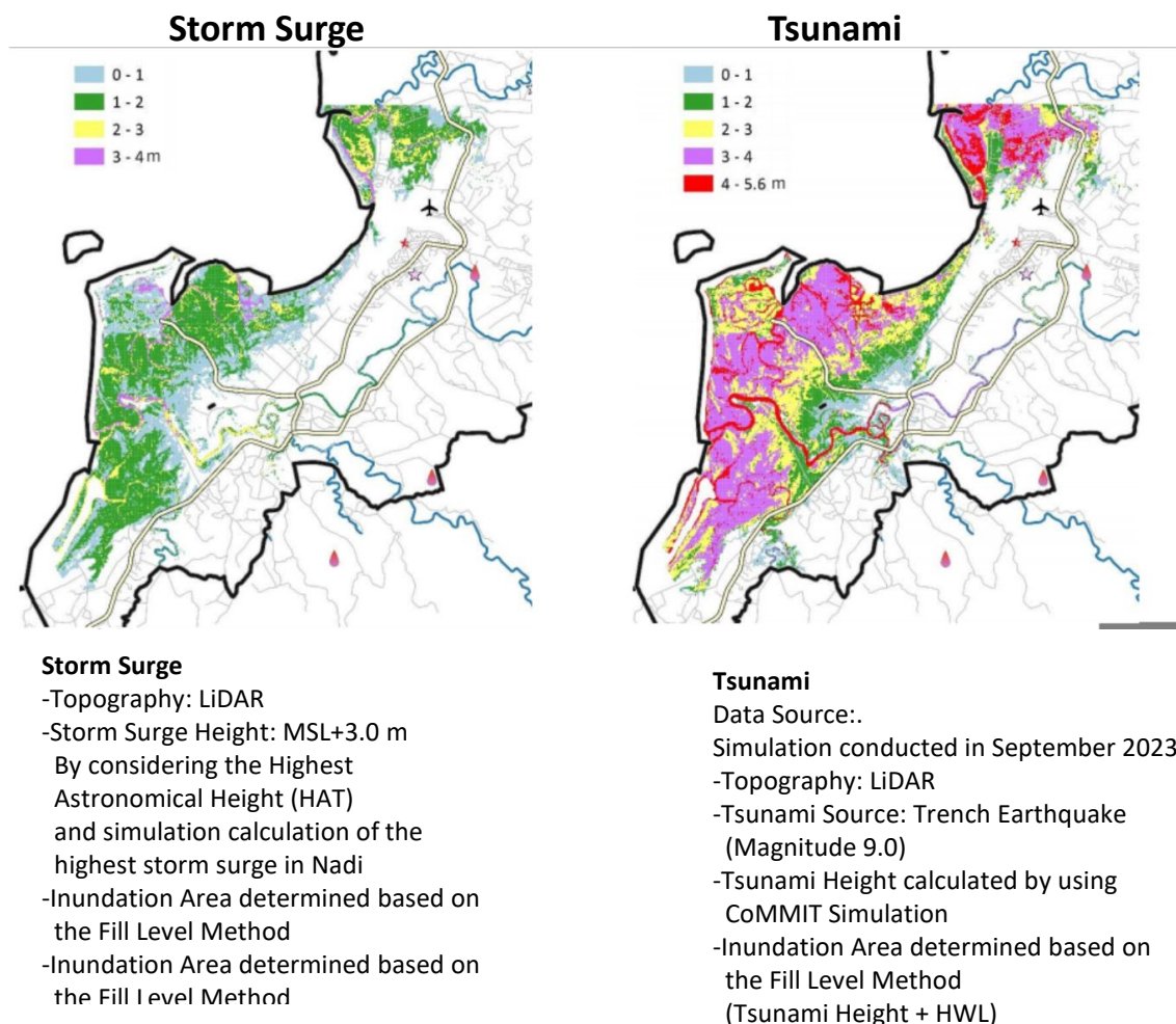
Figure 7: Hazard Risk Simulation Example
