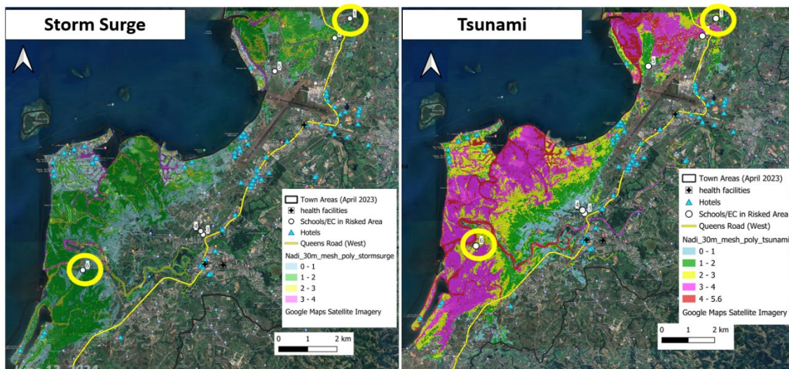
Figure 16: Example of extraction of important public facilities that need to be addressed (superimposed diagram) (Nadi)
