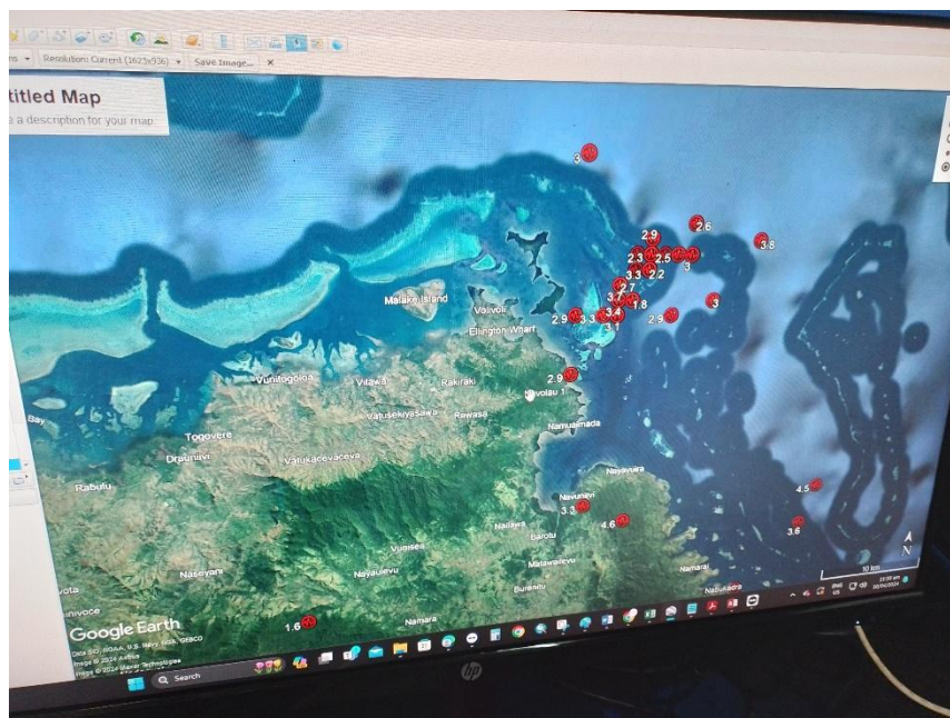
Figure 5-7 Monitoring seismic activity around Rakiraki in March and April 2024 (provided by MRD Seismology Section)
