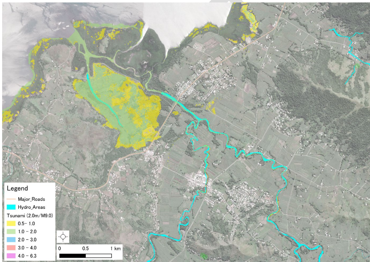
Figure 3-4 Coastal Disaster in Rakiraki (Tsunami, M9.0 Scenario)
