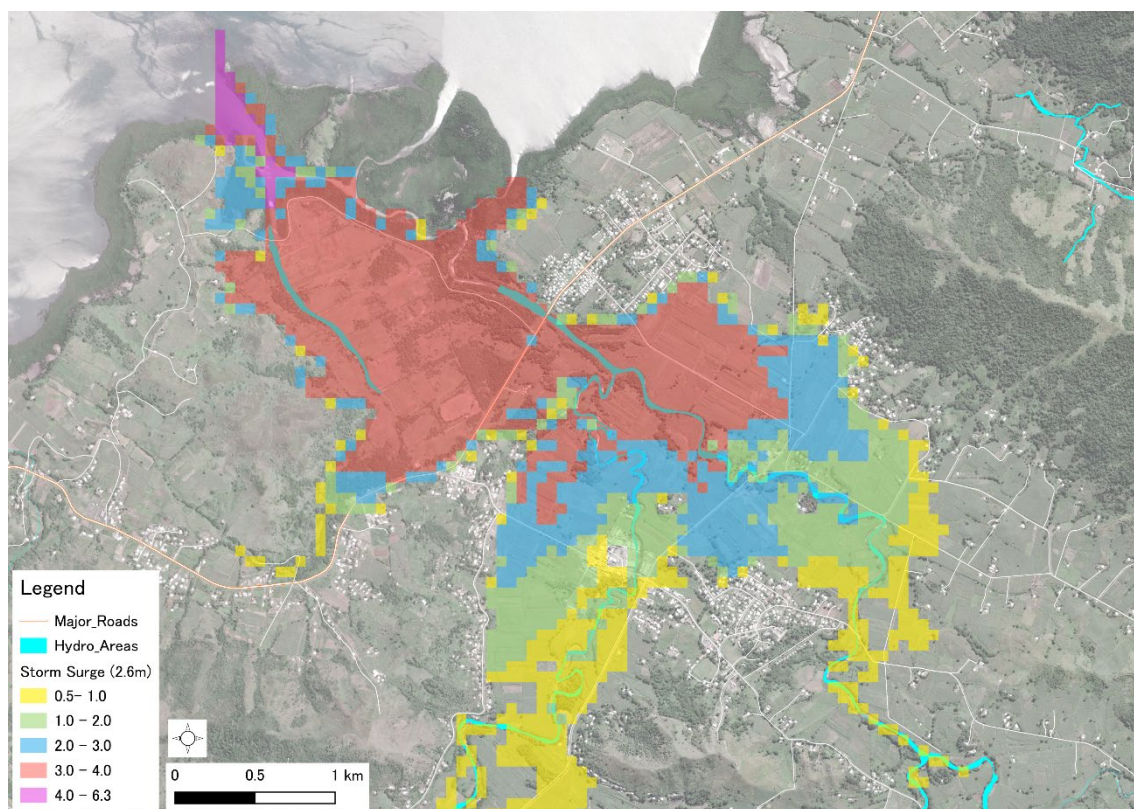
Figure 3-6 Flood Hazard on Rakiraki
