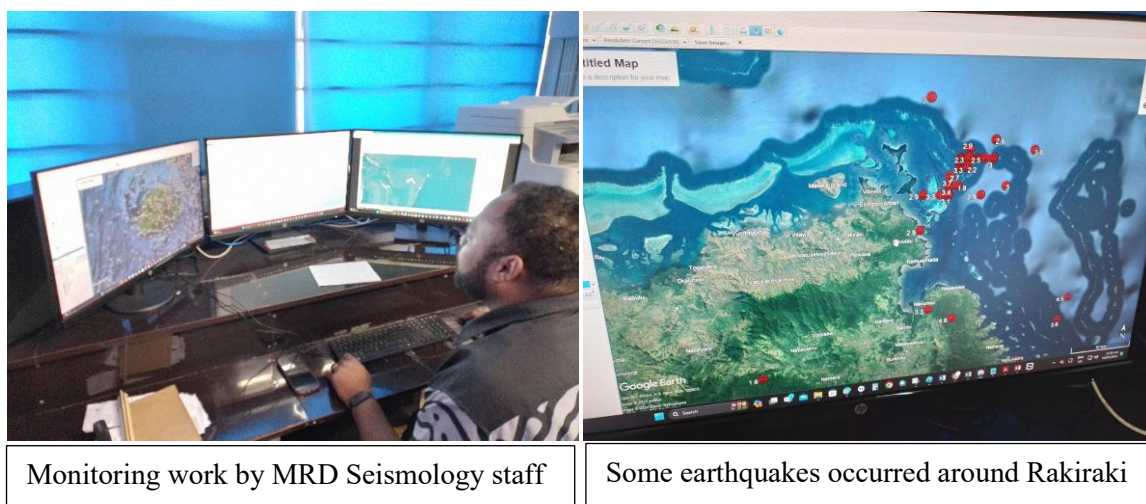
Figure 2-5 Monitoring latest seismic activity in local level by MRD Seismology Section
