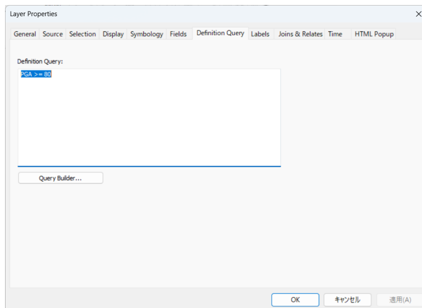
Figure 4-6 Procedure to present Population Exposure to Seismic Intensity by Definition Query in Arc GIS Desktop
