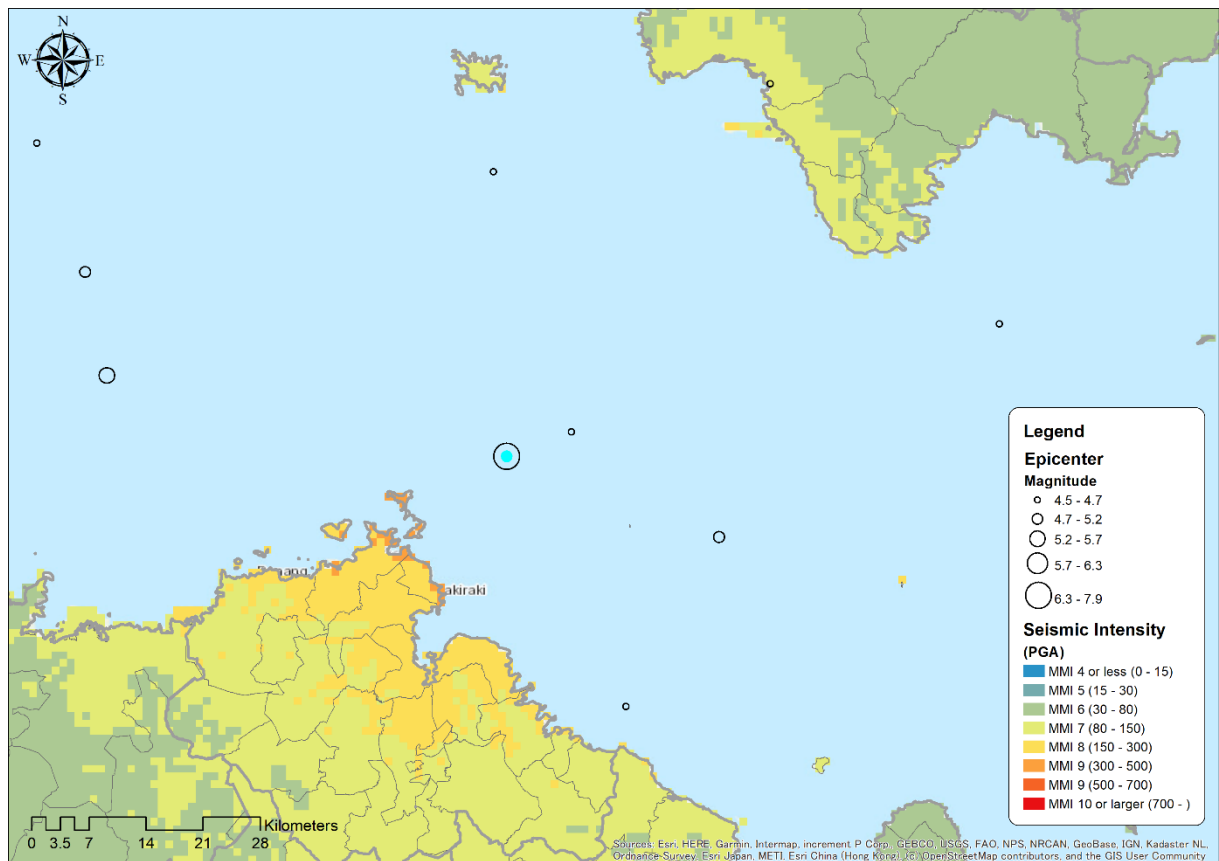
Figure 5-6 Calculation Result of Earthquake Hazard Map due to Rakiraki Scenario (M 6.5)
