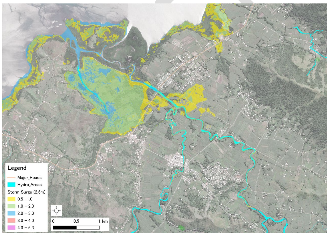
Figure 3-3 Coastal Disaster in Rakiraki (Storm Surge)
