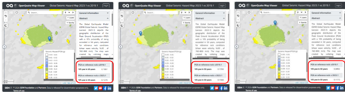
Probabilistic Seismic Hazard at Suva, Nadi and Rakiraki (Comparison of PGA between 2019 and 2023 version, see red line rectangle)
