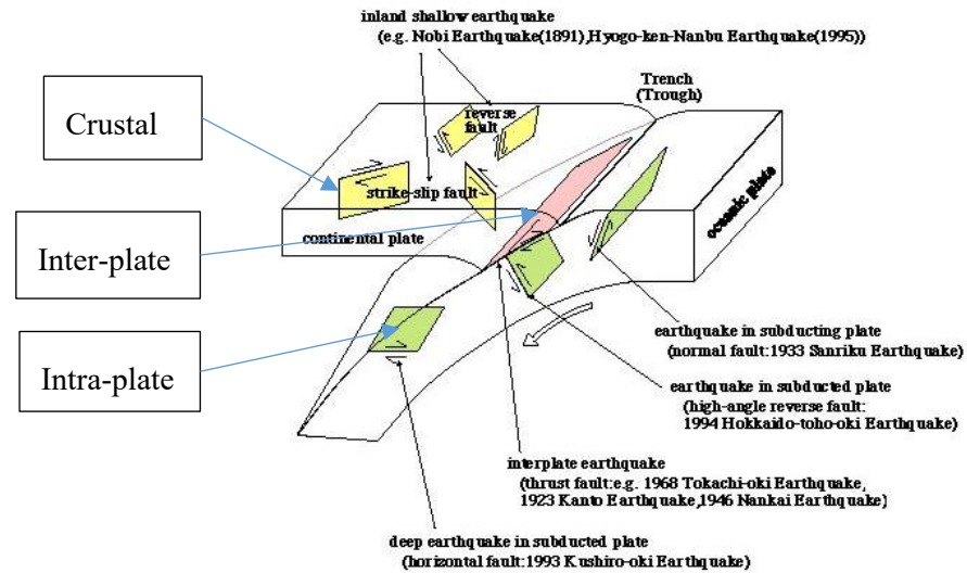
Figure 1-4 Fault type in the attenuation equation of Si and Midorikawa (1999)
