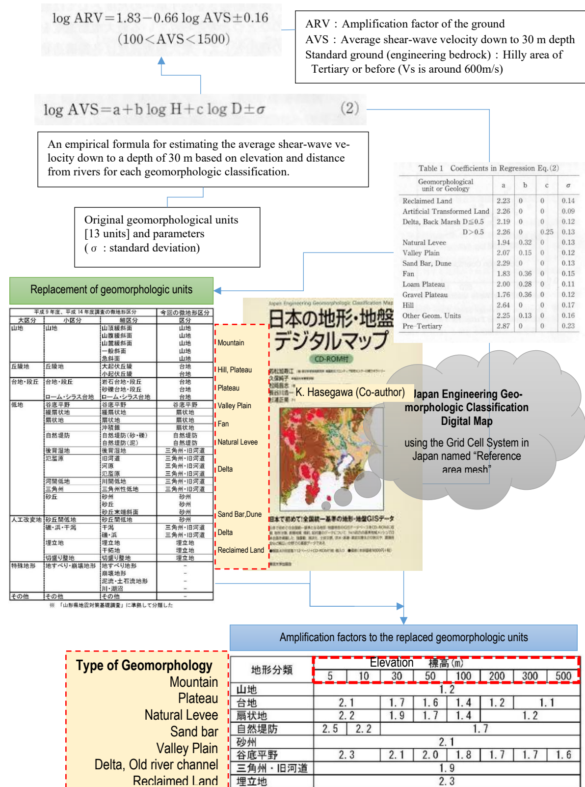
Figure 1-5 Flow for estimation of amplification factor based on geomorphologic classifications. (Japan Engineering Geomorphologic Classification Map 8 )
