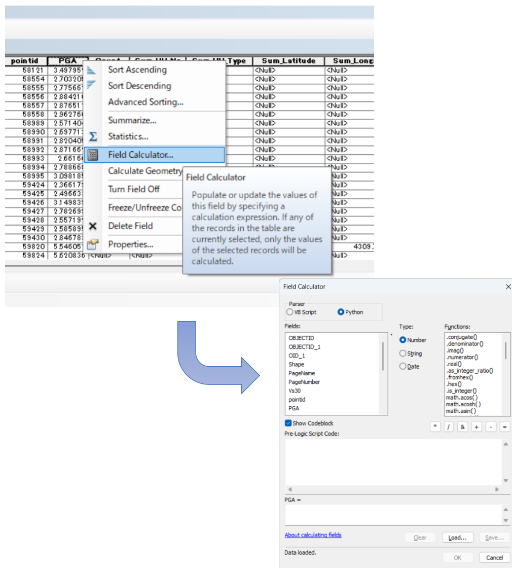
Figure 4-5 Procedure to Execute Field Calculator for Attenuation Relationship and Amplification Factor method
