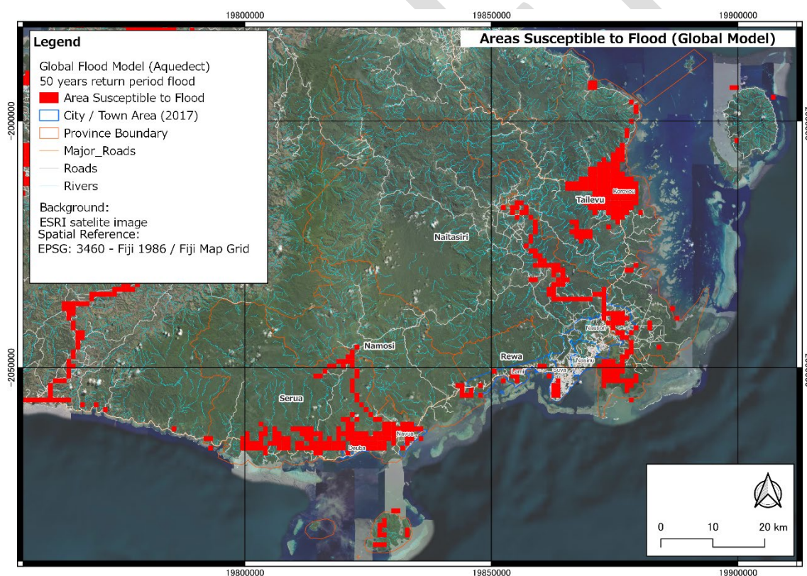
Figure 17. Areas susceptible to flood (50-year)
