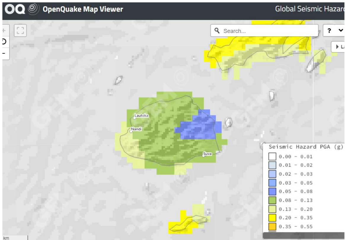
Figure 2-7 Probabilistic Seismic Hazard in and around Viti Levu Island [50-year 10% exceedance probability, PGA on an engineering bedrock layer] (source: Global Earthquake Model 9 )
