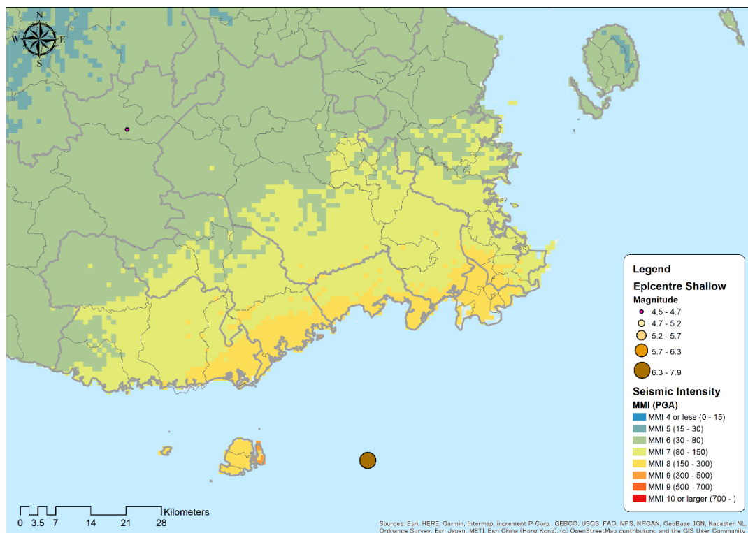
Figure 5-11 Calculation Result of Earthquake Hazard Map due to Suva Scenario (M 6.4)
