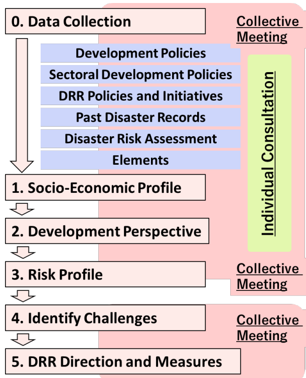
Figure 1 Flow of Data Collection
