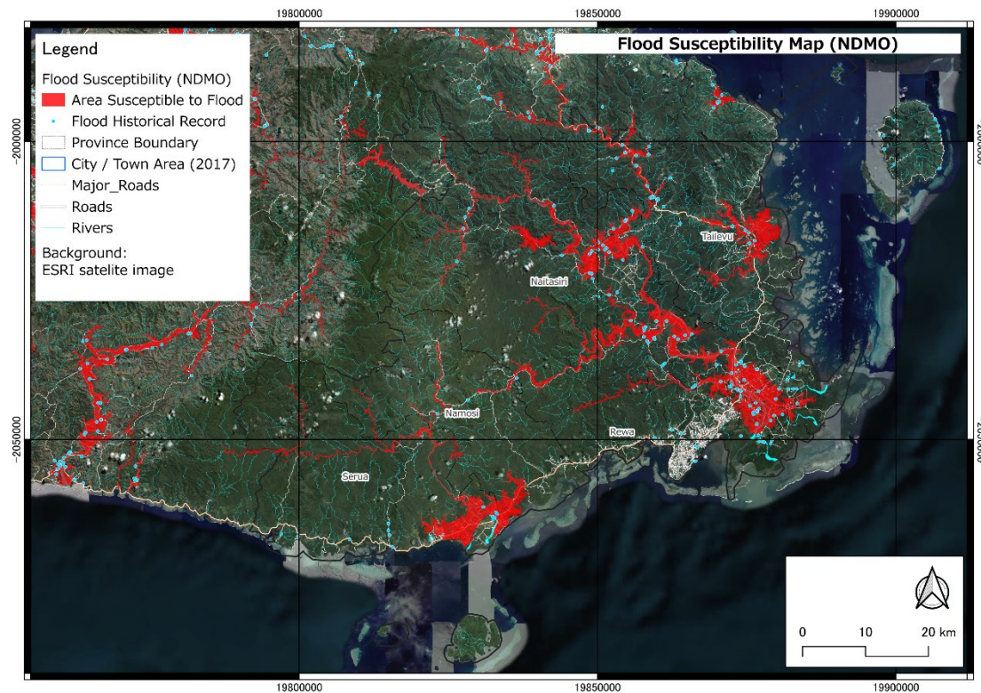
Figure 18. Flood Susceptibility Map
