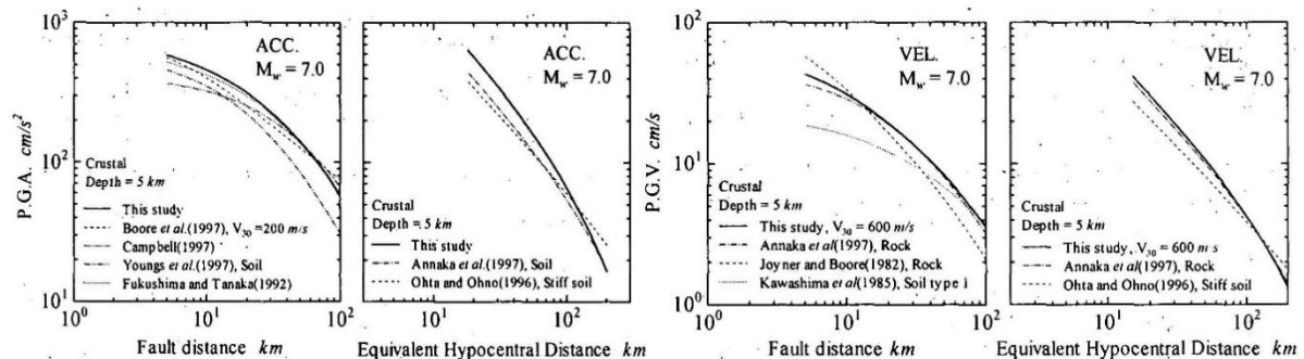
Figure 1-3 Relation of attenuation equation [Si and Midorikawa (1999)] with PGA (left) and PGV (right)
