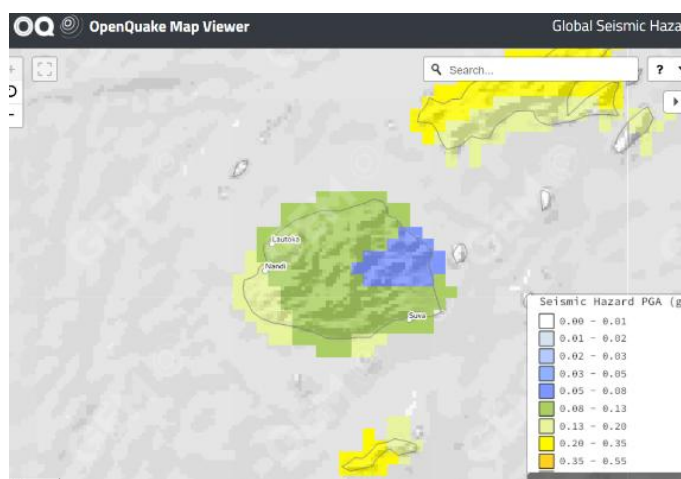
Figure 6-2 Probabilistic PGA Map in GEM
