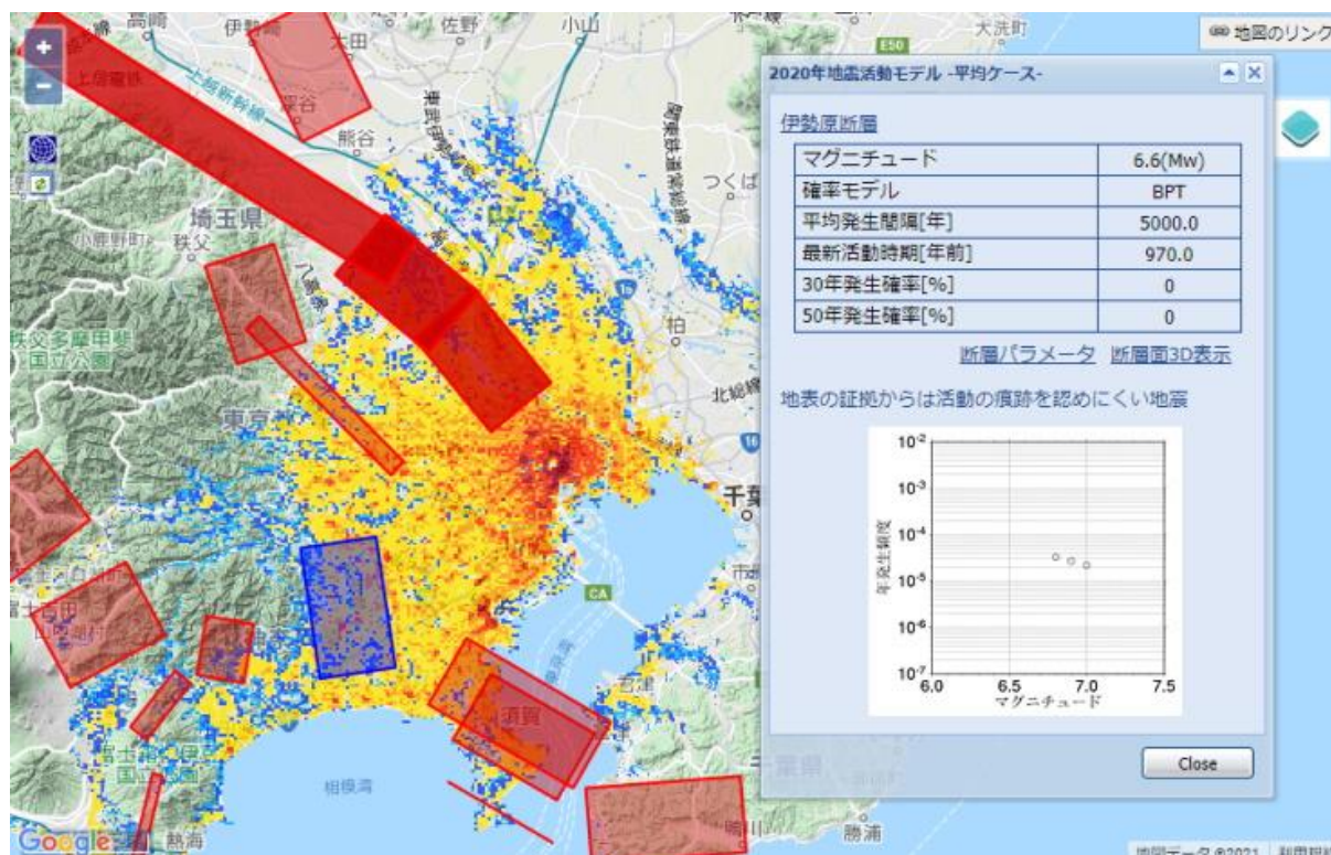
Figure 3-1 Example of Distribution of Population Exposure to Seismic Intensity 10
