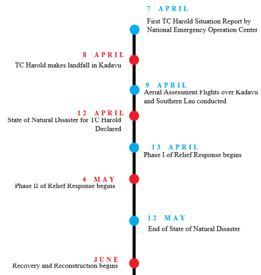
Fig. 2 TC Harold Timeline with respect to preparedness and Response
