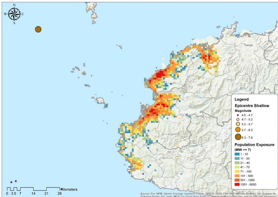
Figure 5-3 Distribution of Population exposed to MMI seismic intensity level 7 and above
