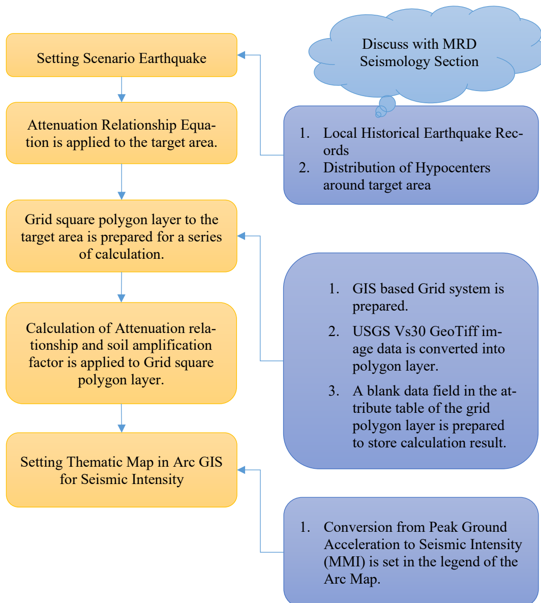
Figure 2-1 Flow of earthquake hazard assessment
