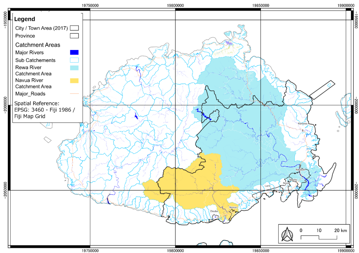
Figure 13. River System
