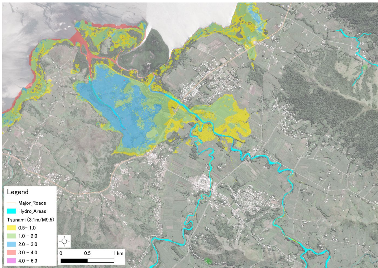
Figure 3-5 Coastal Disaster in Rakiraki (Tsunami, M9.5 Scenario)
