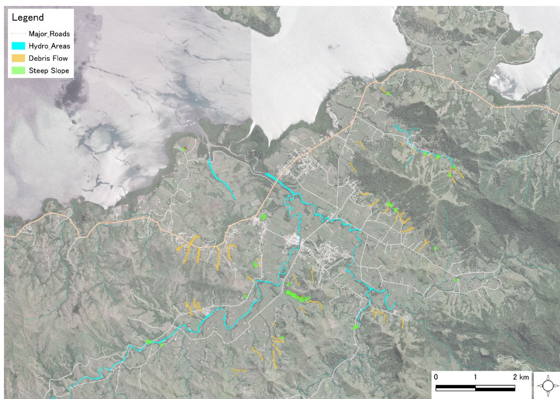
Figure 3-7 Steep slope and Debris Flow on Rakiraki
