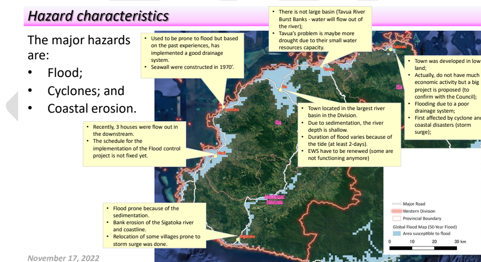
Figure 6. Global Flood Map
