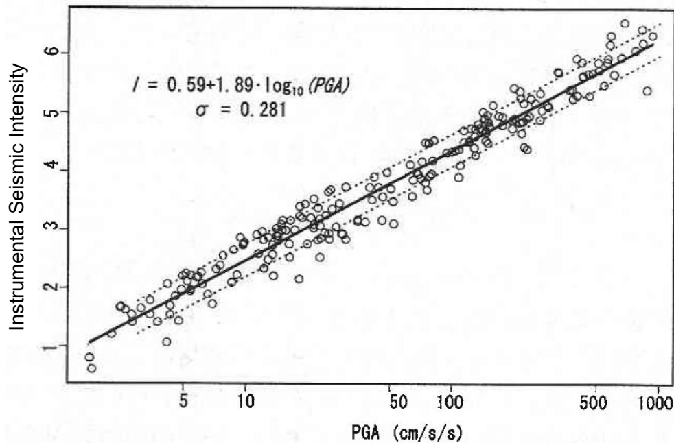
Figure 7-5 Comparison method between PGA and JMA Seismic Intensity (Ton and Yamazaki (1996))
