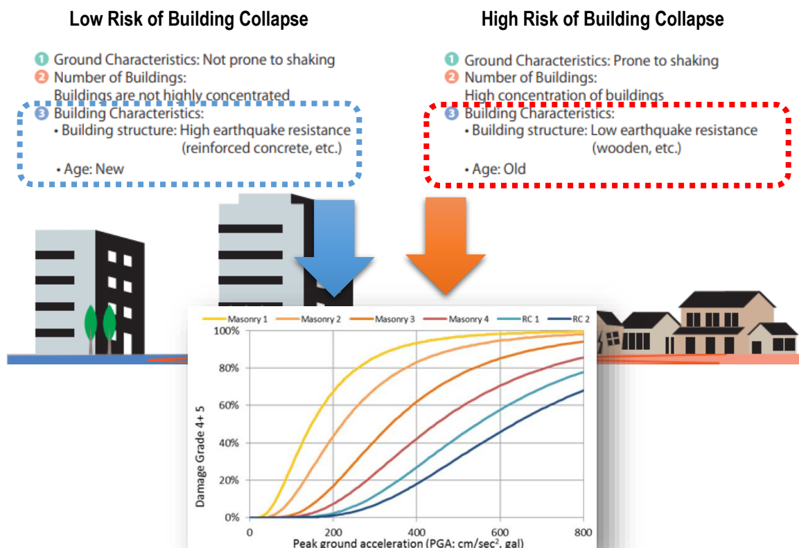
Figure 3-2 Overview of Seismic Risk process (editing Your Community's Earthquake Risk of Tokyo Metropolitan Government, 2022)
