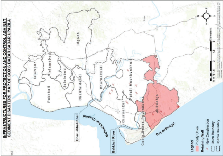
Figure 5-3. Priority Union for Countermeasure to Reduce Risk by Sediment Disaster
