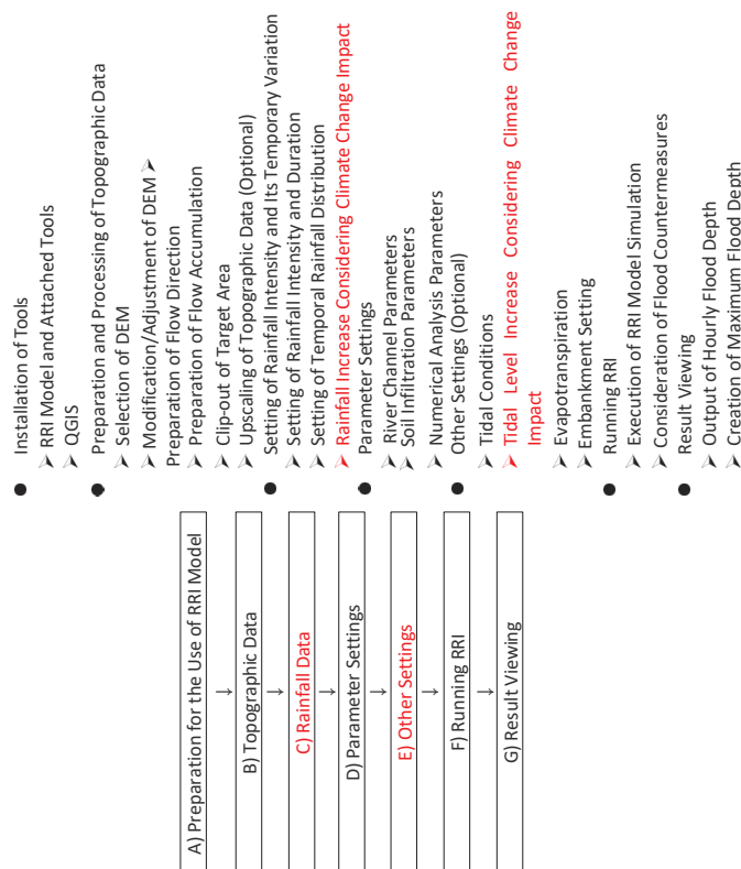
Figure 4 Flow of the RRI Model Simulation Considering Climate Change
