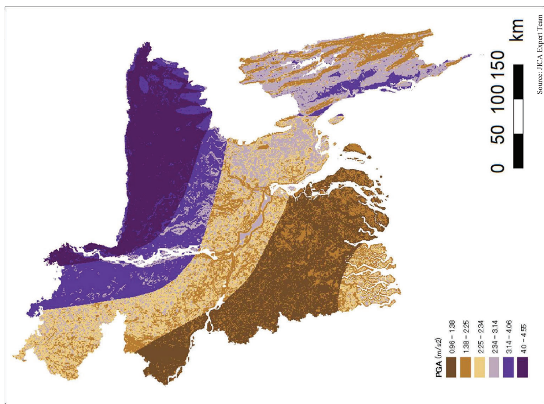
Figure 2.4.5 PGA in Bangladesh
