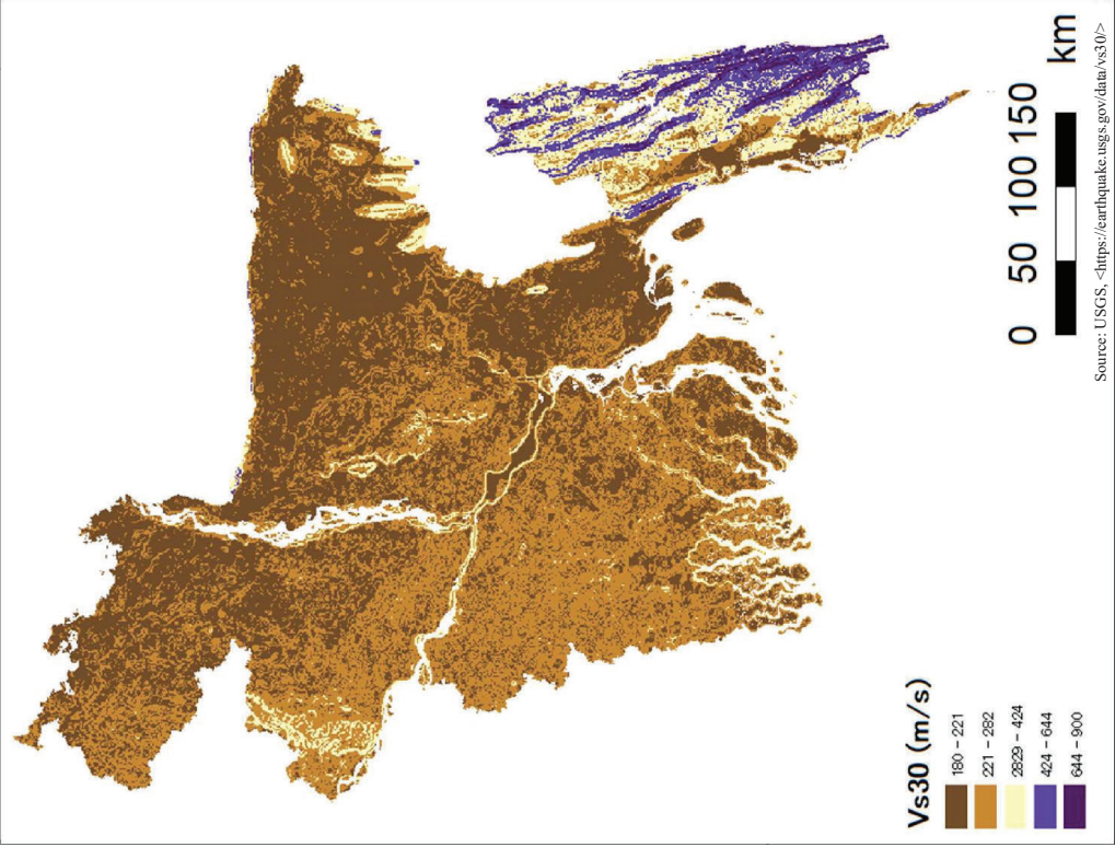
Figure 2.4.4 Vs30 Model in Bangladesh (30 arc-second grid)
