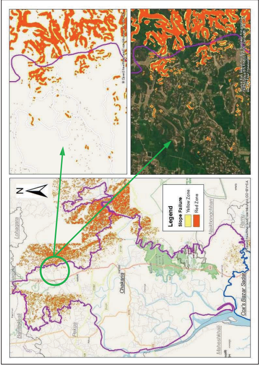
Figure 2.3.4 Result of Slope Failure Hazard Zoning of Chakaria Upazila
