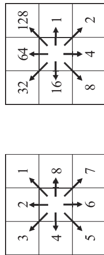
Flow Direction Code as the result of "r.watershed" command in QGIS* Flow Direction applicable to RRI Model
