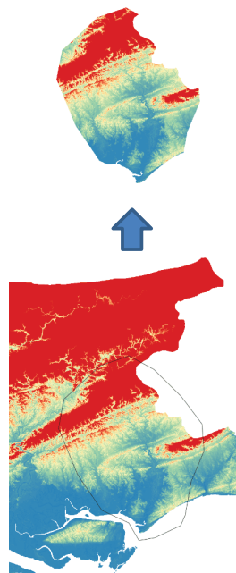
Figure 13 Rough Clip-out of DEM
