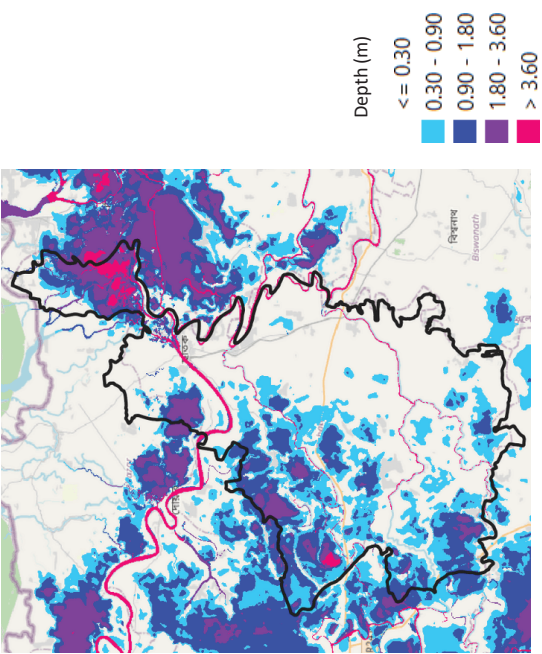
Figure 2.1.6 Sample Output of Flood Analysis (Chhatak Upazila)
