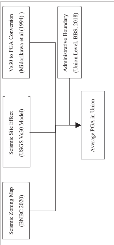
Figure 1-1 Process of Estimating Strength of Earthquake Shaking in Union
