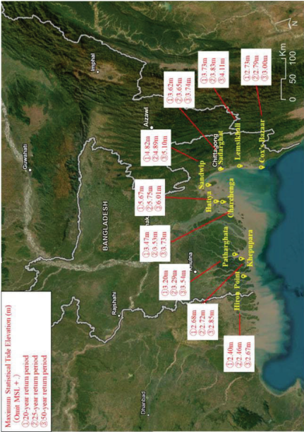
Figure 4-18 Maximum Statistical Tide Elevation(m)
