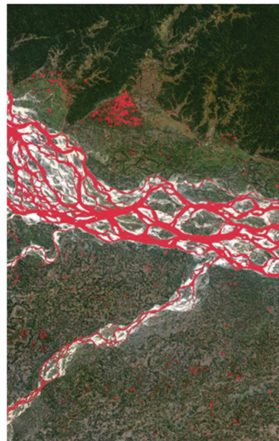
Figure 2.1.16 Extracted Water Body (shown in red)
