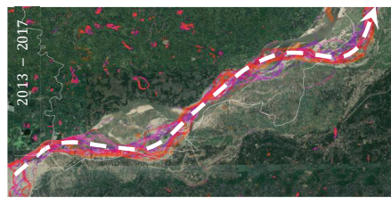
Figure 2.1.17 Tendency of Movement of Teesta River along Ulipur Upazila in Large Scale
