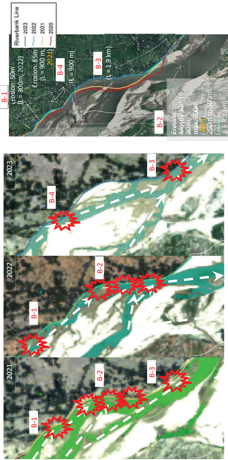
Tendency of Movement of Teesta River along Ulipur Upazila in Local scale
