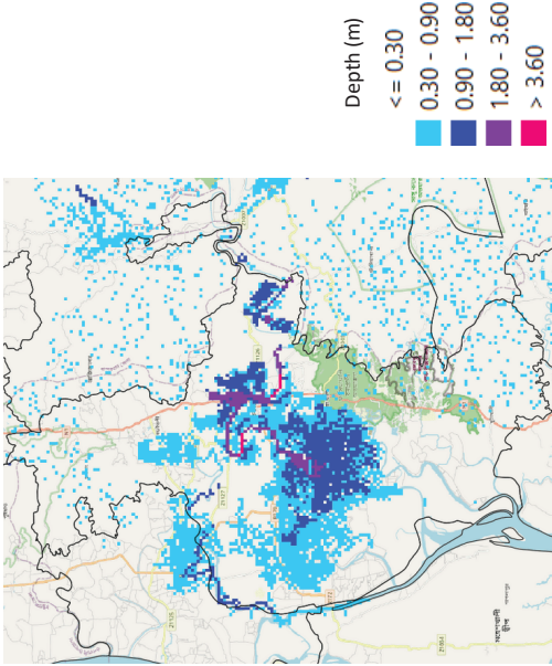
Figure 32 Sample Output of Flood Analysis (Chakaria)
