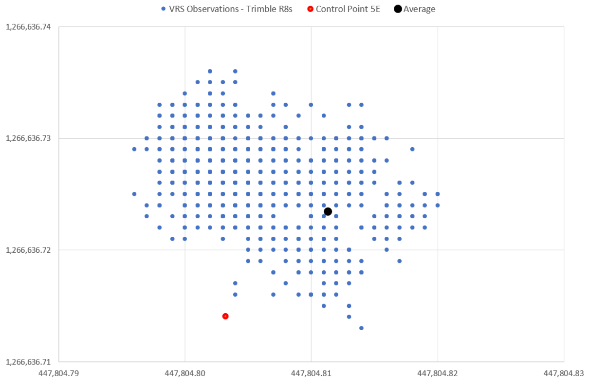
Figure 2-5: Horizontal coordinates of observation over known point 5E with R8s Receiver
