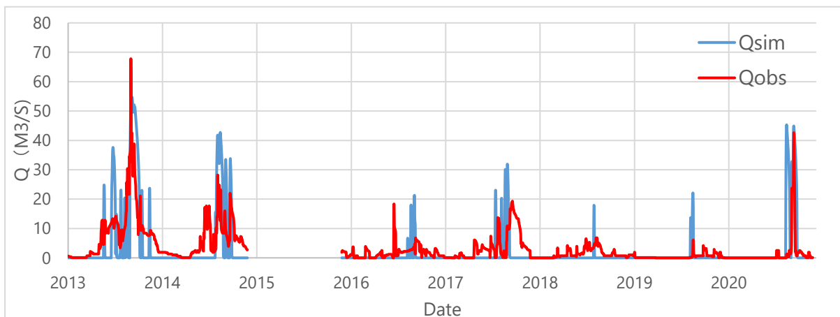
Figure 2-22 Comparison flow of staging gauge in Siem Reap River, 2013-2021
