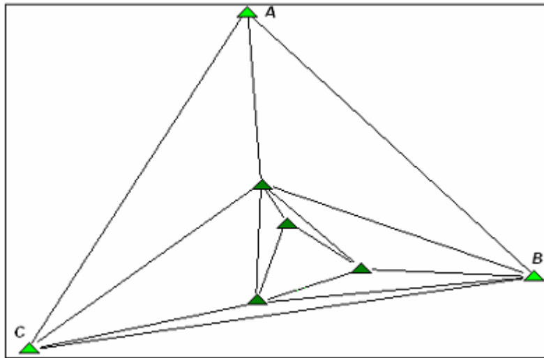
Figure 2-10: Diagram of example network and residual calculations
