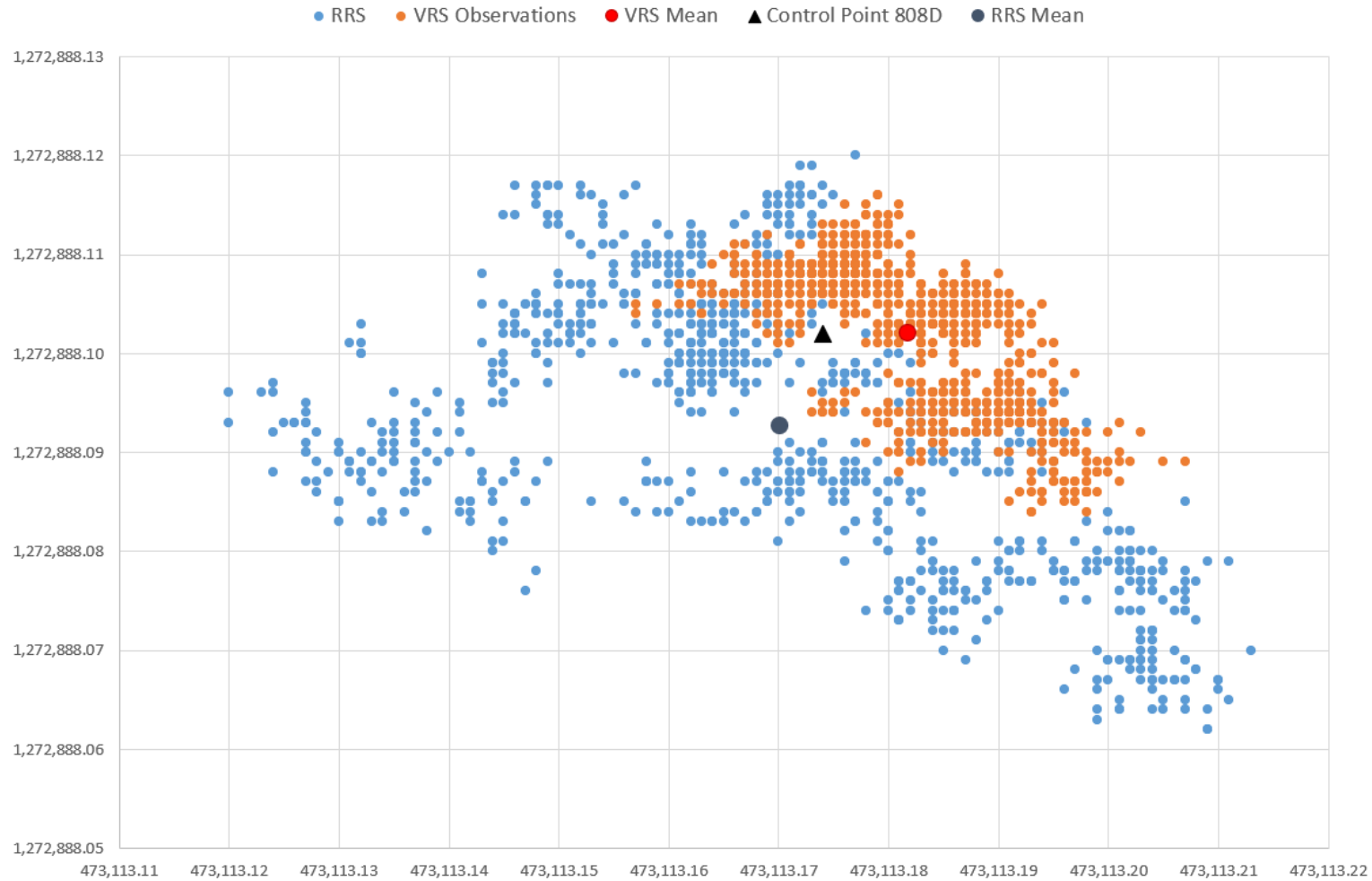
Figure 2-8: Comparison of Observations of RRS vs VRS over known point 808D with R8s receiver
