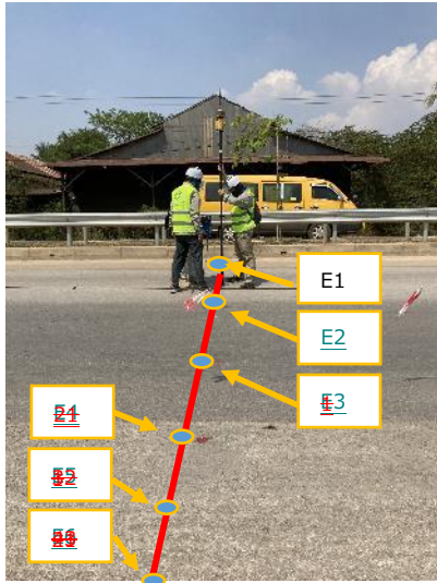
Figure 2-14 Survey for thickness of survey (mmGPS)
