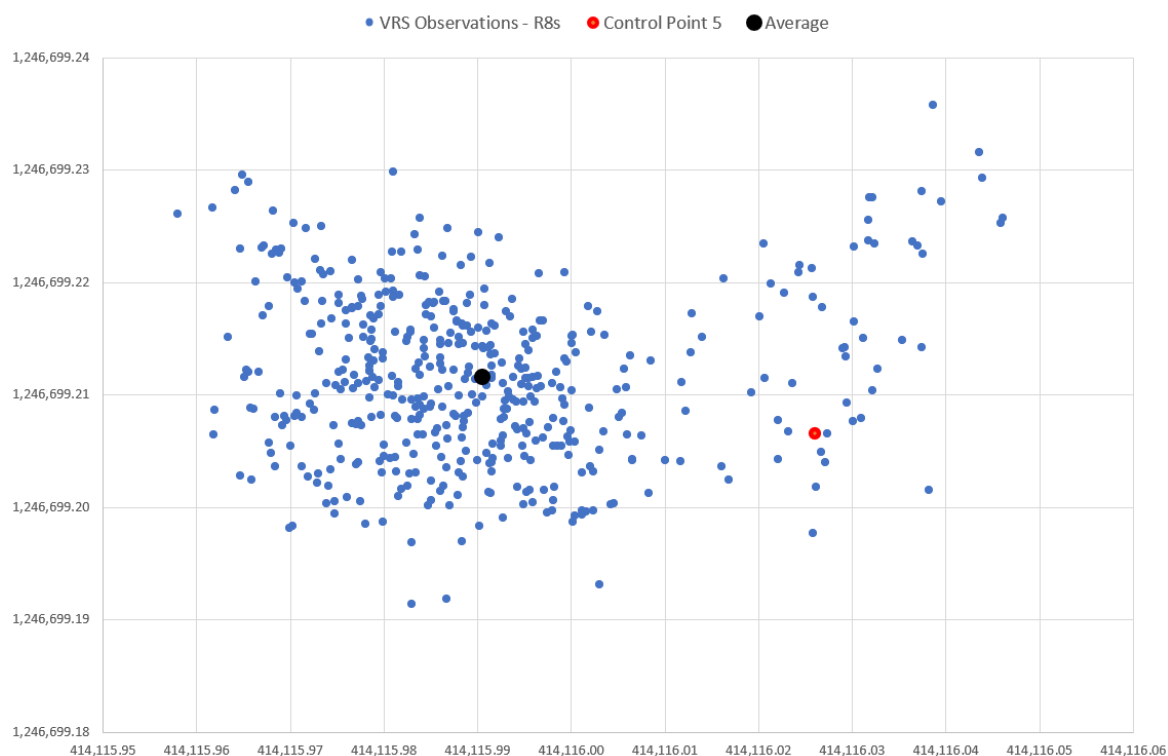
Figure 2-2: Horizontal coordinates of observation over known point 5 with R8s Receiver
