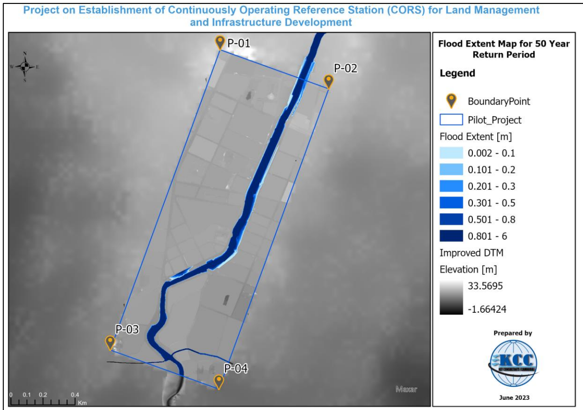
Figure 2-25 Flood extent map for 50-year return period
