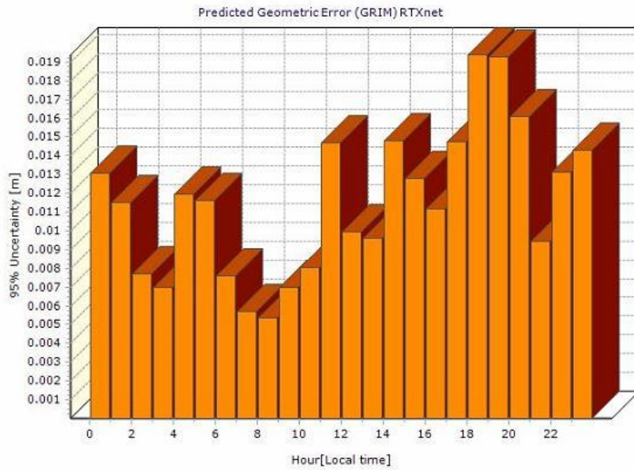
Figure 2-13: Predicted Geometric Error (GRIM) on 23-09-2023
