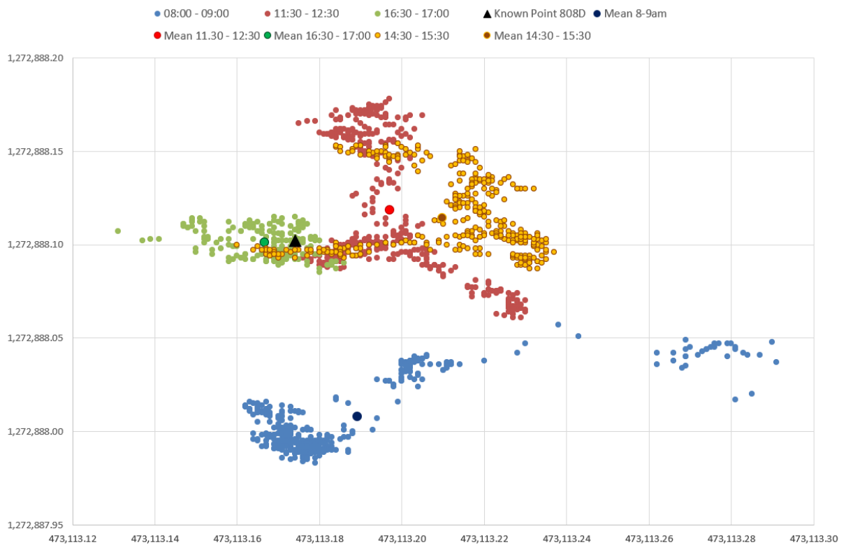
Figure 2-14: Comparison of Observations under different ionospheric conditions
