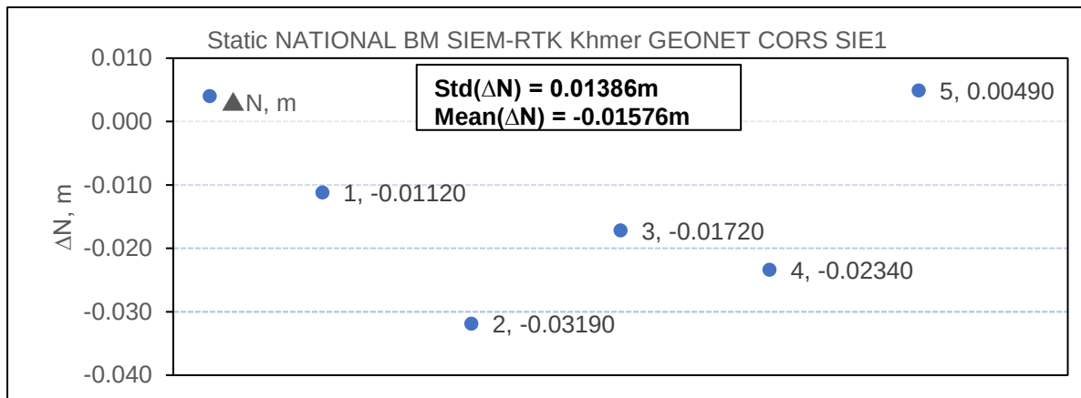
Figure 2-12 The difference of Northing data getting from BM SIEM and Khmer GEONET CORS
