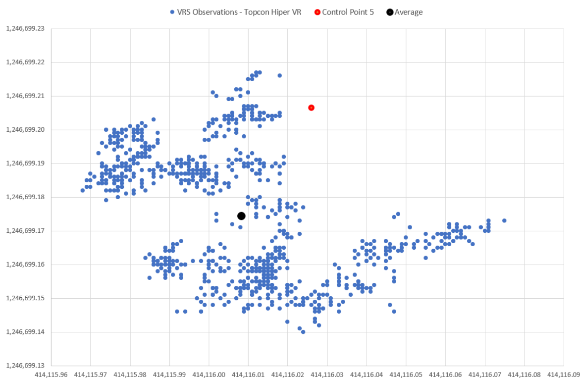
Figure 2-3: Horizontal coordinates of observation over known point 5 with Topcon Hiper VR Receiver
