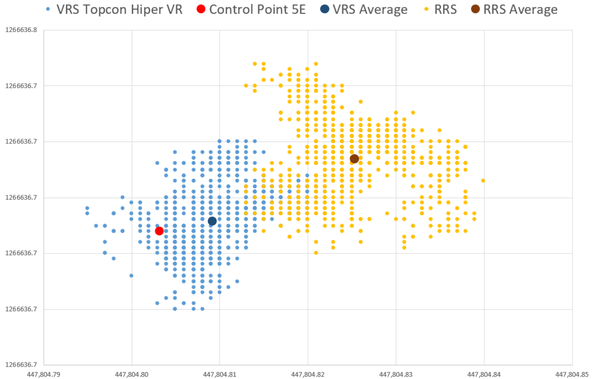
Figure 2-6: Horizontal coordinates of observation over known point 5E with Topcon Hiper VR Receiver
