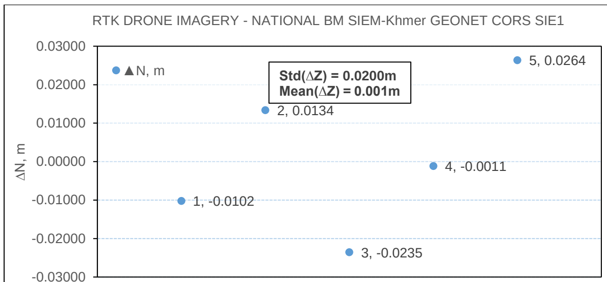
Figure 2-15, the difference of Northing from drone imagery
