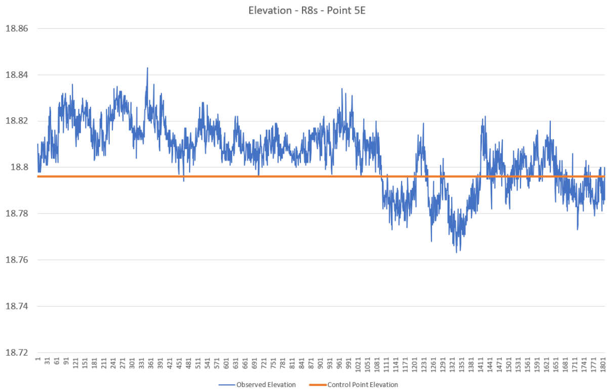
Figure 2-7: Elevation of observation over known point 5E with R8s Receiver
