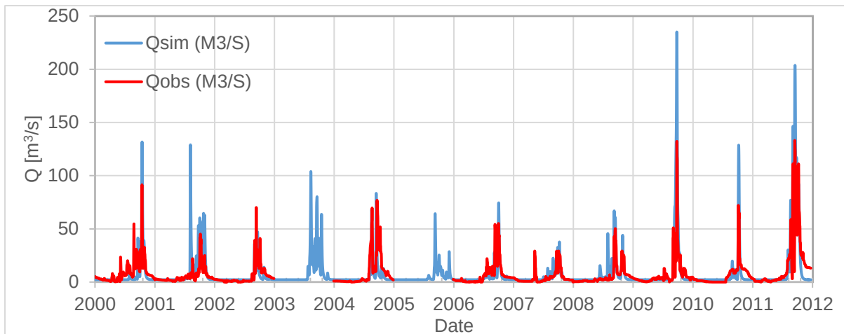
Figure 2-21 Comparison flow of staging gauge in Siem Reap River, 2000-2012
