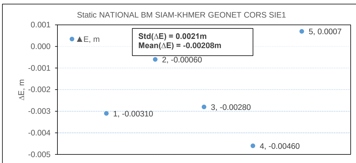
Figure 2-10 The difference of Easting data of checkpoint
