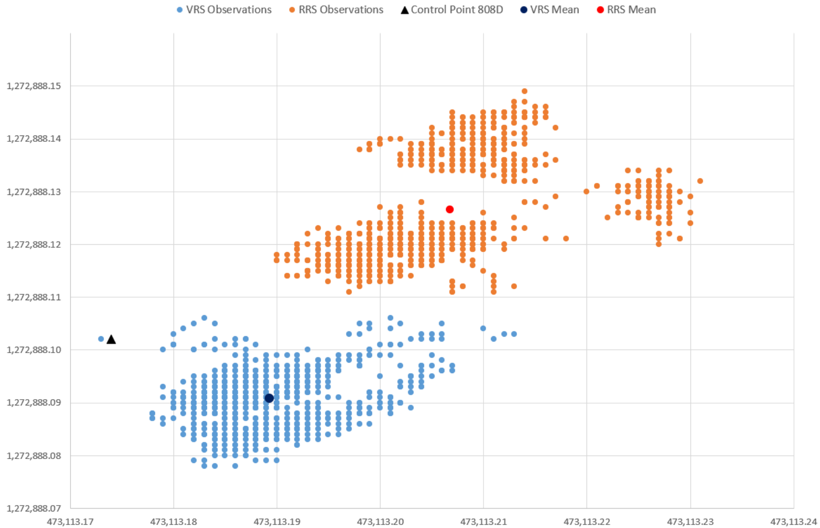
Figure 2-9: Comparison of Observations of RRS vs VRS over known point 808D with Topcon HiPer VR receiver
