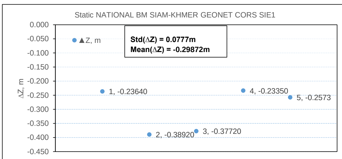
Figure 2-11 The difference of elevation (ellipsoid height) of checkpoints
