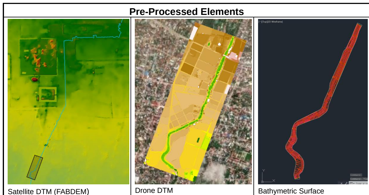
Figure 2-23 Pre-processing of improvement DTM
