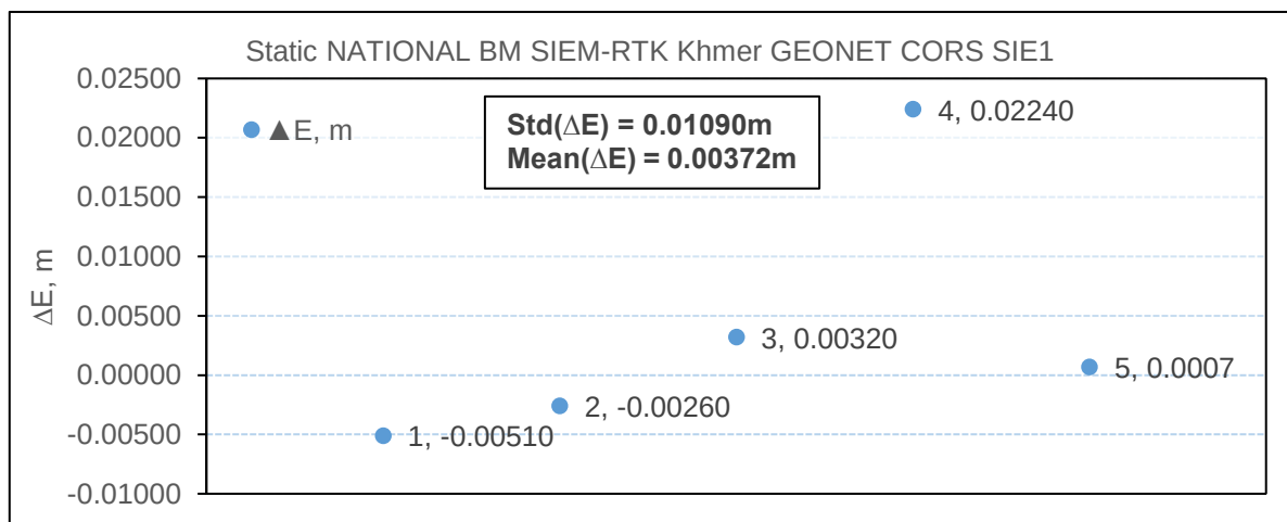
Figure 2-13 The difference of Easting data getting from BM SIEM and Khmer GEONET CORS
