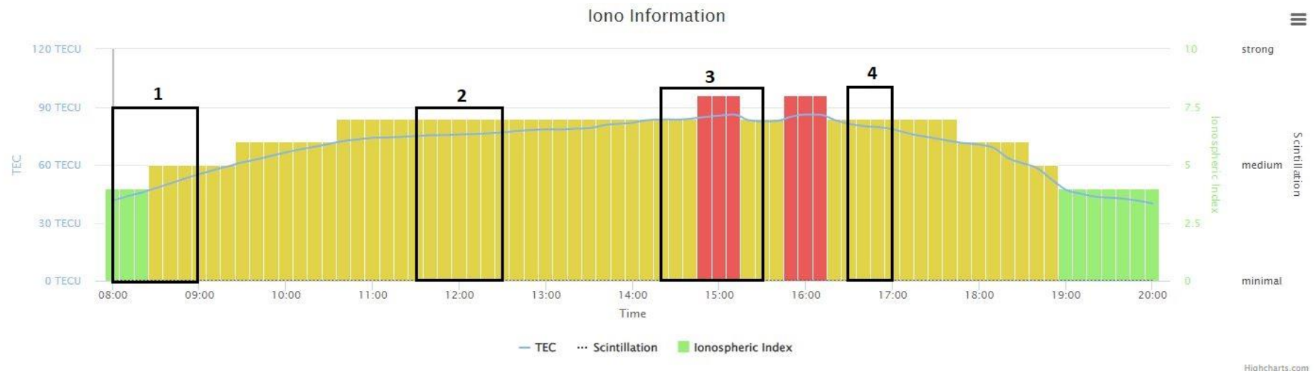
Figure 2-15: Ionospheric Conditions over time on 23-09-2023
