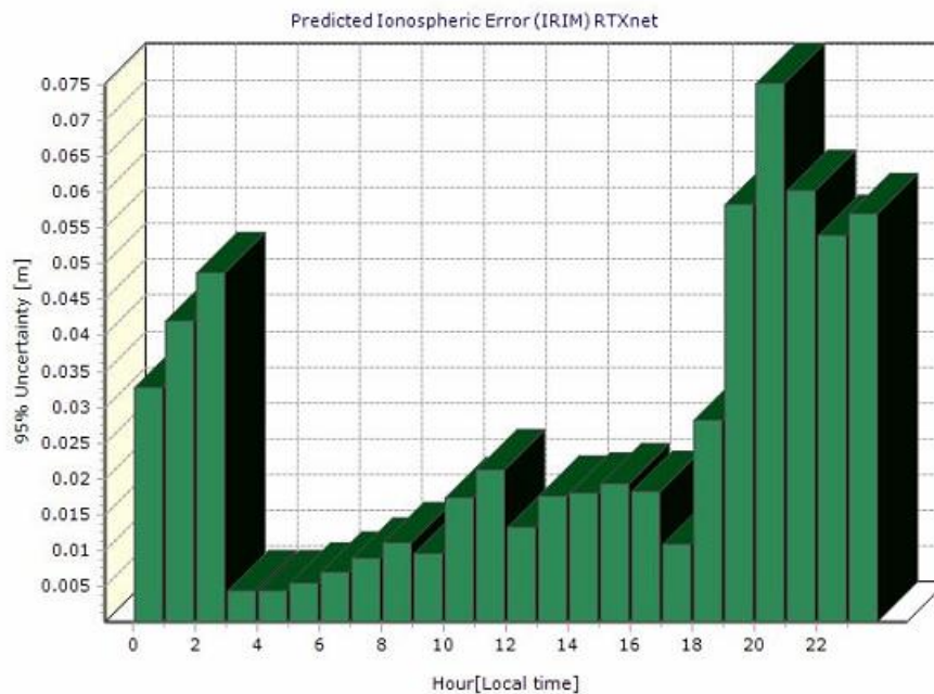
Figure 2-12: Predicted Ionospheric Error (IRIM) on 23-09-2023
