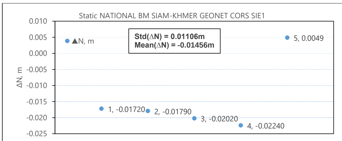
Figure 2-9 The difference of Northing data of Checkpoint
