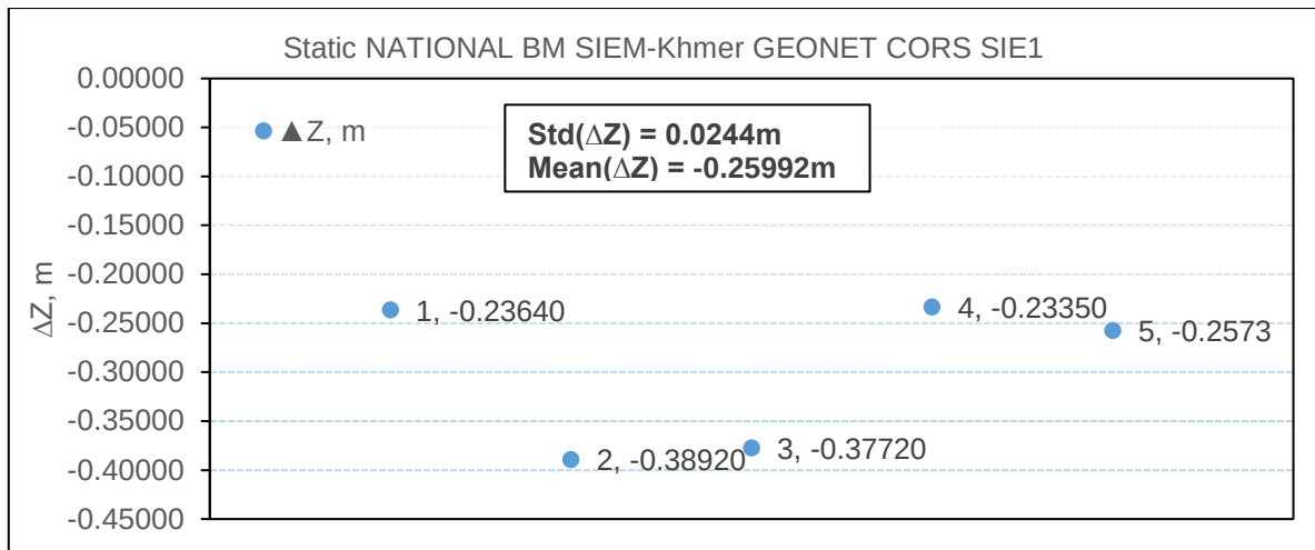
Figure 2-14 The difference elevation (ellipsoid height) of BM SIEM and Khmer GEONET CORS SIE1
