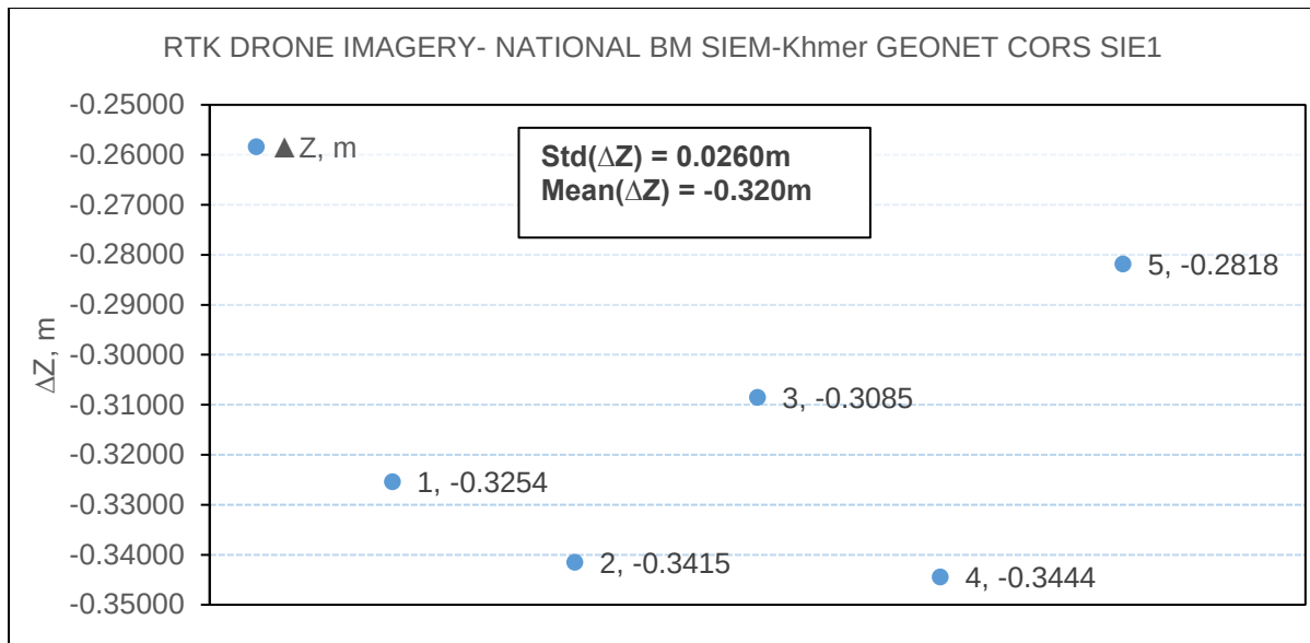
Figure 2-17, the difference of elevation from drone imagery
