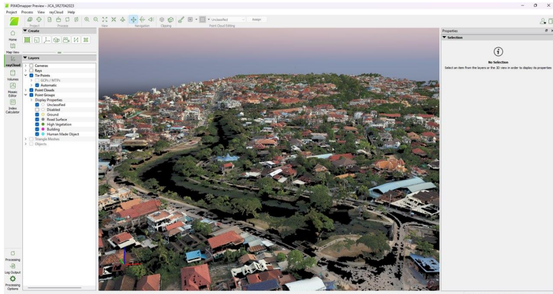
Figure 2-1 Three-dimensional point cloud obtained from drone camera and constructed in Pix4D mapper software
