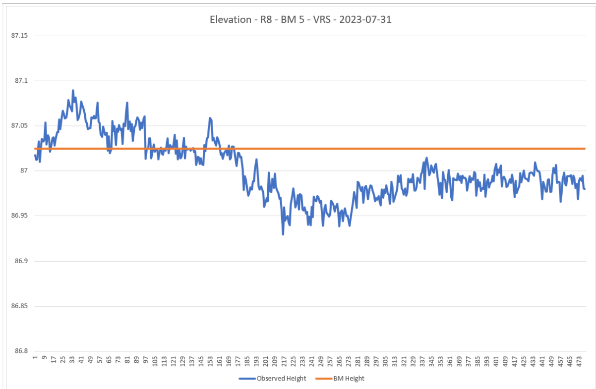
Figure 2-4: Elevation of observations over known point 5
