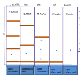
Experiment on optimal bund spacing Runoff plots in croplands
