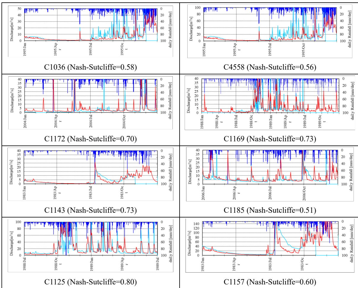
Figure D-86 Results of Tank Model Calibration of WRR-IV, Palawan
