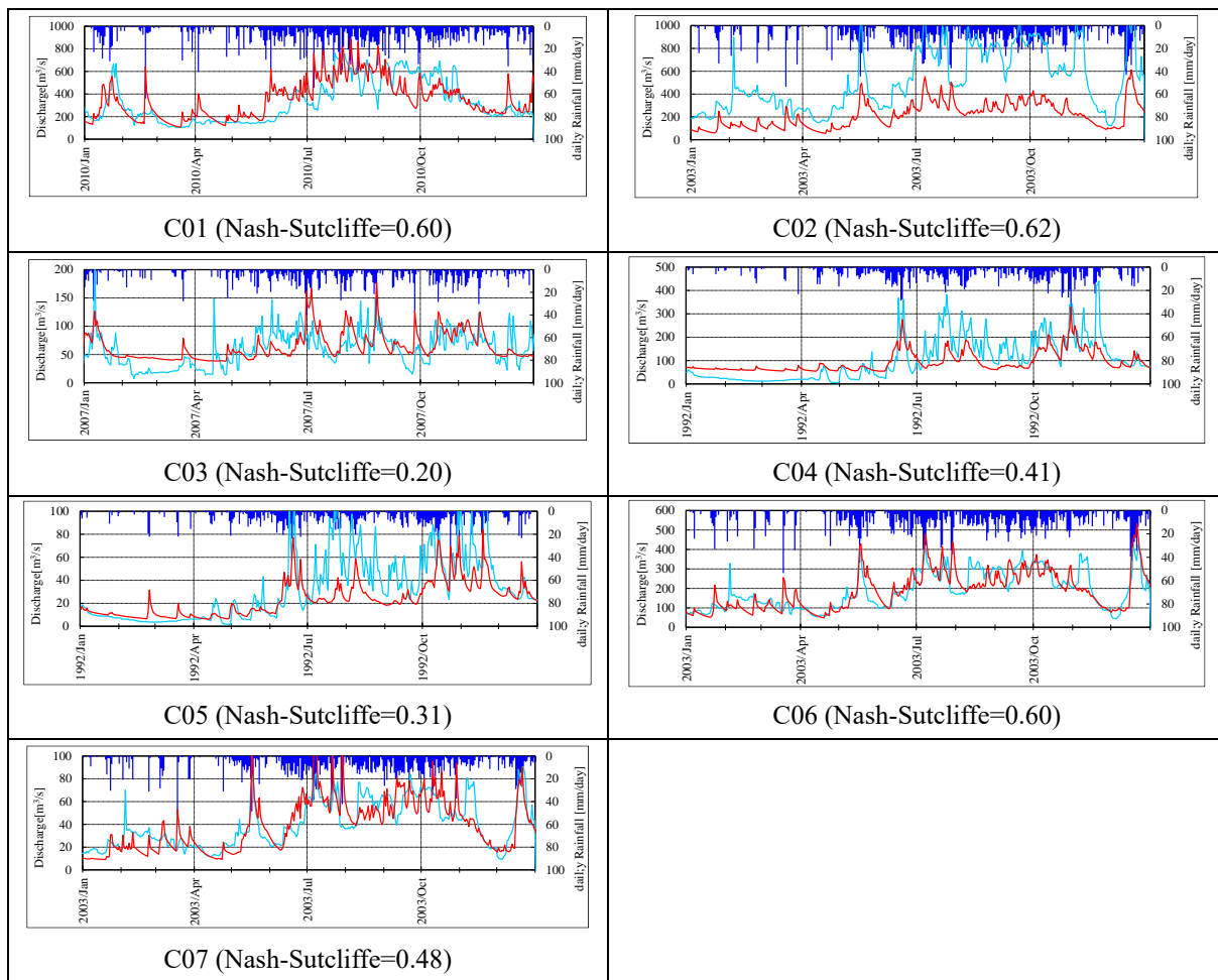
Figure D-100 Results of Tank Model Calibration of WRR-XII, Mindanao
