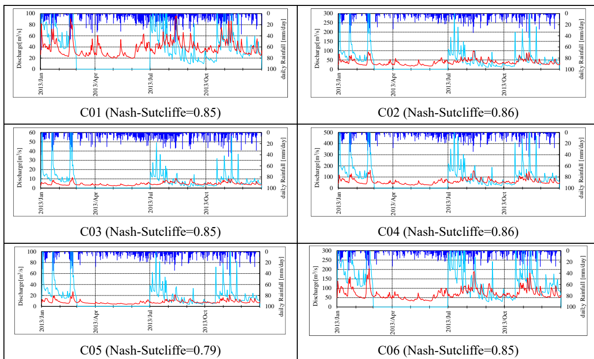
Figure D-98 Results of Tank Model Calibration of WRR-XI, Davao
