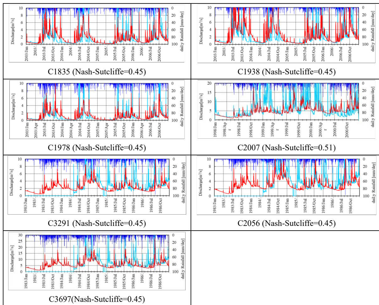
Figure D-92 Results of Tank Model Calibration of WRR-VII, Negros Oriental
