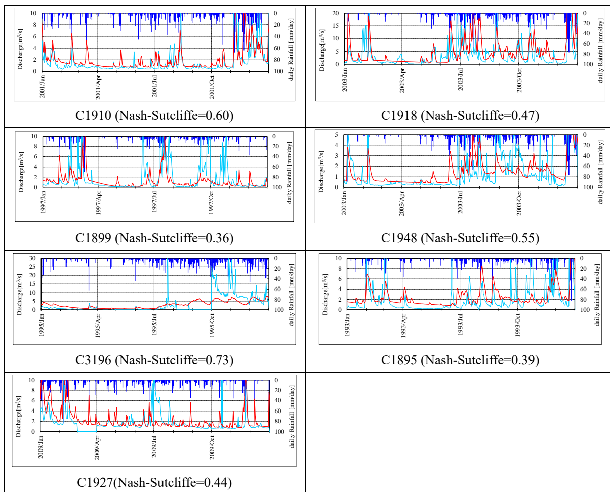
Figure D-93 Results of Tank Model Calibration of WRR-VII, Bohol
