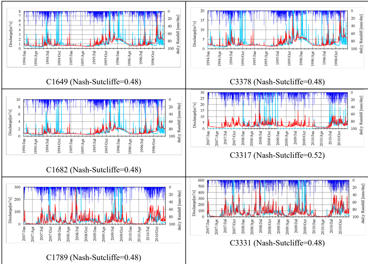
Figure D-90 Results of Tank Model Calibration of WRR-VI, Ilog-Hilabangan
