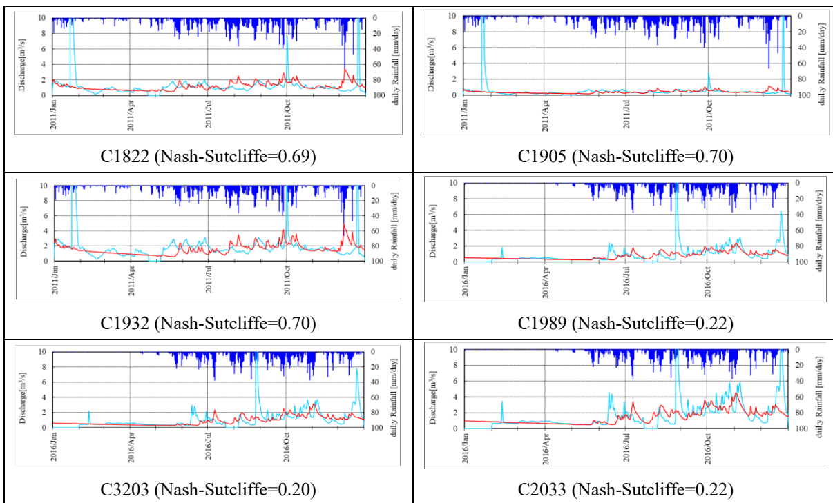
Figure D-86 Results of Tank Model Calibration of WRR-IV, Palawan
