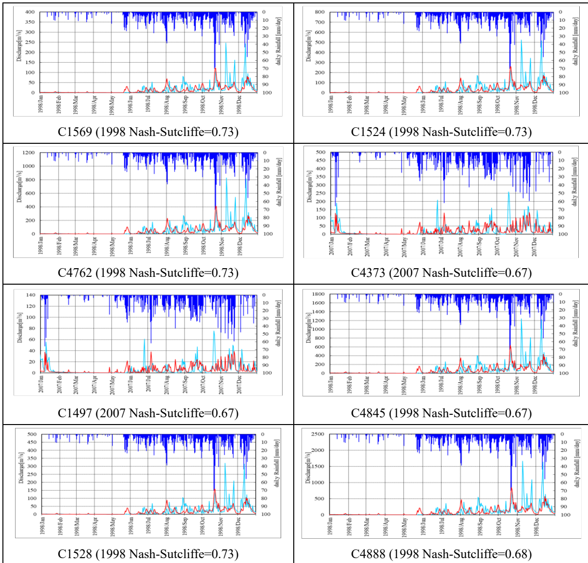
Figure D-87 Results of Tank Model Calibration of WRR-V, Bicol
