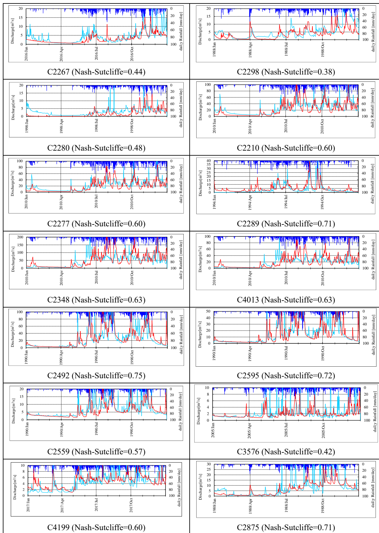
Figure D-95 Results of Tank Model Calibration of WRR-IX, Southwestern Mindanao
