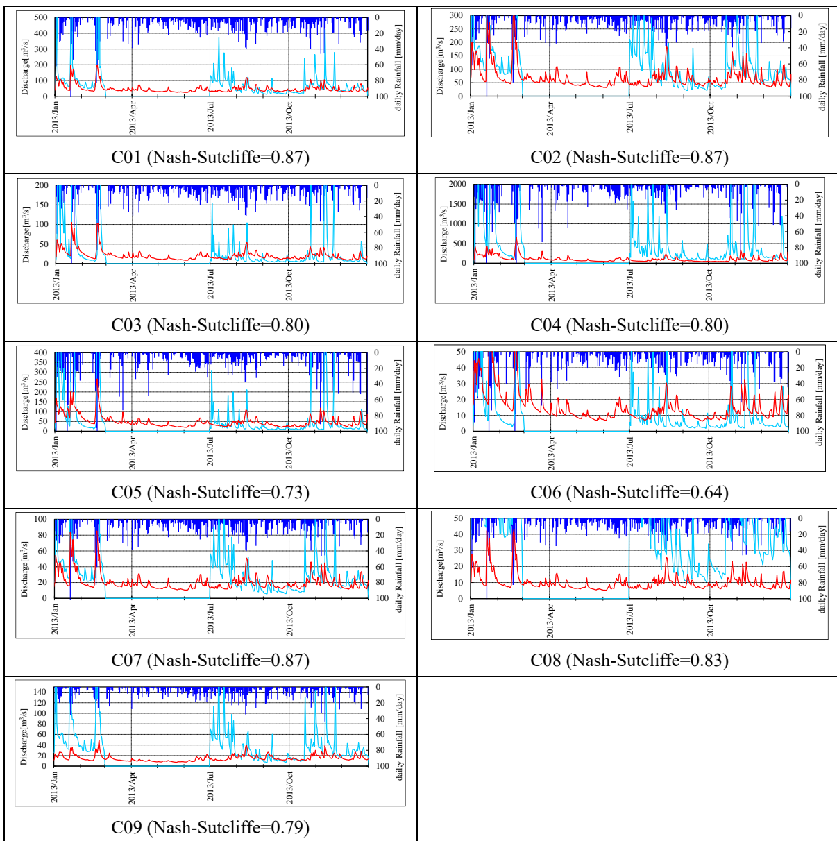
Figure D-99 Results of Tank Model Calibration of WRR-XI, Tagum Libuganon
