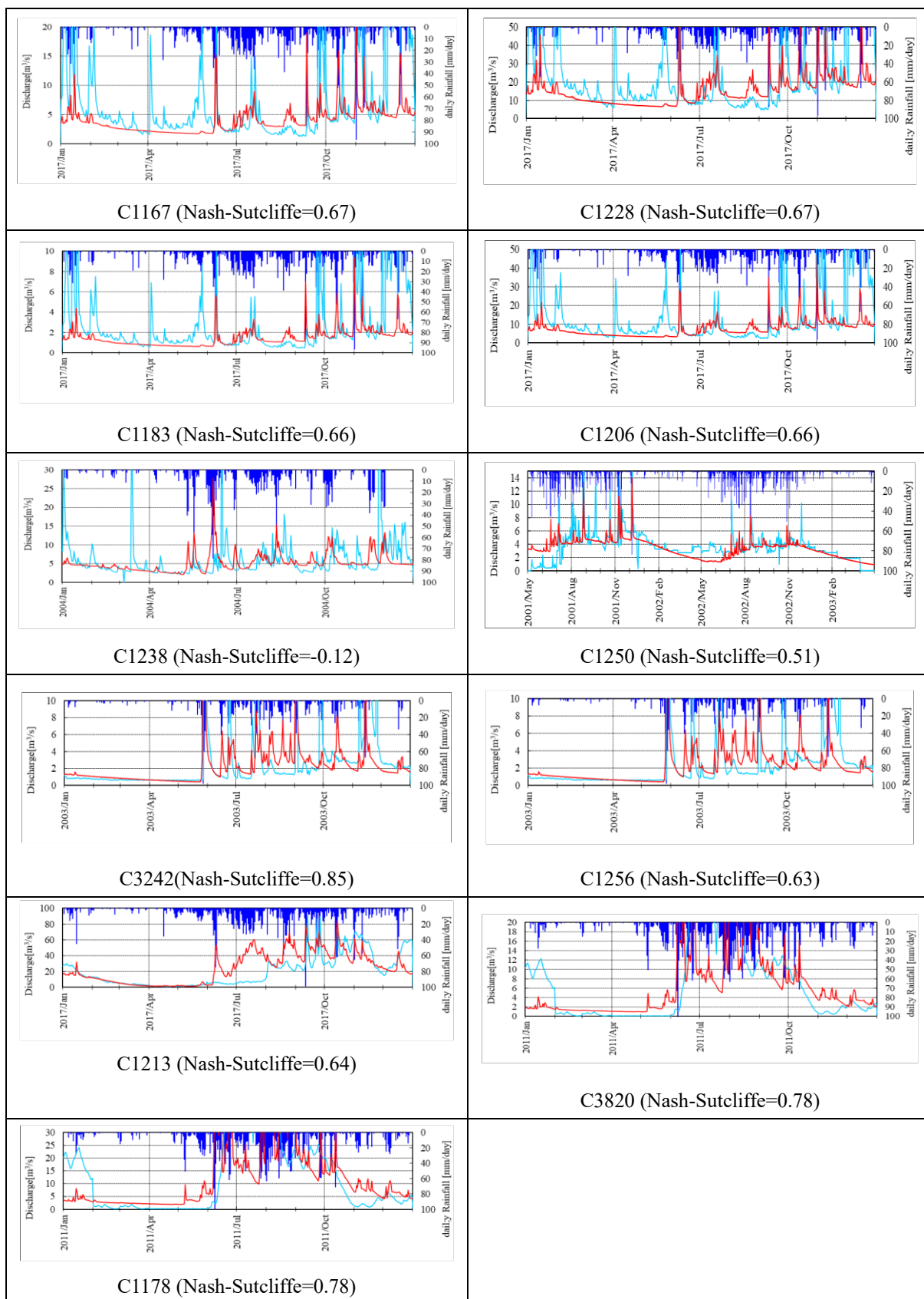
Figure D-85 Results of Tank Model Calibration of WRR-IV, Mindoro
