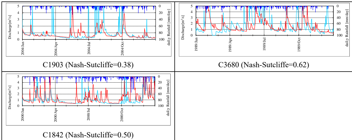
Figure D-90 Results of Tank Model Calibration of WRR-VI, Ilog-Hilabangan
