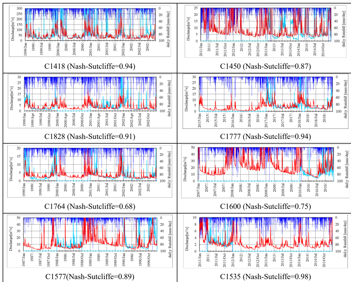
Figure D-94 Results of Tank Model Calibration of WRR-VIII, Samar & Leyte
