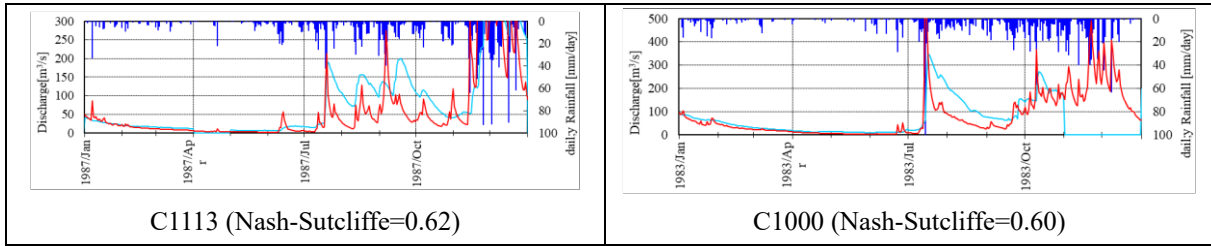
Figure D-87 Results of Tank Model Calibration of WRR-V, Bicol
