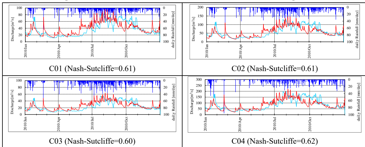
Figure D-96 Results of Tank Model Calibration of WRR-X, Agusan
