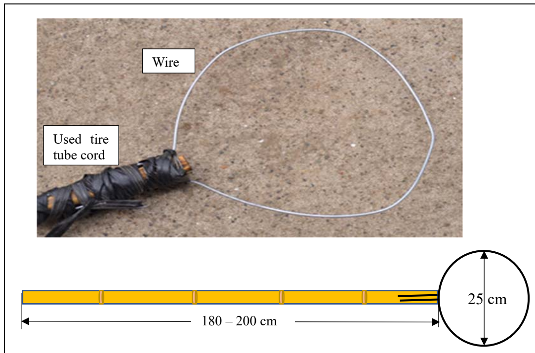
Figure 11 Wire Weeder
