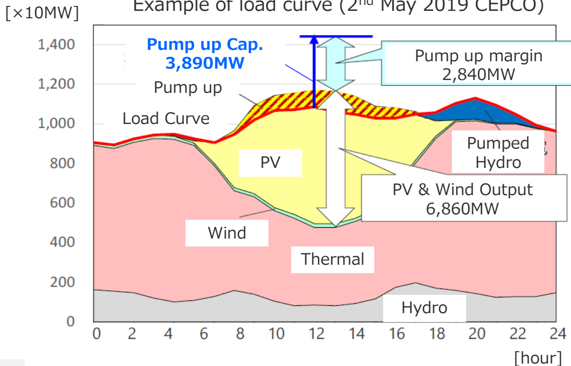
Example of load curve (2 nd May 2019 CEPCO)
