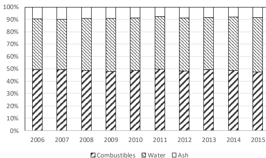
Figure 3-11 Yearly Changes of 3 Components
