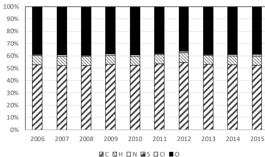
Figure 3-12 Yearly Changes of Elemental Composition
