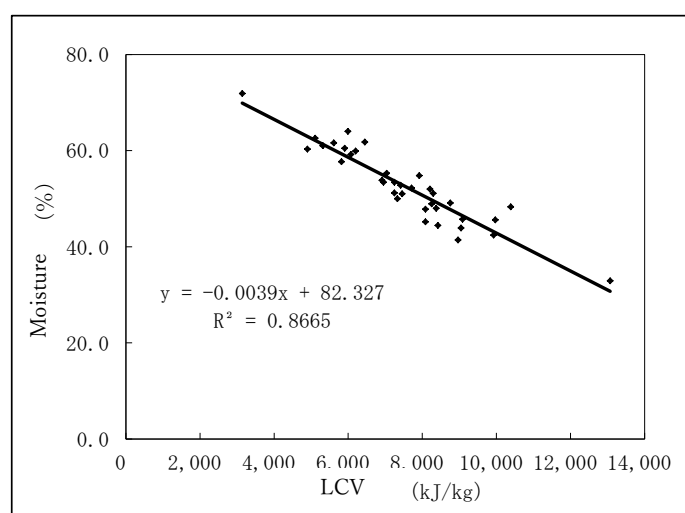
Figure 3-15 Approximated Linear Function of LCV and moisture content
