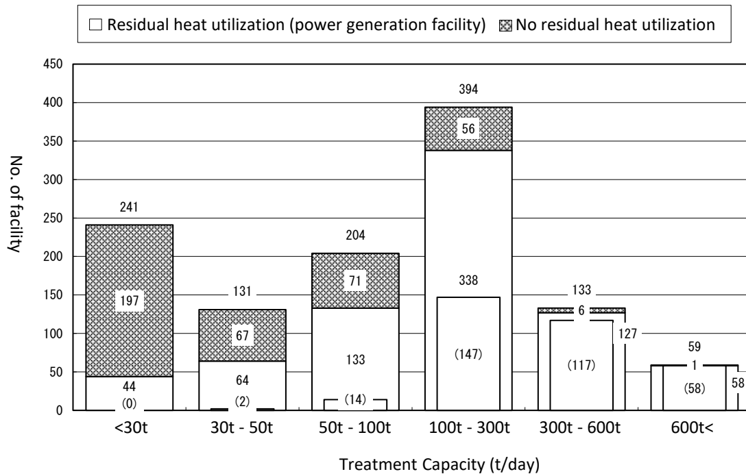
Figure 7-7 Situation of residual heat usage by waste incineration facilities (record of 2014)
