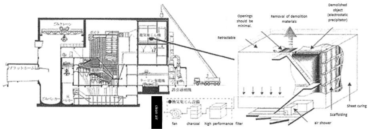
Figure 6-1 Image of dismantling plant
