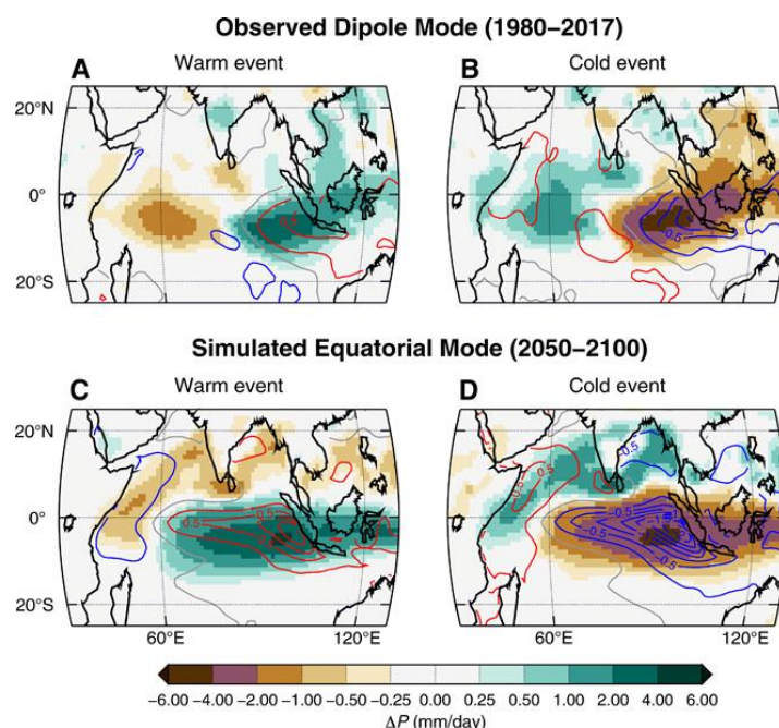
Figure 5 Rainfall impacts of current and future modes of climate variability in the IO
