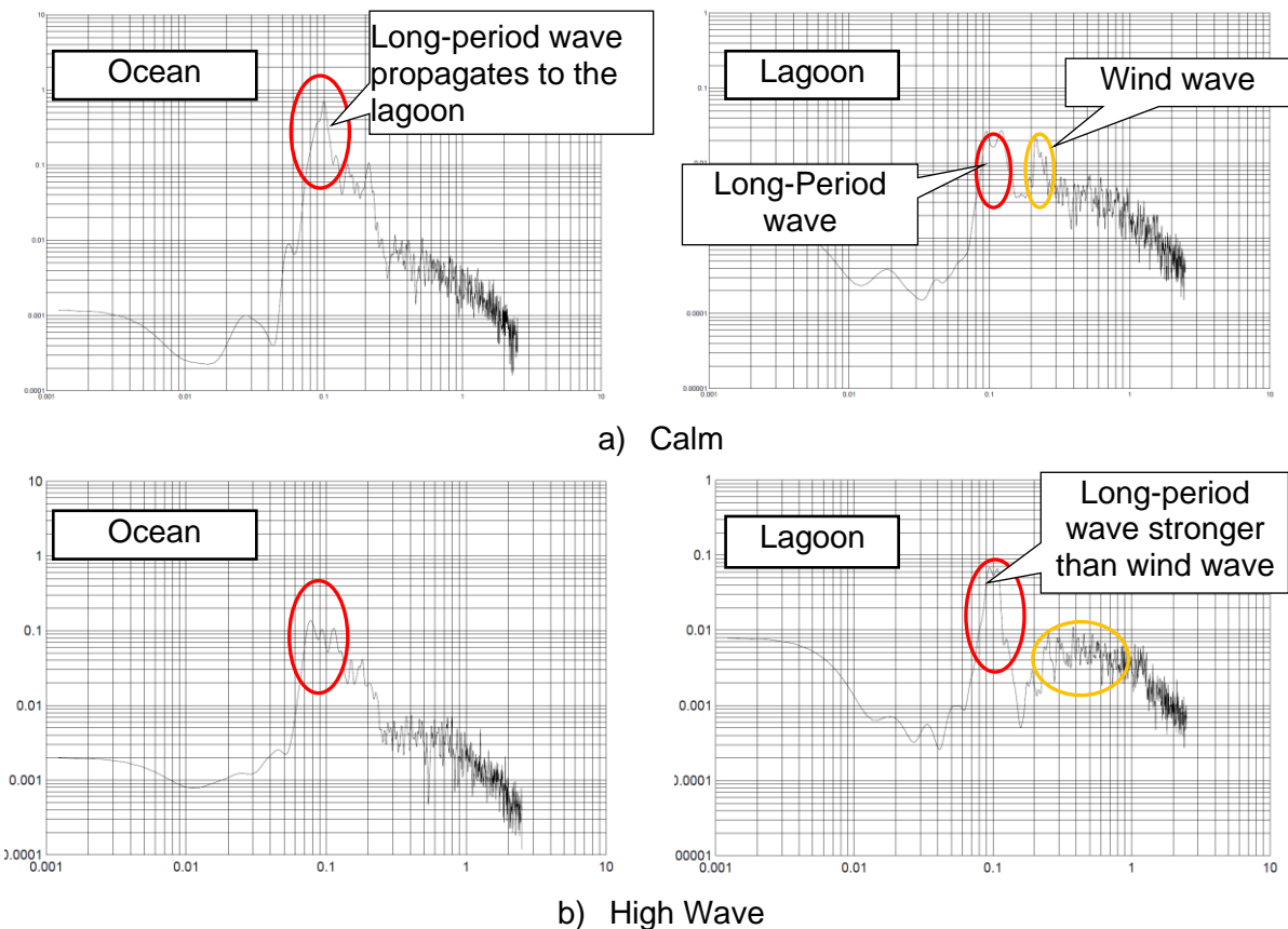
Figure 2.1.18 Power Spectrum of Wave (Vertical : Spectrum Density ( \text{m}^2\text{s} ), Horizontal : Frequency (Hz))
