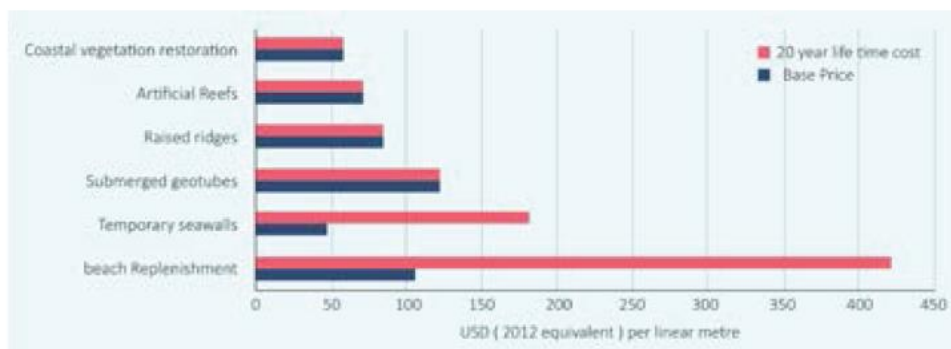
Figure 43 Cost comparison of soft engineering solutions for coastal adaptation
