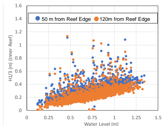
Figure 14 Relation of wave height and water level at inside of coral reef (ocean side, Addu)
