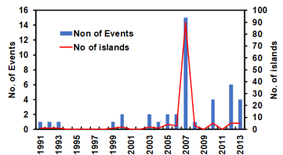
Figure 21 Frequency of inundation caused by swell wave and number of islands affected
