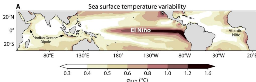
Figure 2 Variability of Sea Surface Temperature
