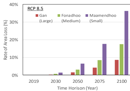
Figure 24 Rate of Area Loss by Coastal Erosion
