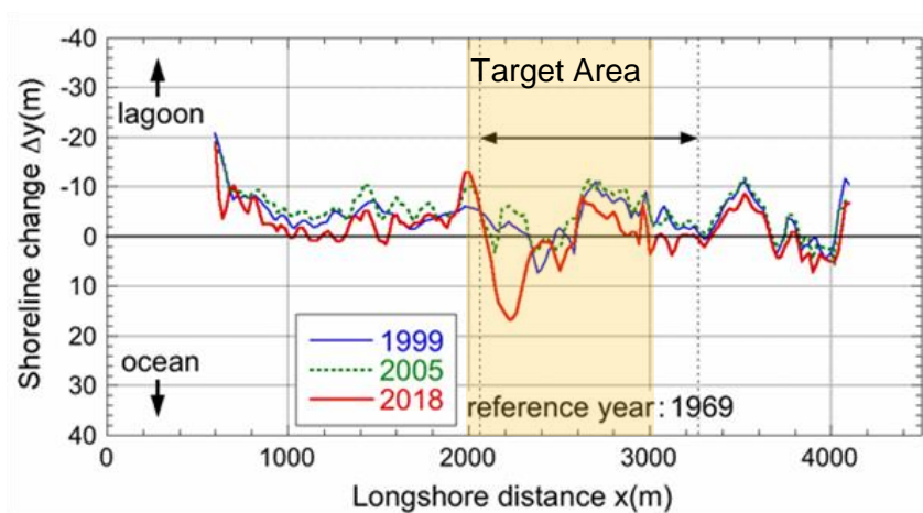
Figure 31 Long-Term Shoreline Change at Fonadhoo from 1969
