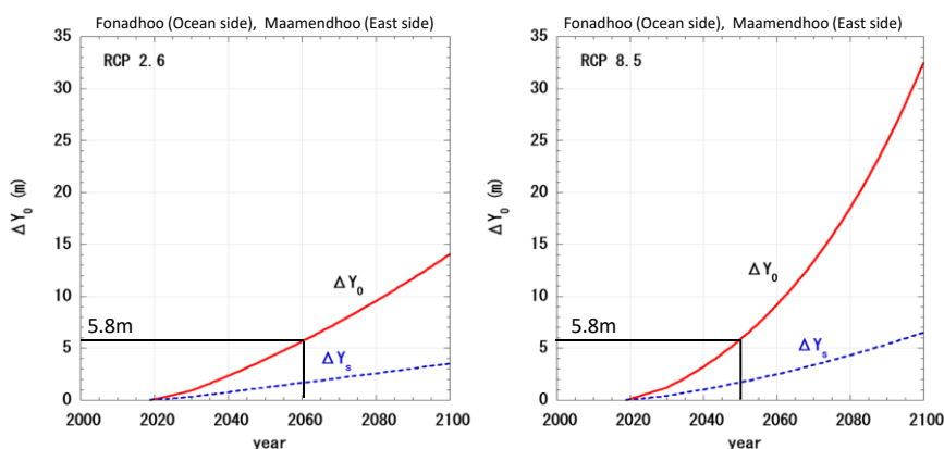
Figure 36 Estimated Beach Retreat due to SLR at Fonadhoo and East Side of Maamendhoo
