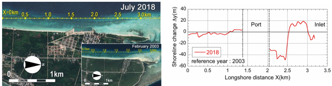
Figure 27 Coastal Erosion at down-drift side of Port Construction
