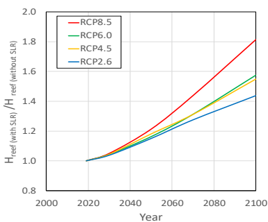
Figure 23 Increase of Wave Height on Coral Reef due to SLR
