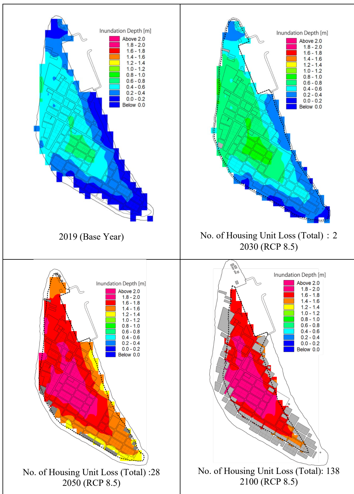
Figure B.1 Compound Damage Map Due to Erosion and Flooding with SLR for Maamendhoo
