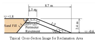
Figure 44 Proposed Intervention for Activity 2.2 funded by GCF
