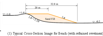
Figure 44 Proposed Intervention for Activity 2.2 funded by GCF
