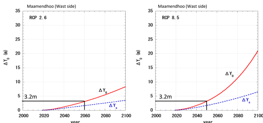
Figure 37 Estimated Beach Retreat due to SLR at West Side of Maamendhoo
