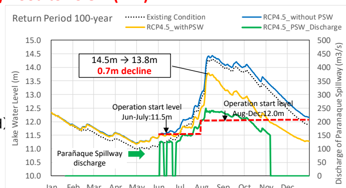
Figure 1-2 Effect of Parañaque Spillway of 100-year Return Period (with Climate Change, D=13m, Max. Discharge=240m 3 /s)
