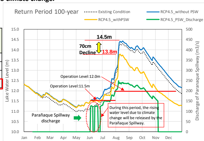
Figure 2-2-1 Analysis Results of Water Level Fluctuation (100-year, D=13m)
