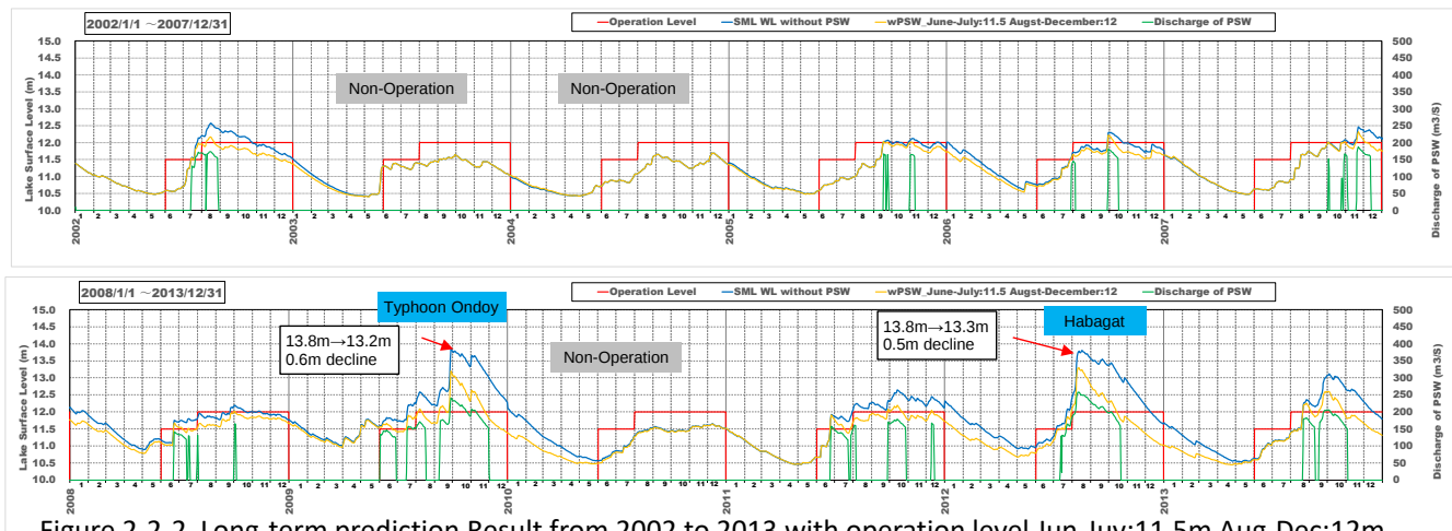
Figure 2-2-2 Long-term prediction Result from 2002 to 2013 with operation level Jun-July:11.5m Aug-Dec:12m (Diameter of Tunnel is 13.0m)
