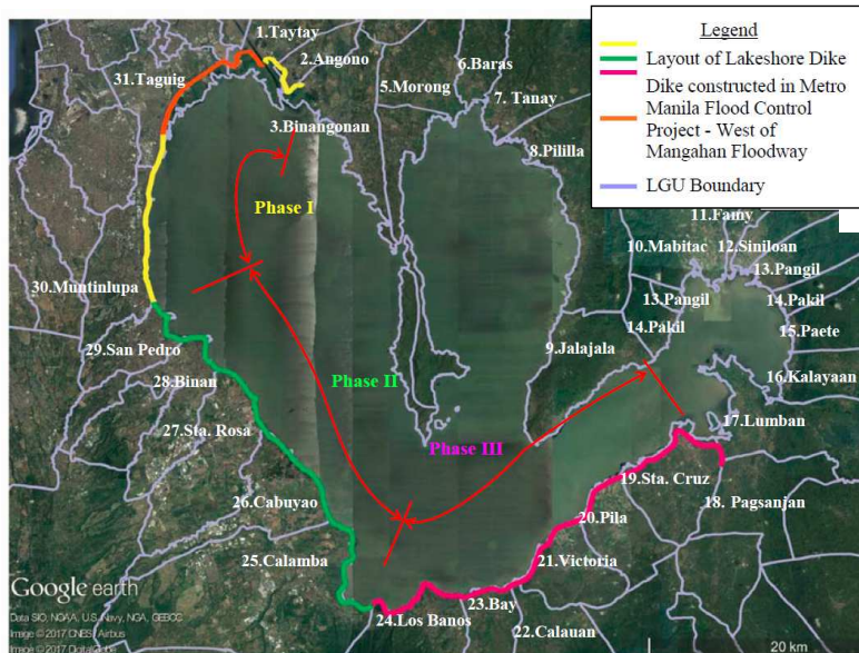
Figure 1-4 Layout of Lakeshore Diking System (Phase I, II, III)
