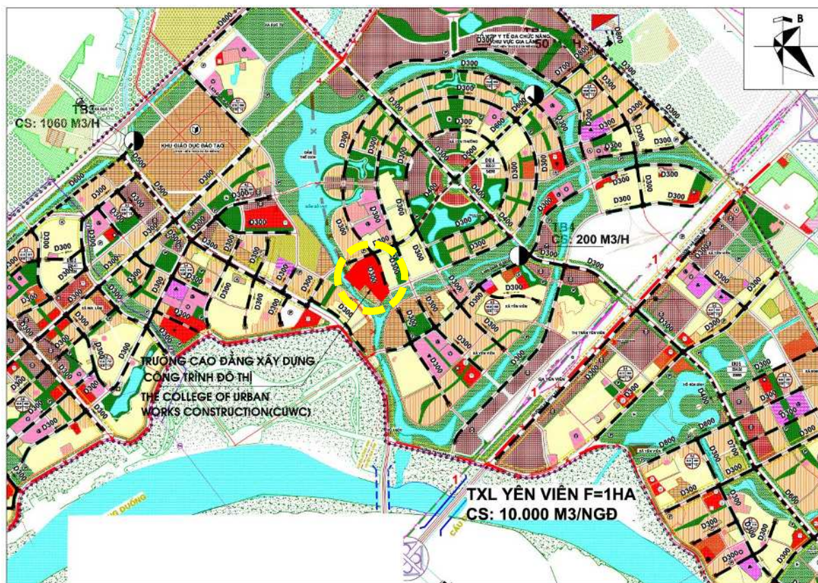
Figure 2.2.1 Mater Plan of Drainage System by 2030 (N9 Zoning)
