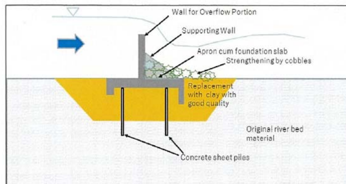
Figure A8-2 Sketch of the Structure of Vay Kor Dam (based on the Information from DOWRAM Svay Rieng Province)
