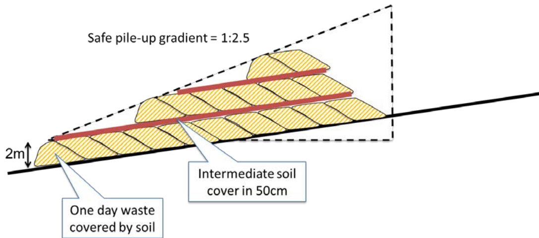
Figure 21: Practice of waste piling and soil covering
