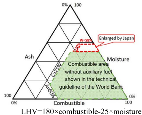
Figure 23: Relationship between the 3 components (moisture, ash, and combustible) in incineration of waste
