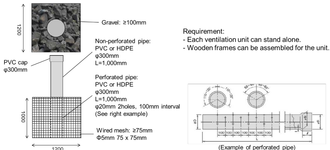
Figure 18: Gas ventilation unit
