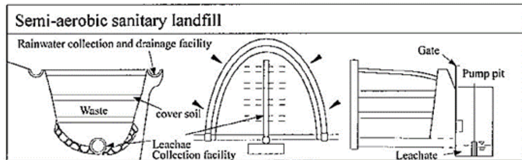
Figure 7: Semi-aerobic landfill
