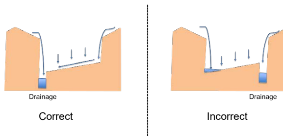
Figure 24: One-side drainage
