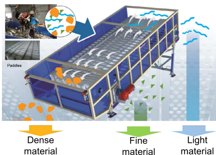
Figure 8: Ballistic separator
