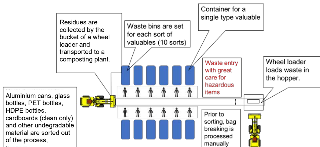
Figure 6: Manual sorting
