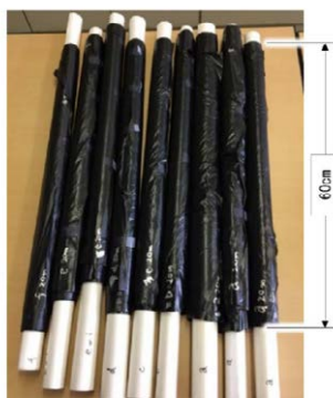
Biodegradable mulch film prototype
