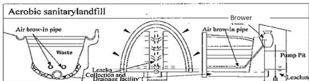
Figure 8: Aerobic landfill
