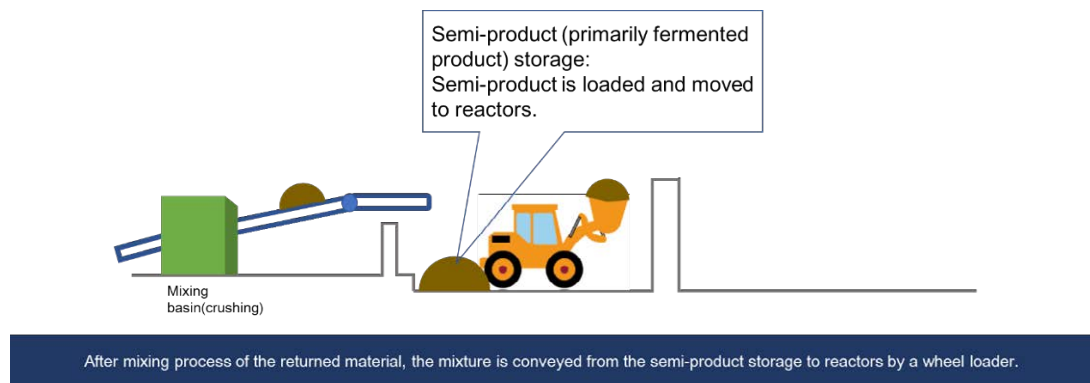
Figure 13: Semi-product Storage
