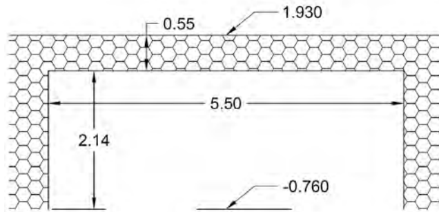
Bridge # C-2 @ Pinnameda Road
