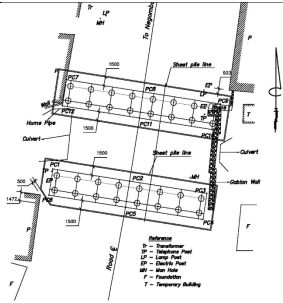
New Bridge (15 m in length) (Source: SLDC presentation material)
