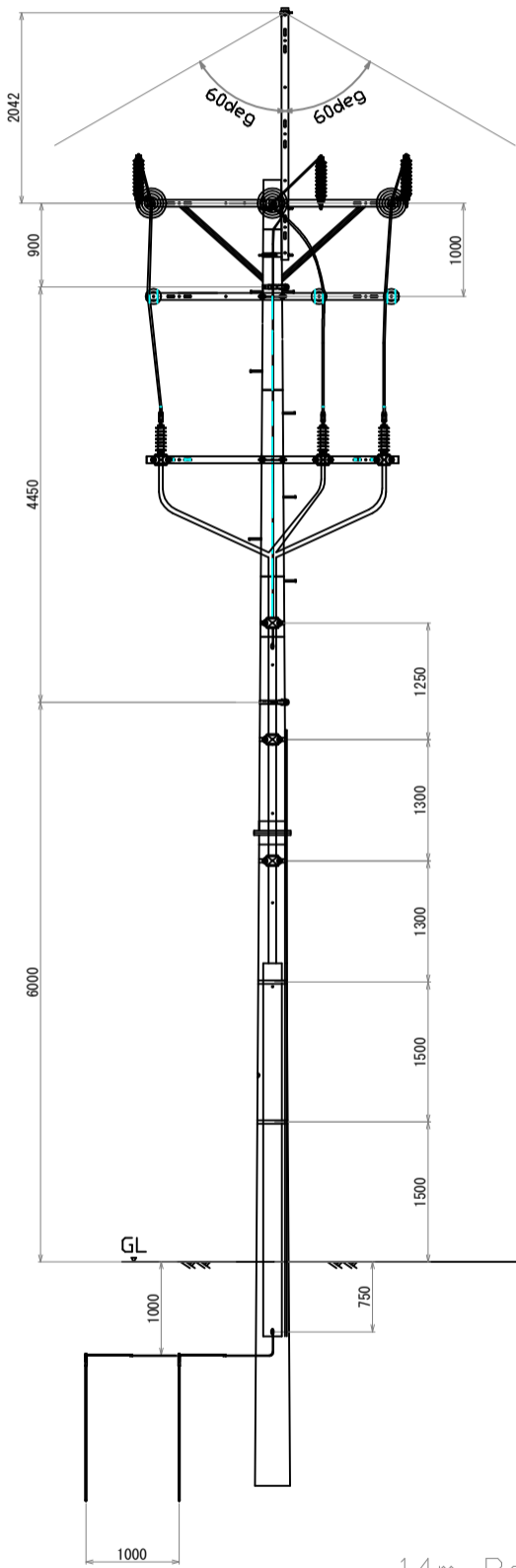
14m Pole Type H
