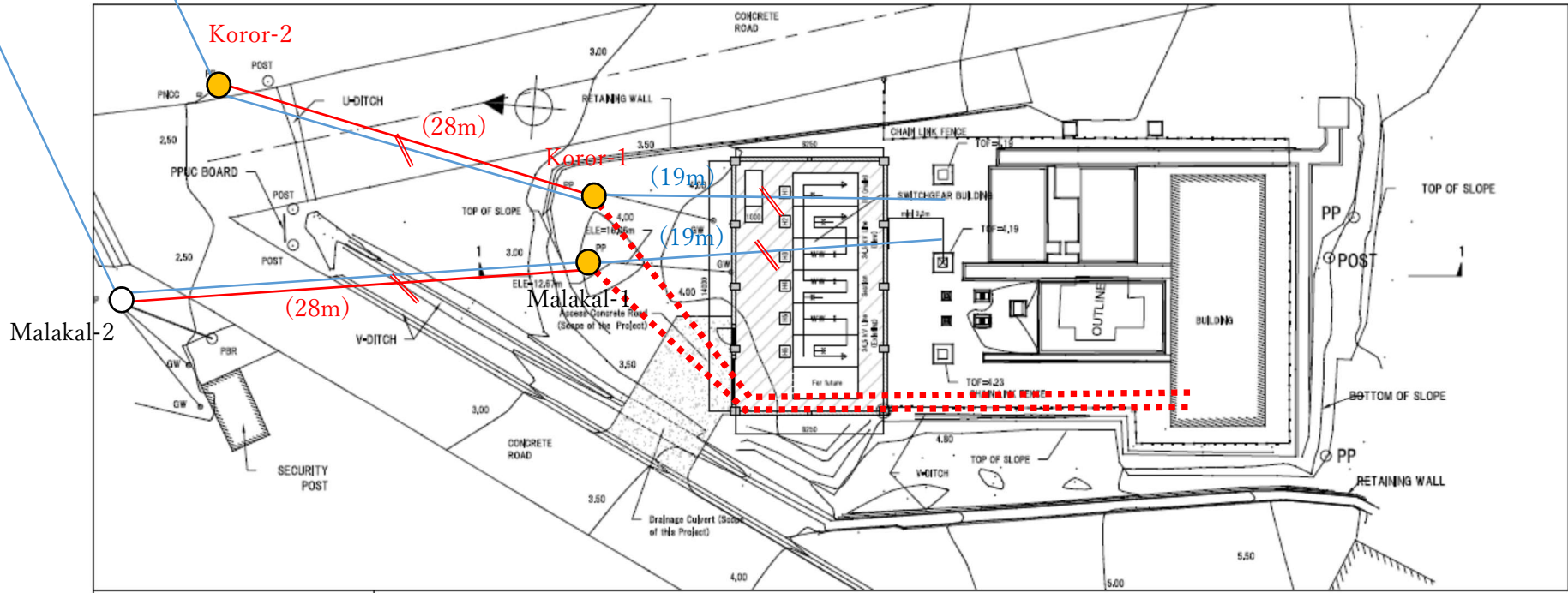
13.8kV Malakal Substation
