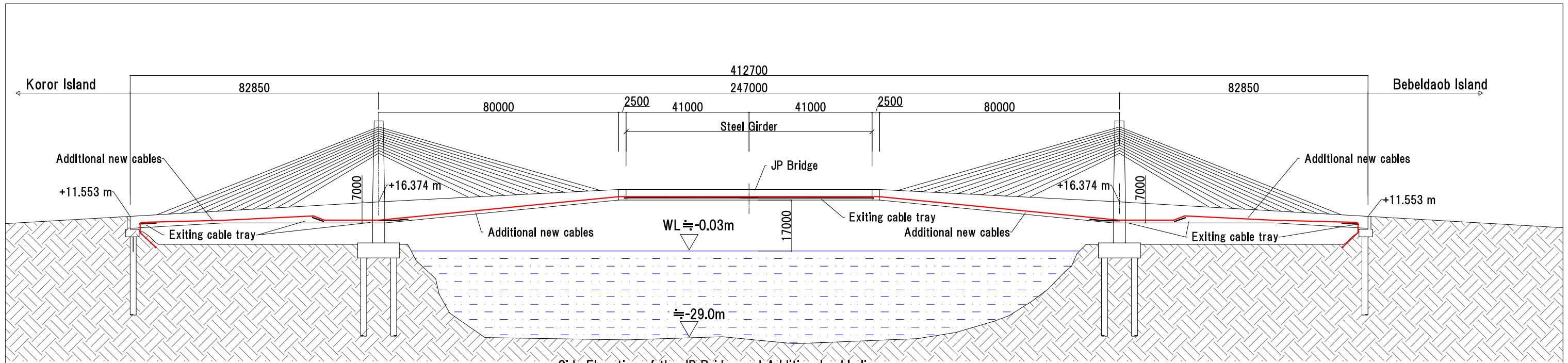
Side Elevation of the JP Bridge and Additional cable line
