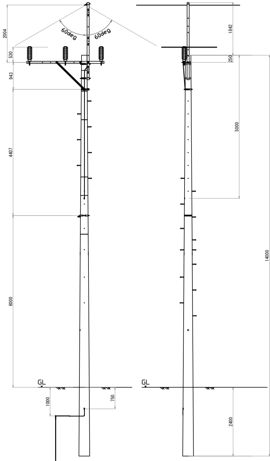
14m Pole Type A
