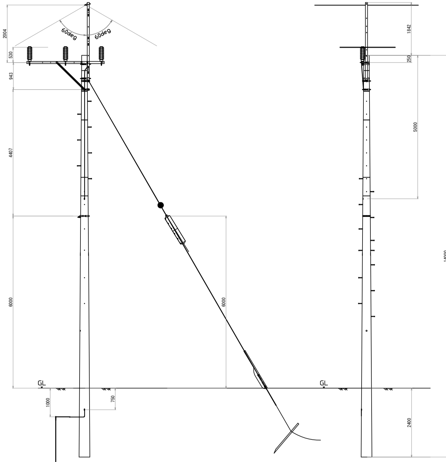
14m Pole Type B
