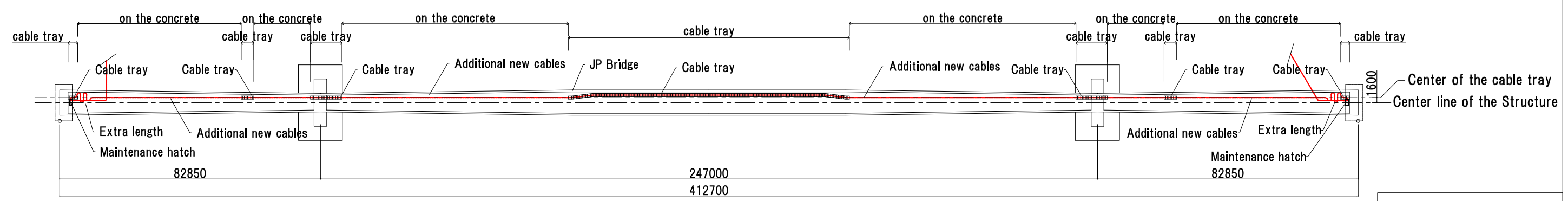
Inside plan of the JP Bridge and Additional cable line (Section A-A)
