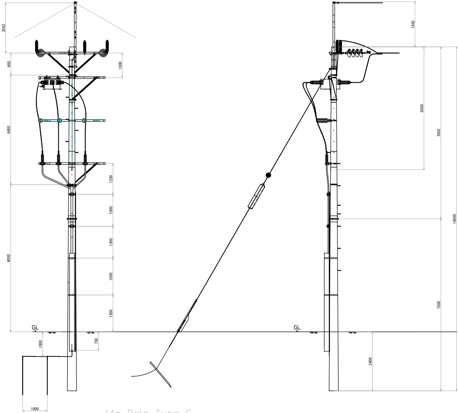
14m Pole Type G
