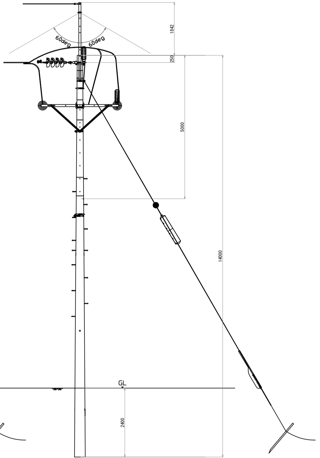
14m Pole Type F
