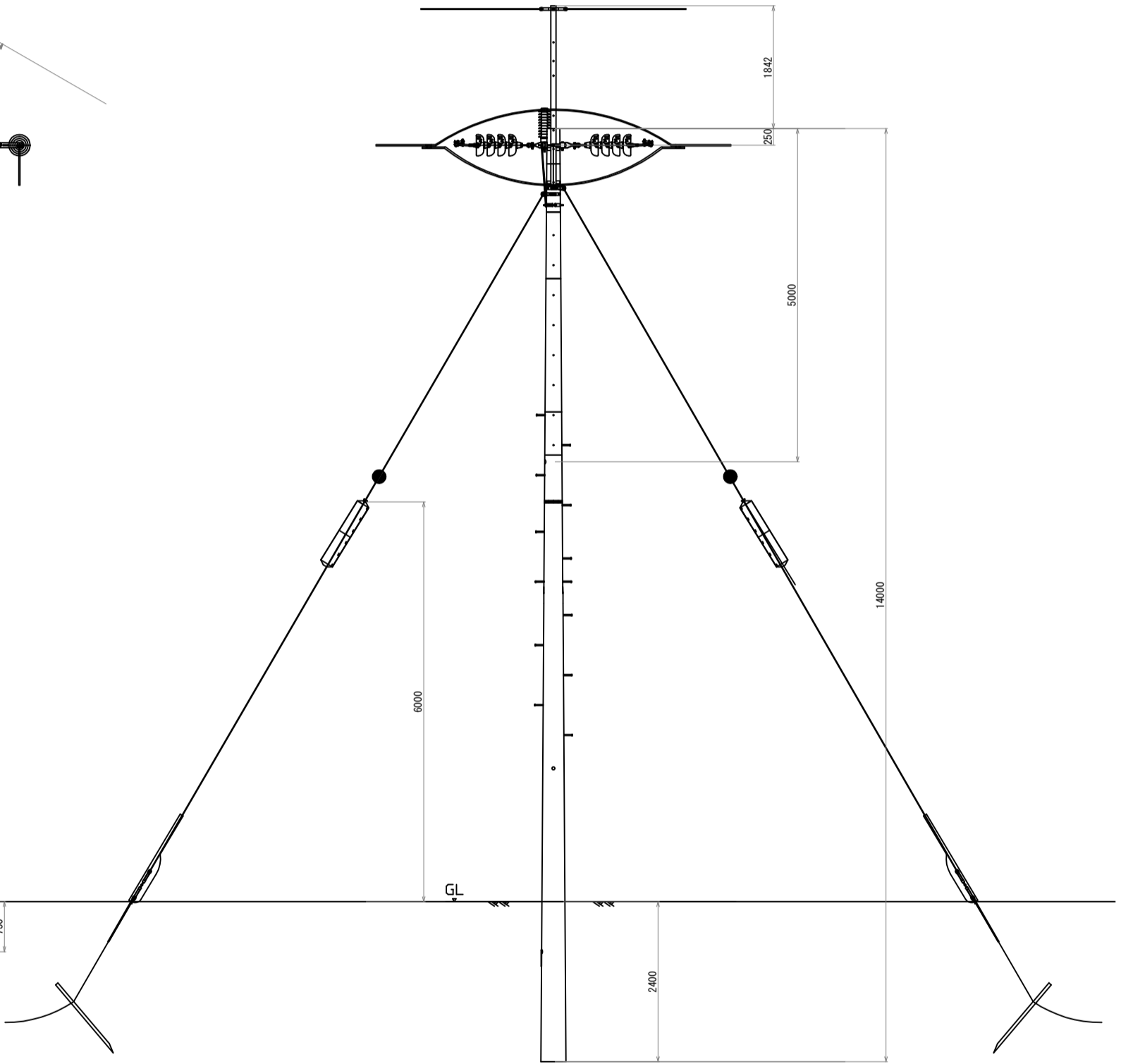
14m Pole Type C
