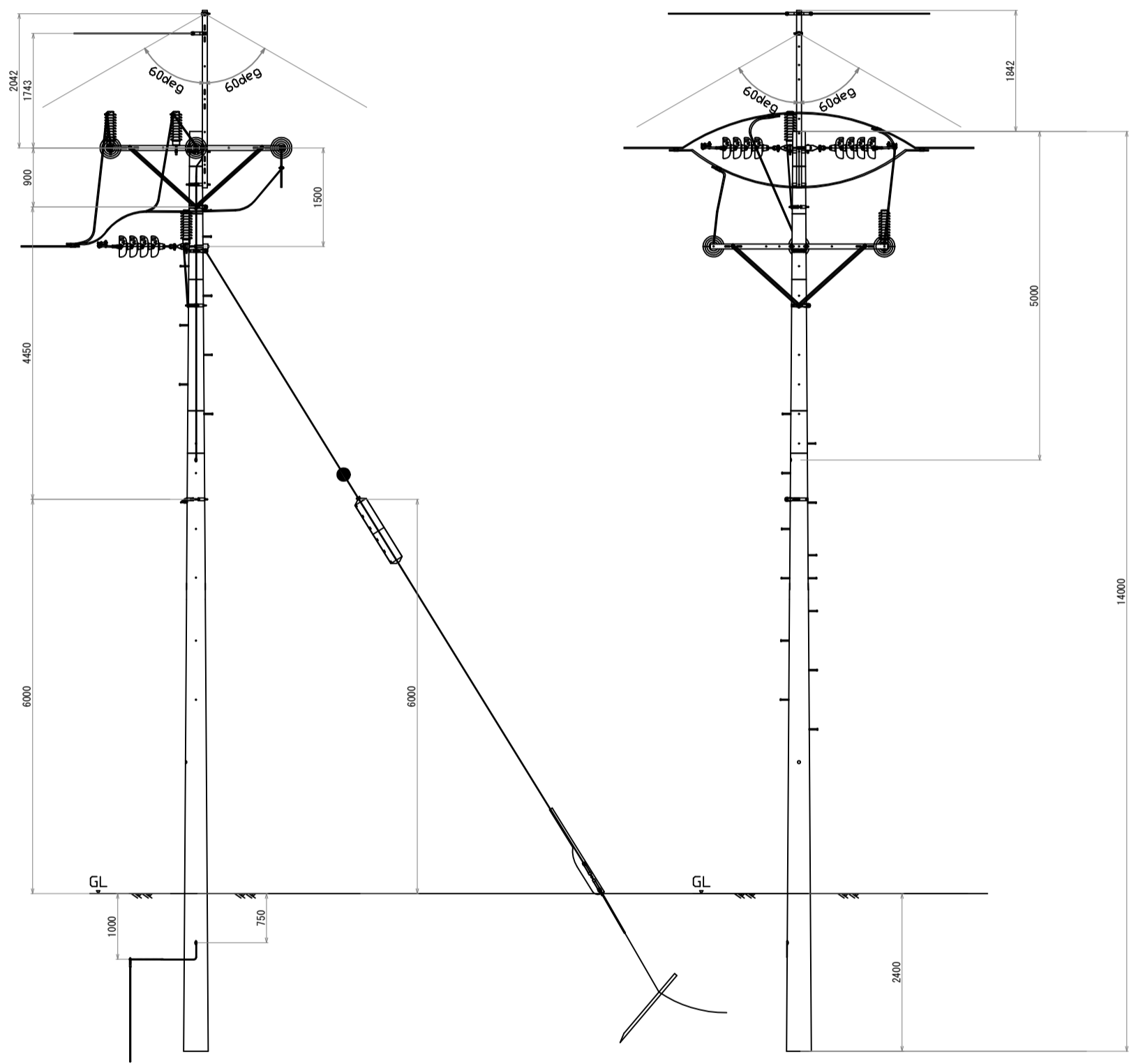
14m Pole Type E
