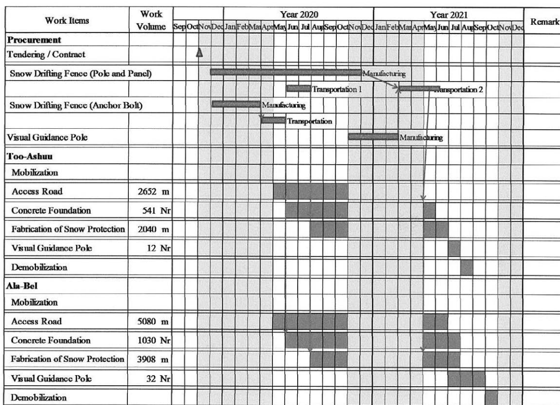
Figure 5-1 Construction Schedule
