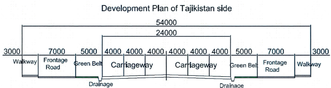
Figure-2 Cross section of road specified in the Master Plan
