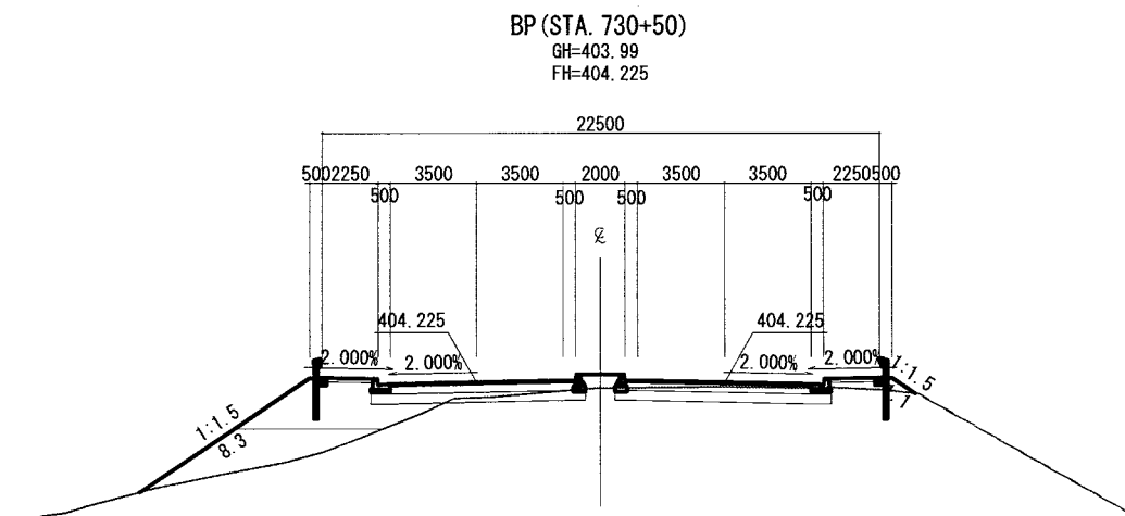
Figure-1 Cross Section at STA.730+50
