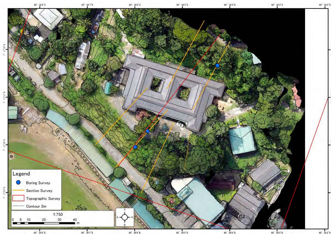
Figure 2.1 Investigation Plan for Kandy Nursing School Site
