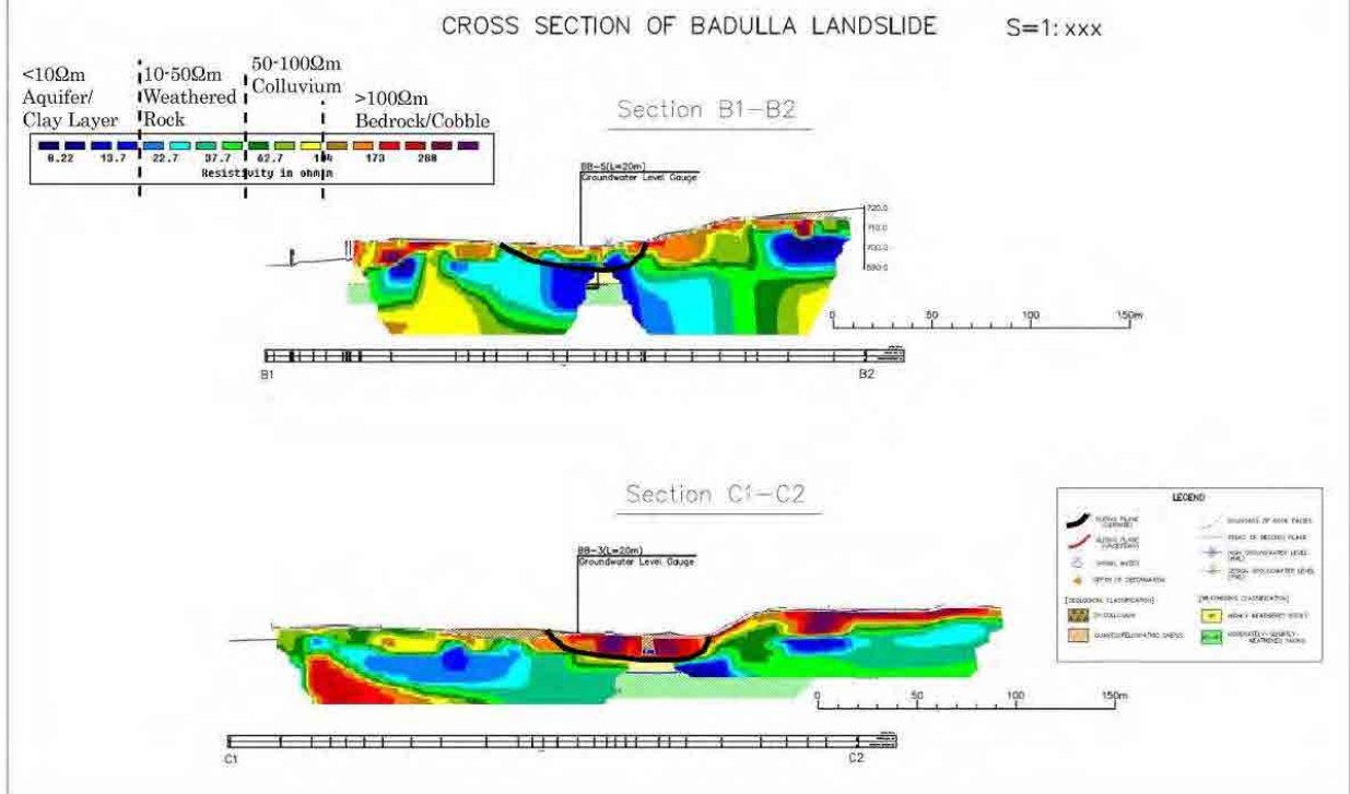
Figure 3.9 Result of Resistivity Survey of Badulusirigama Landslide (2)
