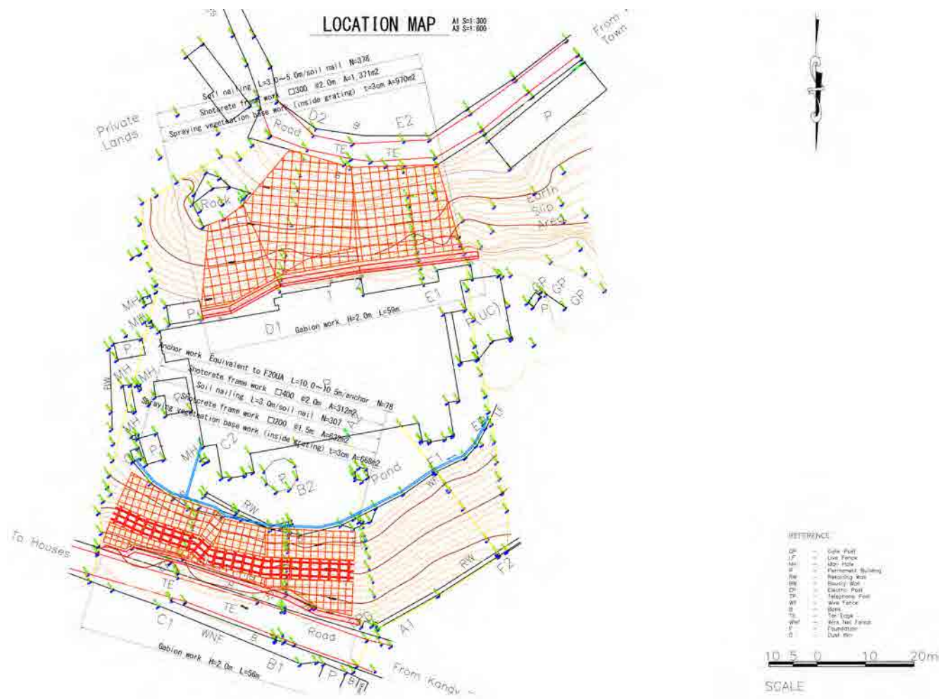
Figure 5.1 Plan of Basic Design of Countermeasures against Kandy Nursing School site
