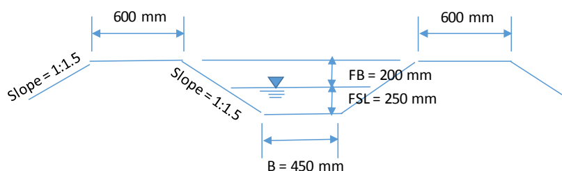
Typical Cross Section of Canal (Type 1)
