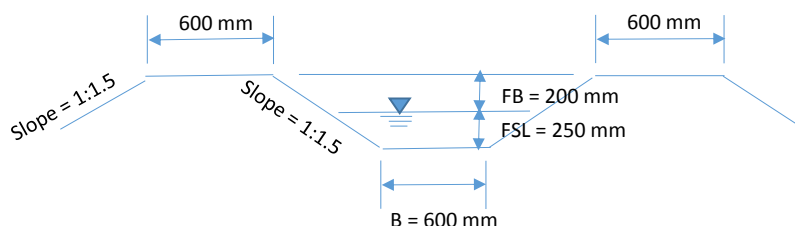
Typical Cross Section of Canal (Type 3)
