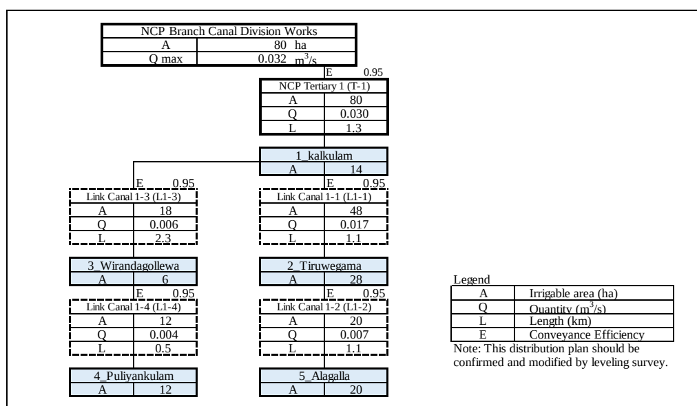
Distribution Diagram of Alagalla Cascade
