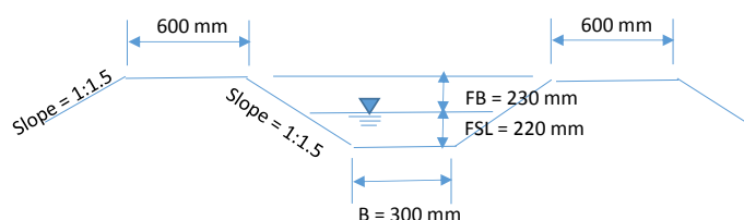
Typical Cross Section of Canal (Type 1)
