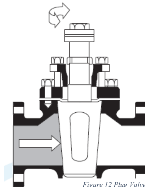
Figure 12 Plug Valves
