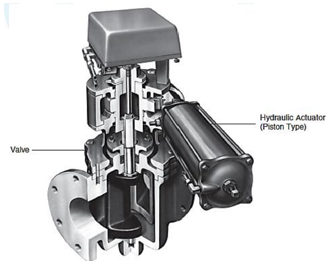
Figure 3 Eccentric plug valve with hydraulic actuator
