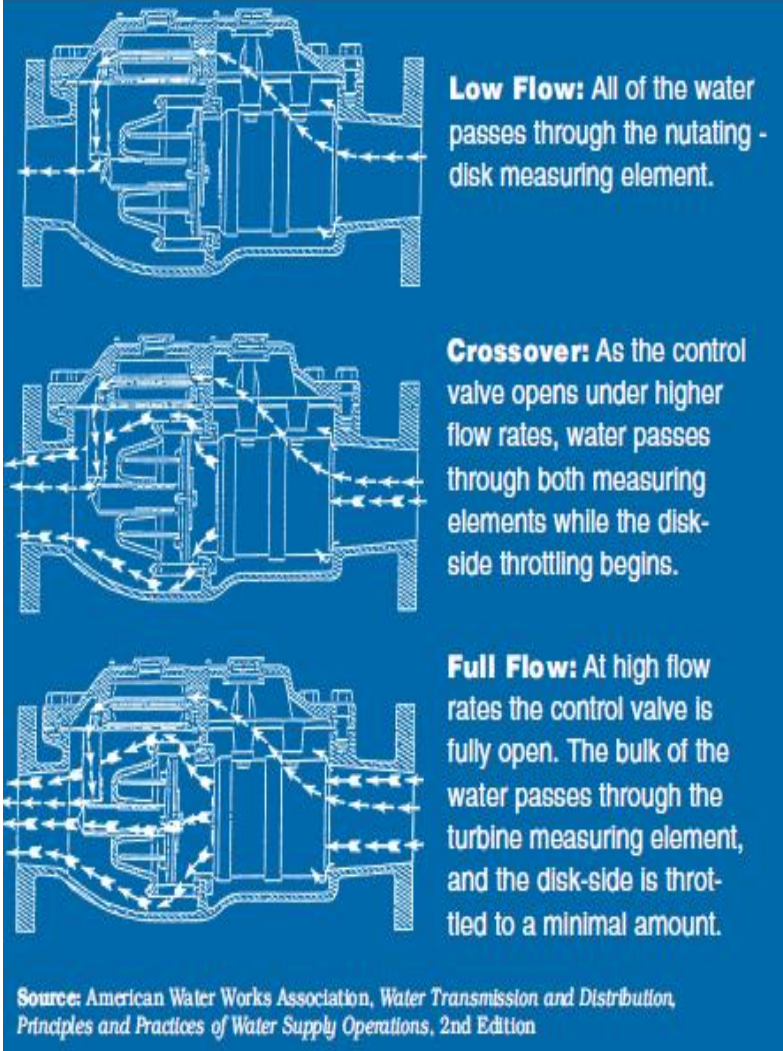
Figure 2 - Compound Meter
