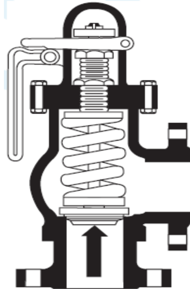
Figure 9 Pressure release valve
