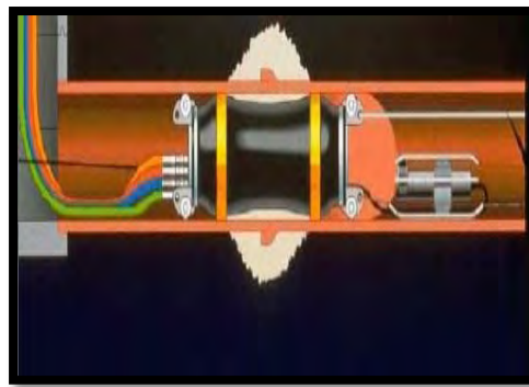
Figure 10: Internal Grouting
