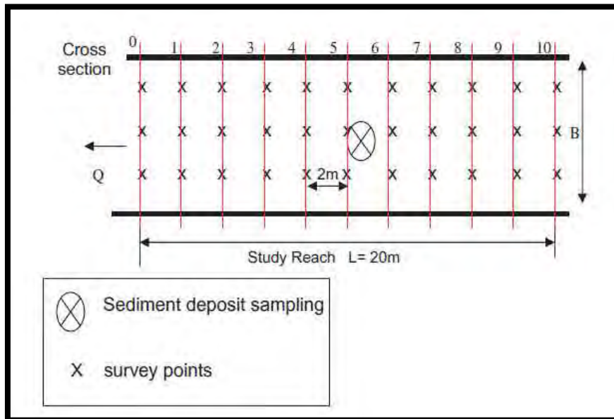
Figure 3: Measurement points at a station
