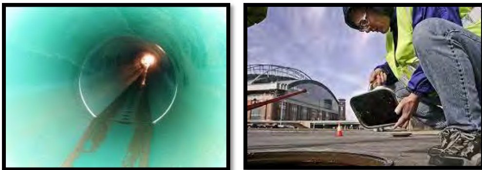
Figure 4: Lamping Test Operation
