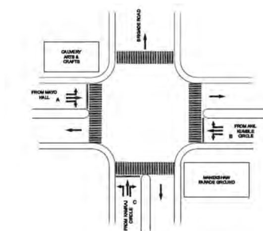
Figure 5: Details of Cauvery Arts & Craft Intersection
