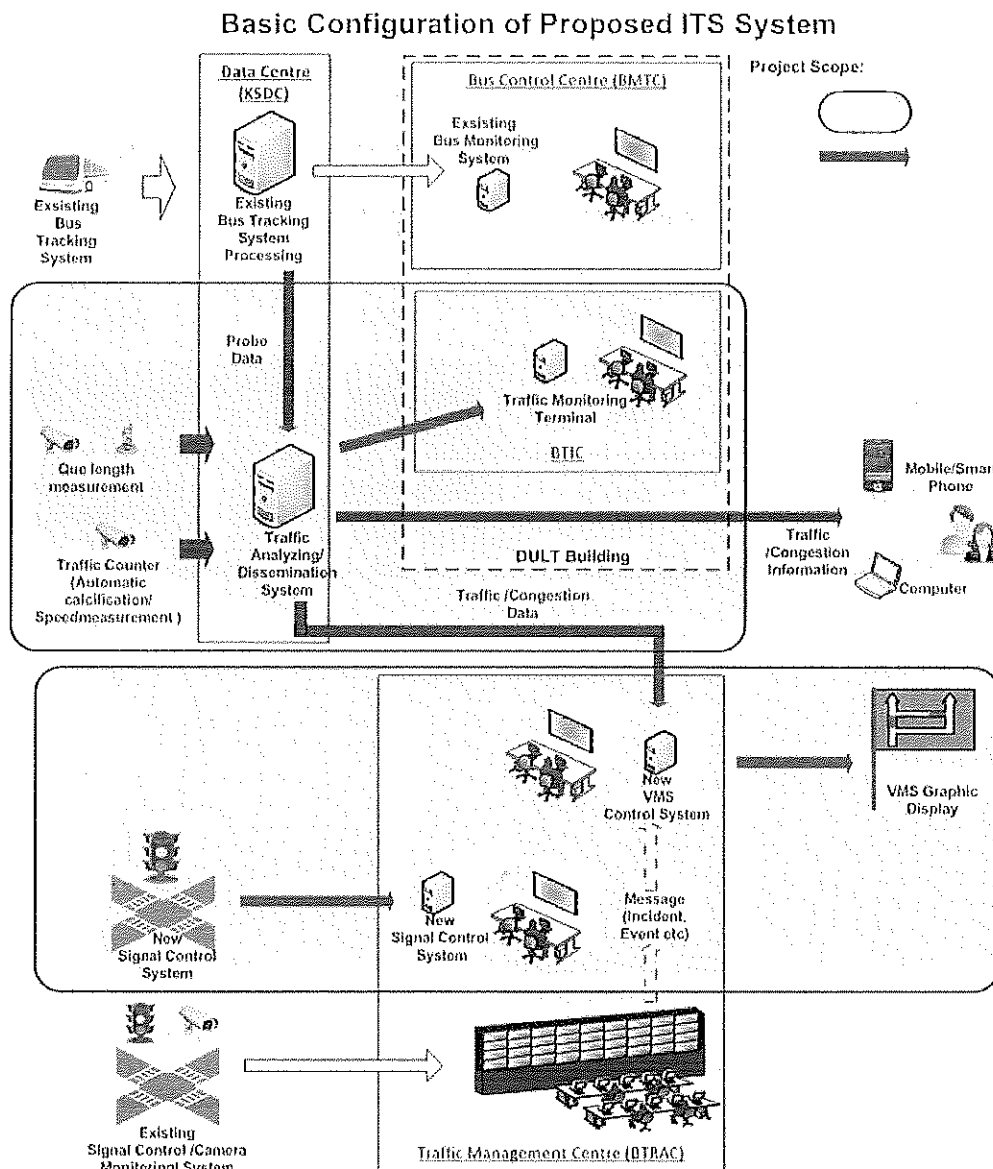
Figure 2-8 Basic Configuration of B-TIC
