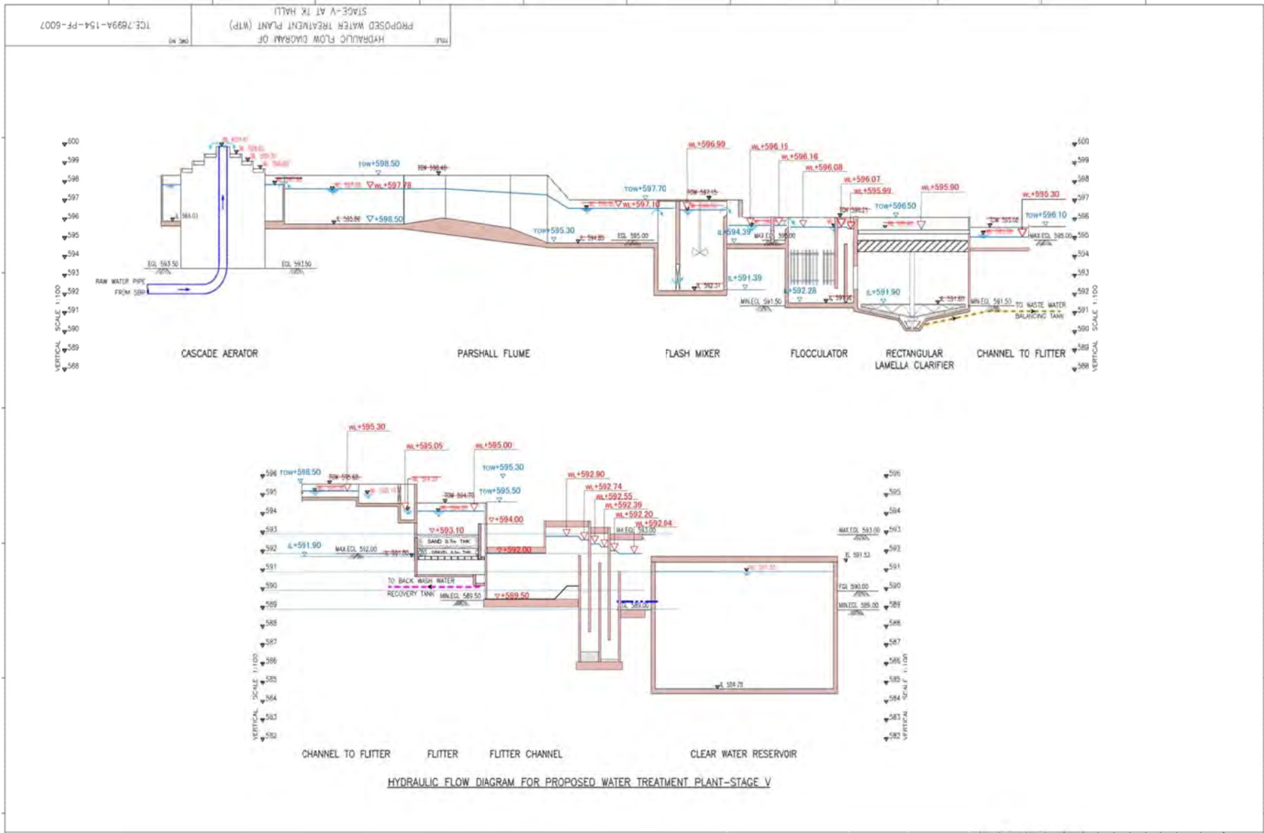
Figure 12.1.9 Hydraulic Profile
