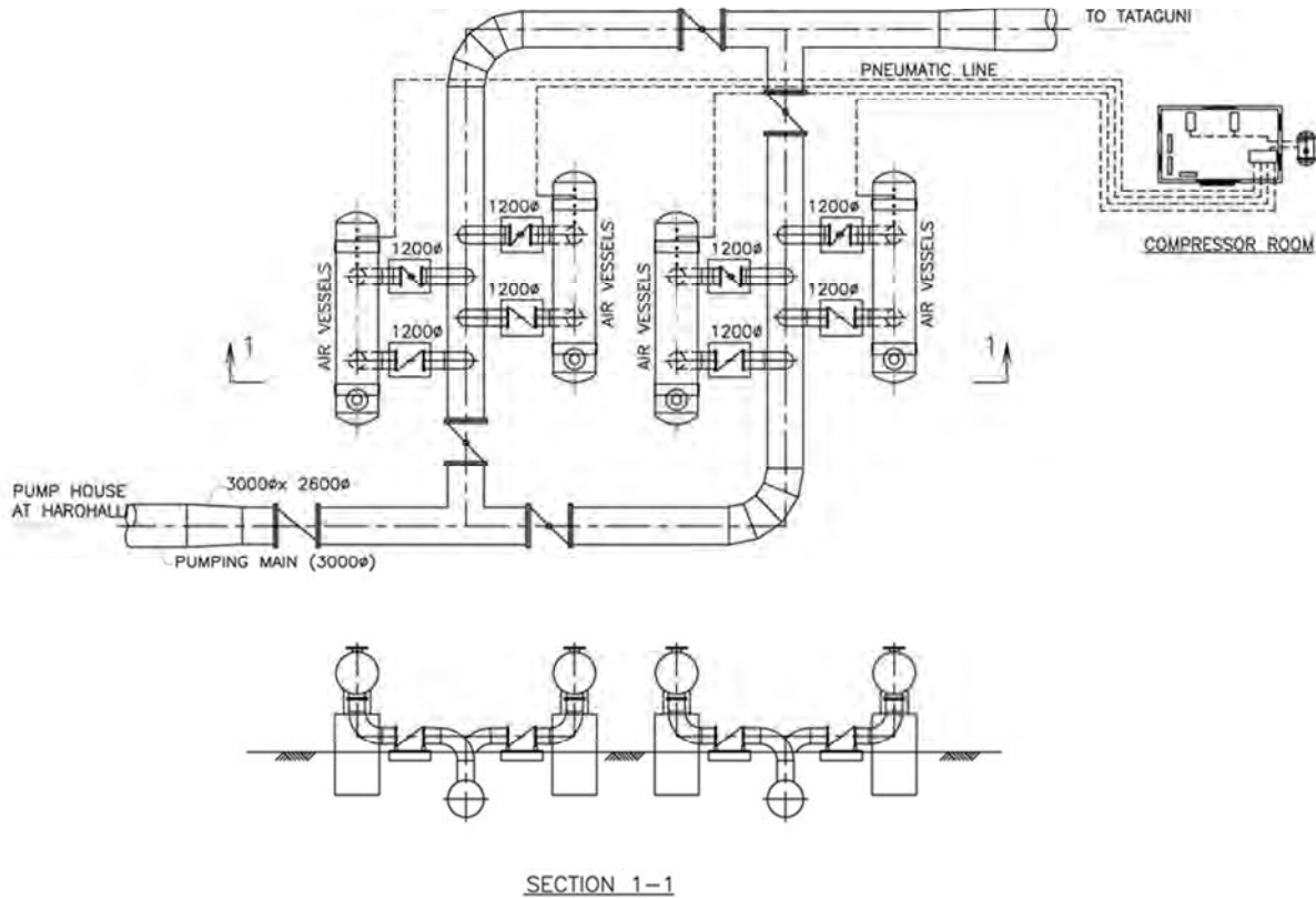
Figure 12.1.14 Typical Air Vessels
