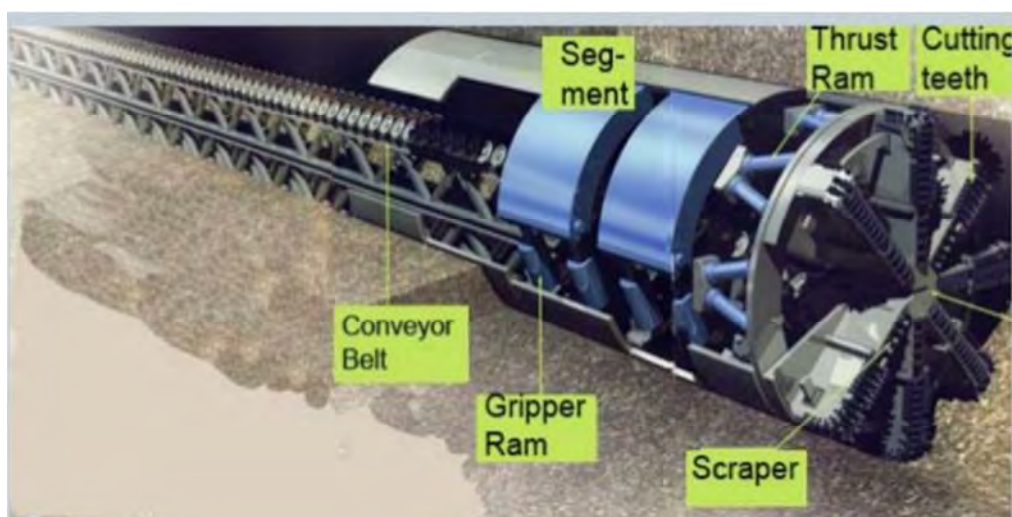
Figure 12.2.6 Tunneling Method
