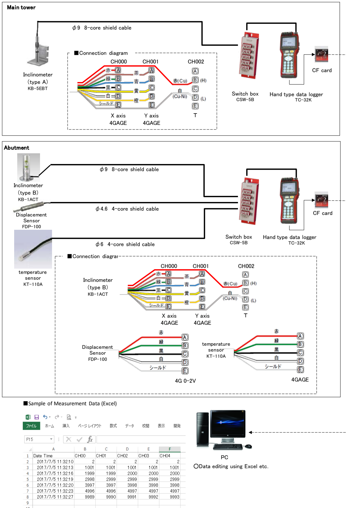
Figure-2: Measurement System Diagram
