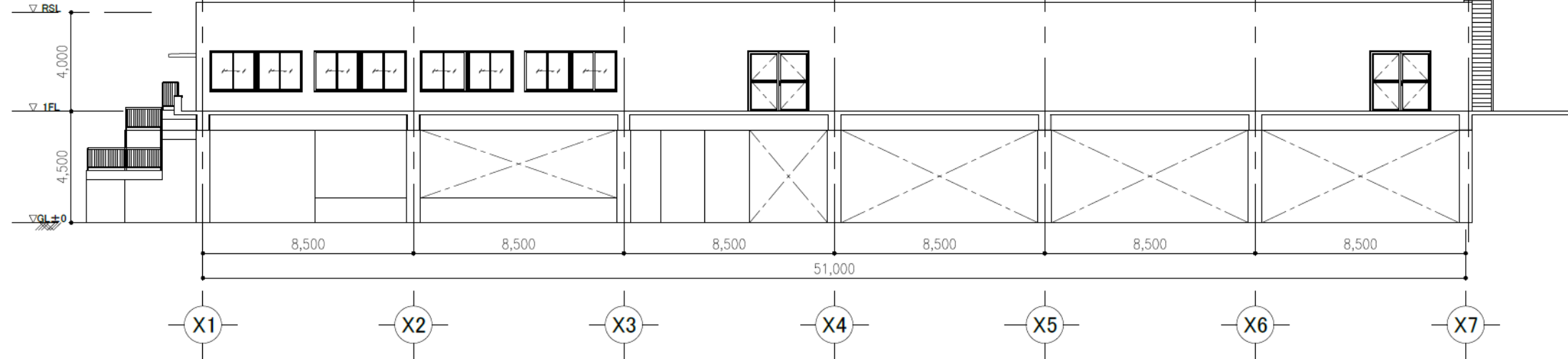
SOUTH ELEVATION
