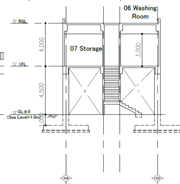
B-B' SECTION
