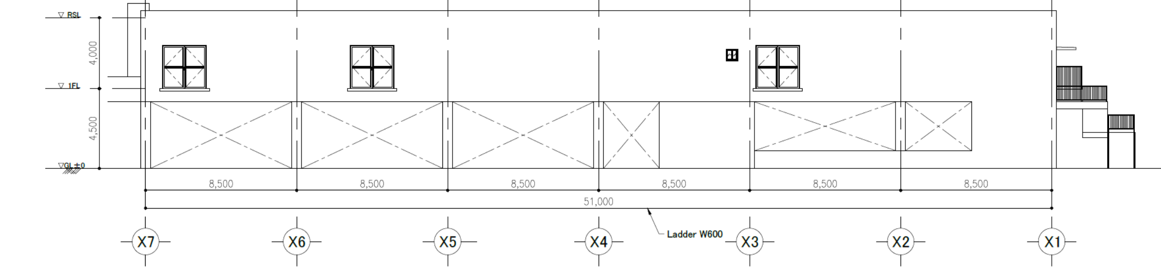
NORTH ELEVATION
