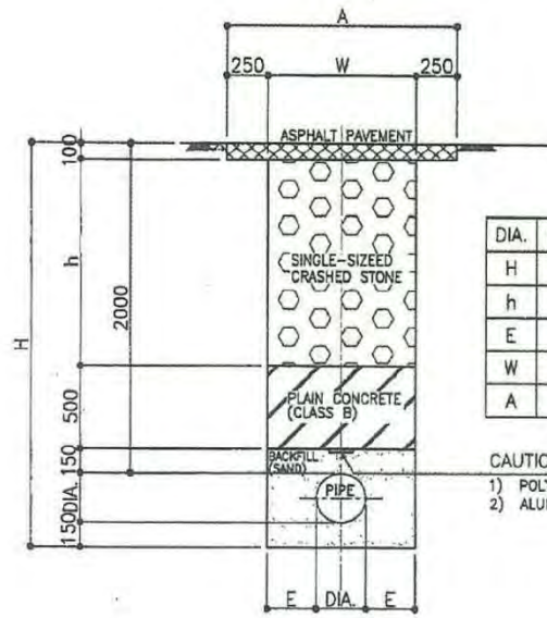
ROAD ALONG PAVEMENT FOR NATIONAL ROAD AND MAIN ROAD
