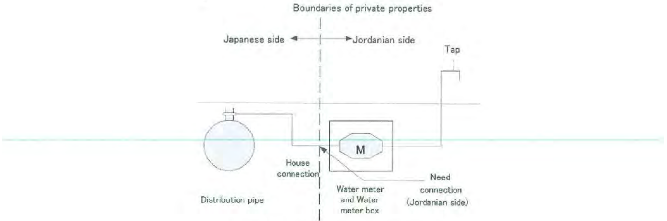
Figure 4.2 Boundary of Service Pipes Laying
