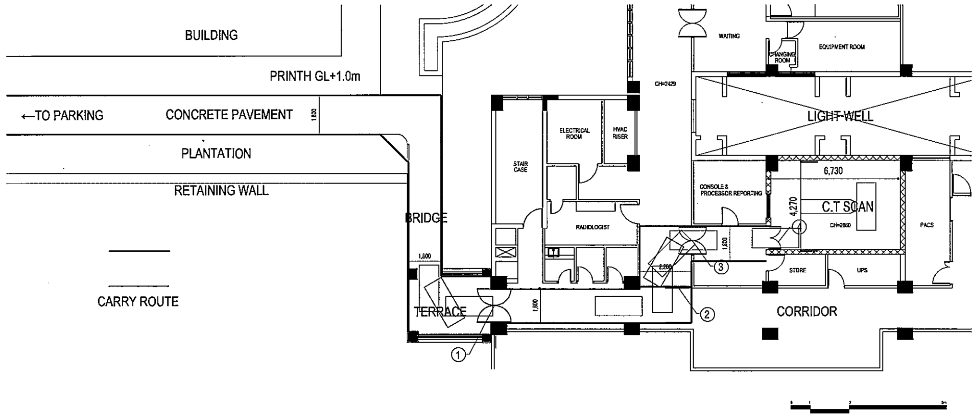
RENOVATION WORKS (EXPANSION OF DOOR OPENING)
