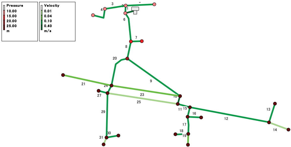
Kapala RGC : Pressure and Velocity ( Pipe Number )
