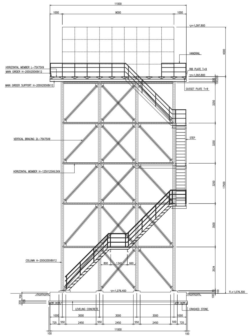
SECTION B-B
