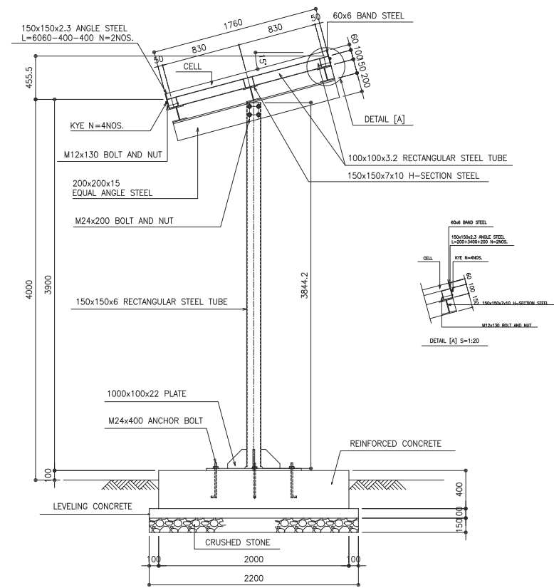
SECTION B-B
