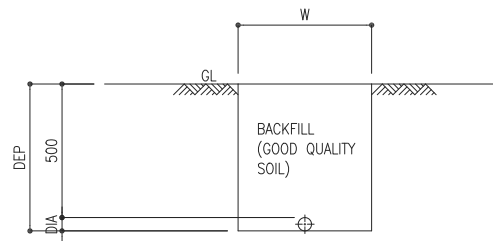
SERVICE PIPE INSTALLATION
