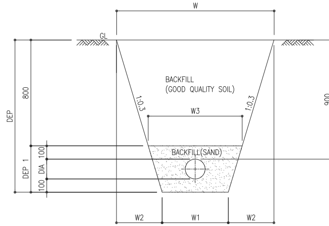
PIPE INSTALLATION
