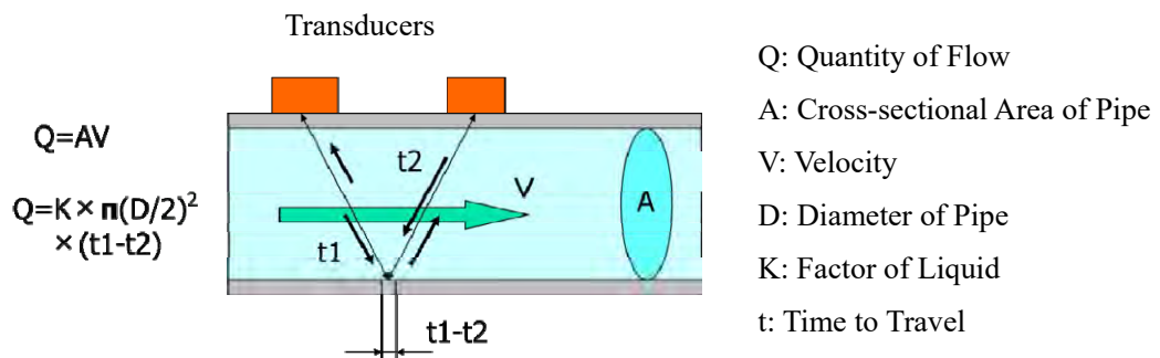
Figure 1-1 Principle of the Ultrasonic Flow Meter
