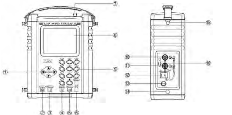
Figure 2-9 Main unit of Leak Noise Correlator
