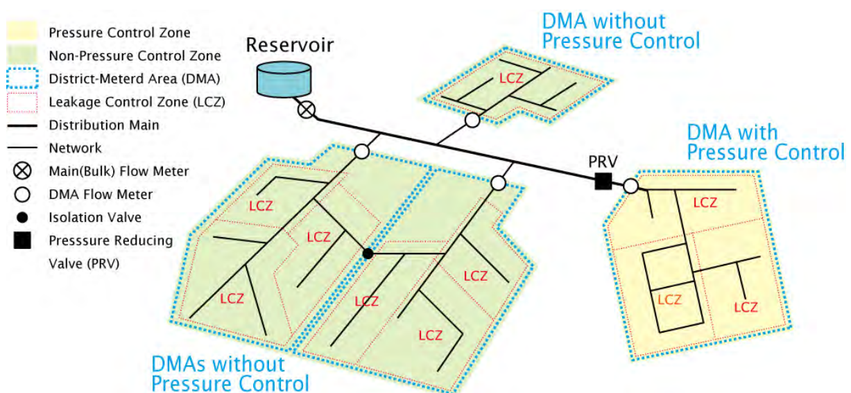
Figure 2.1 Conceptual Drawing of DMA, LCZ and Pressure Control Zone (PCZ) /Non-PCZ
