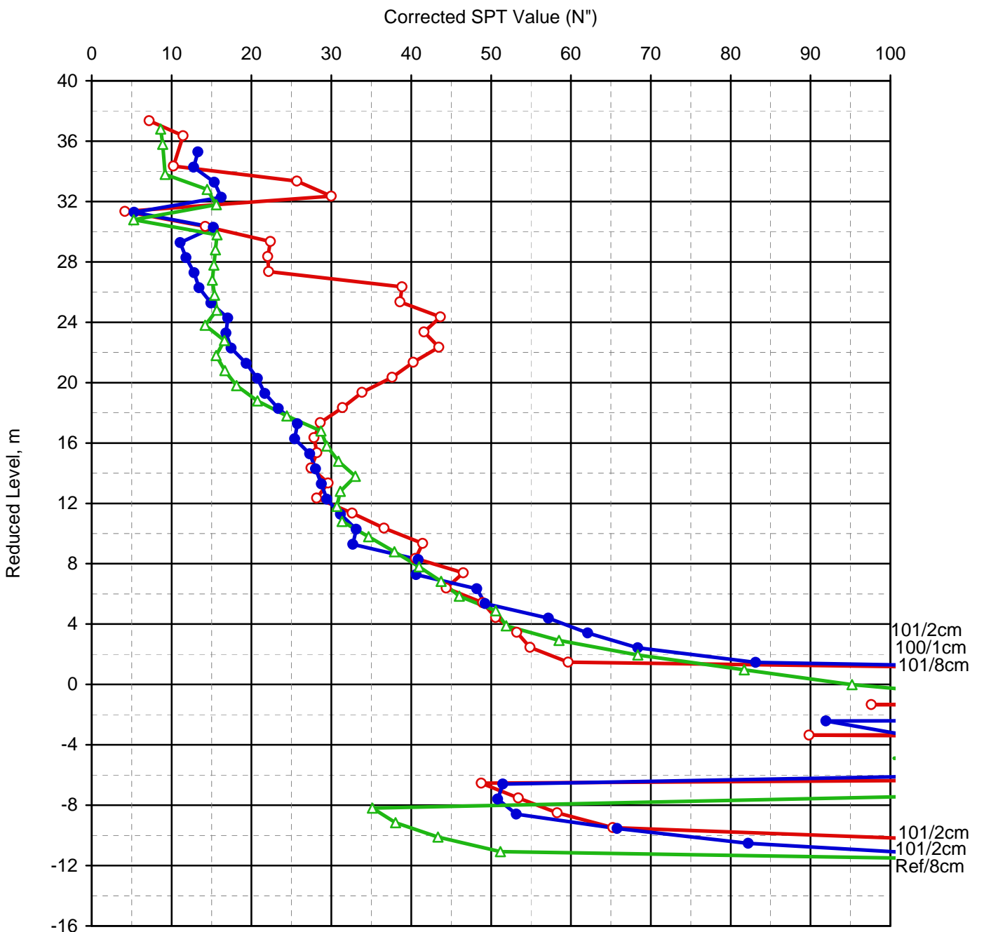
Corrected SPT Values versus Reduced Level
