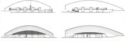
CUT DOME SHELTER SECTION, ELEVATION
