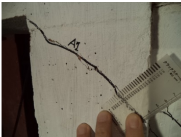
Diagonal crack width of left column is 0.3mm, right column is 0.1mm shear crack of column
