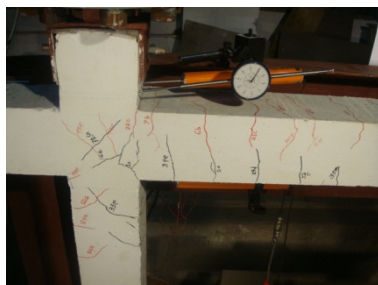
Flexural crack on beam, shear crack at panel area
