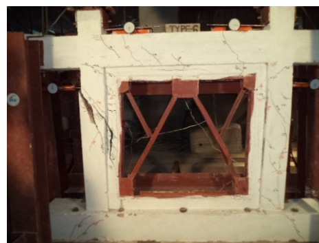
Failure at deflection 20.9mm
