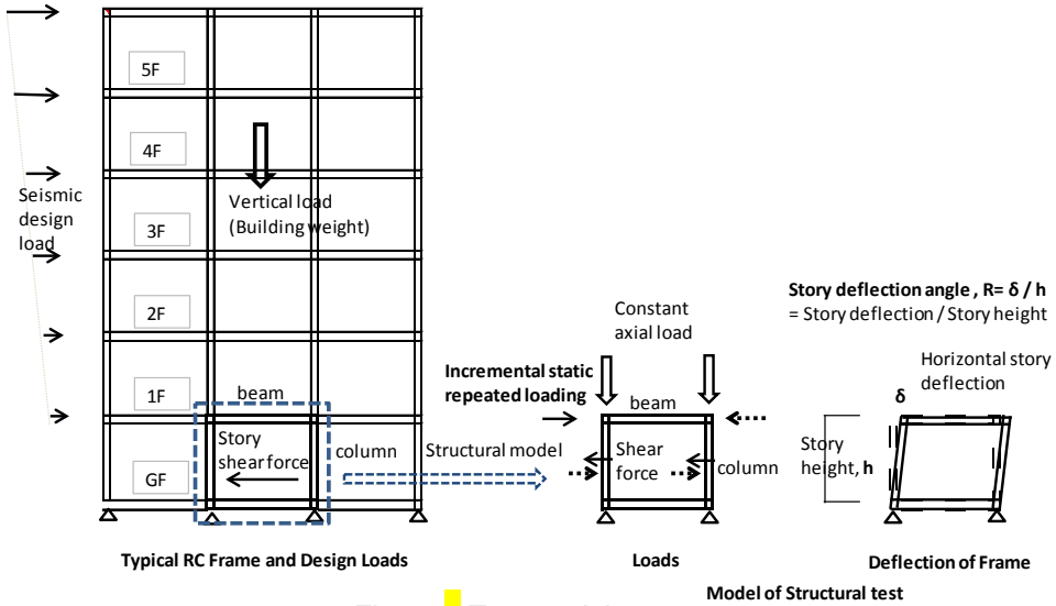
Figure 1 Test model
