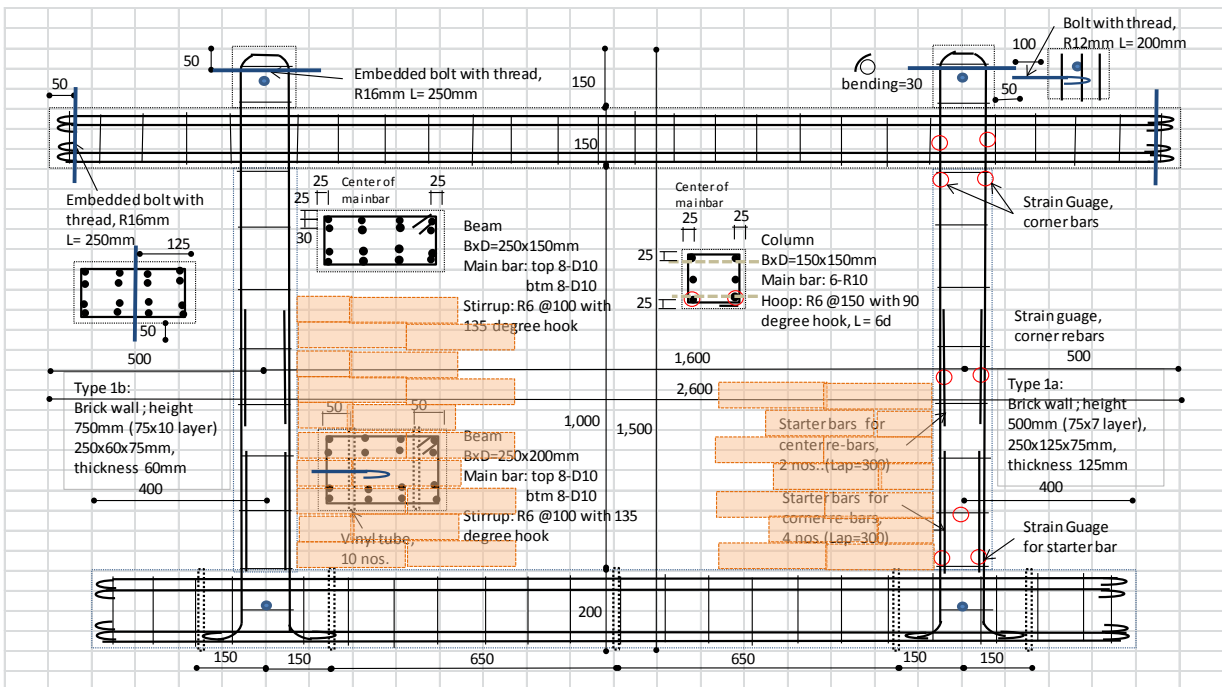
Type 1a & 1b (Strong beam, plain bar and brick wall) x 1 each (total 2)
