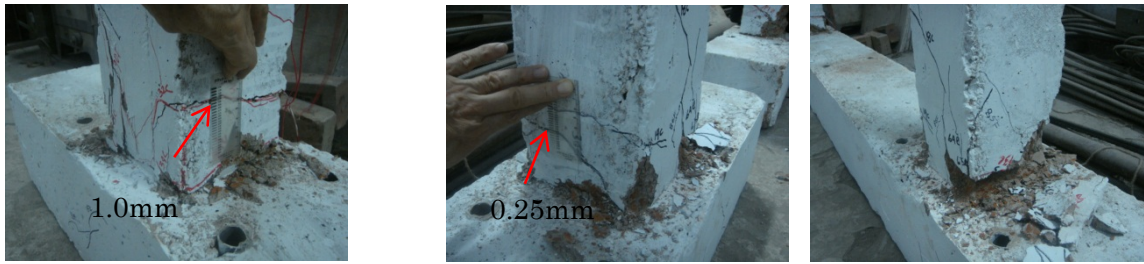
Left column, flexural crack 1.0mm Right column, flexural crack 0.25mm and compressive failure
