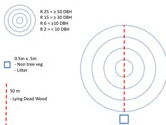
Figure: Location and layout of subplot carbon pool sampling areas.
