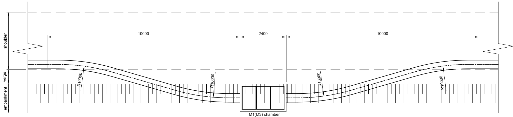
CHAMBER FOR COMMUNICATION DUCT ON ROAD scale: 1/100
