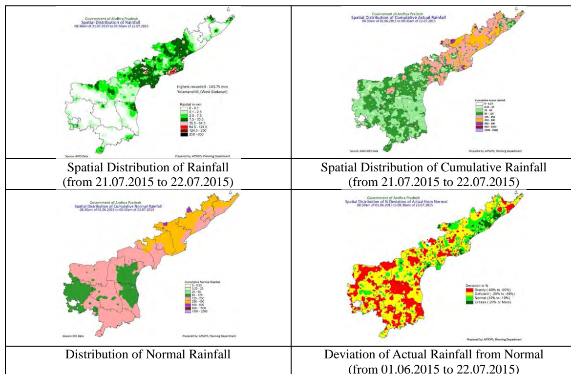
Figure 7.4.5 Example of Daily Spatial Maps by APSDPS
