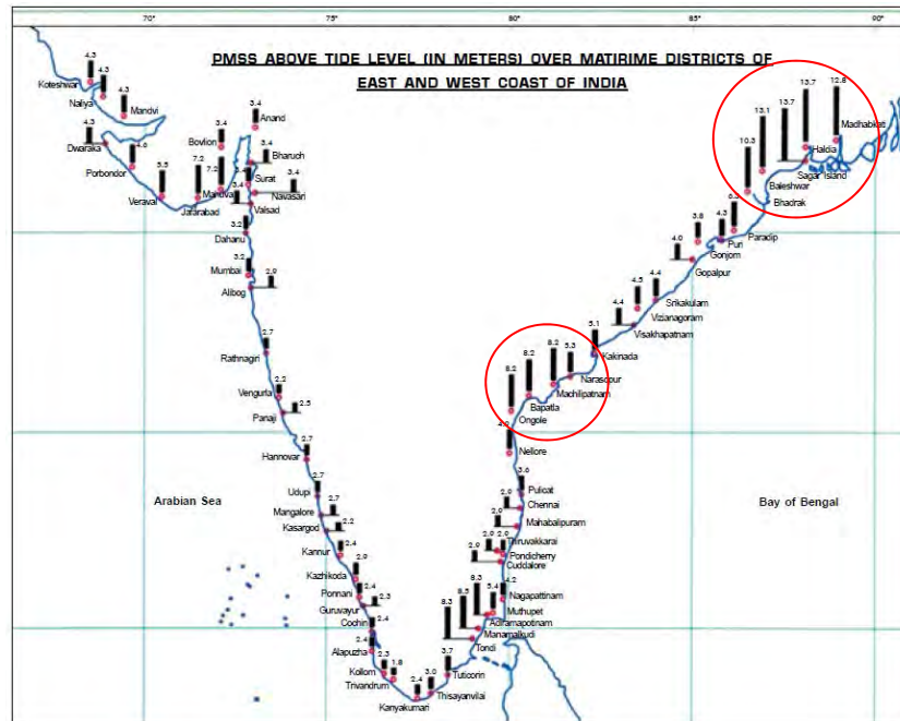
Source: compiled by the Survey Team based on “Cyclone Warning in India Standard Operation Procedure”, (2013) of the IMD
