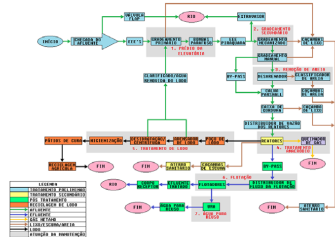
Image 3 - Operational Flowchart of Atuba Sul WWTP
