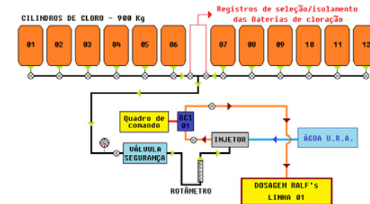
Image 41 - Chlorination flowchart
