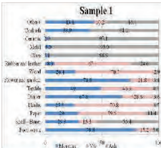
Figure 4a Correlation of moisture content, VS and ash (% wet weight) of each composition in sample 1
