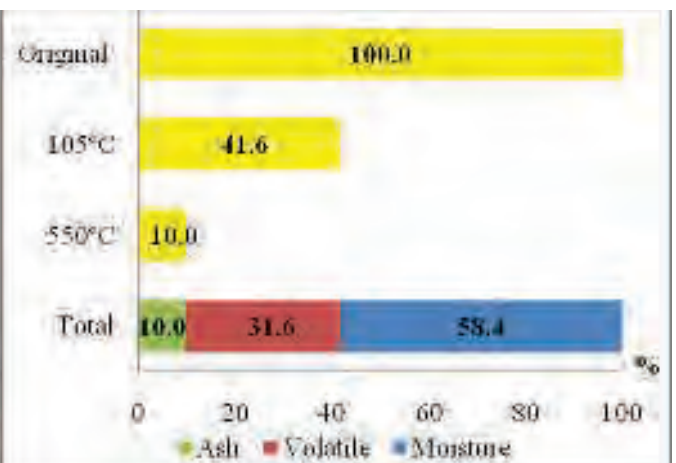
Figure 25 Correlation of moisture content, VS and ash values by wet weight in sample 2
