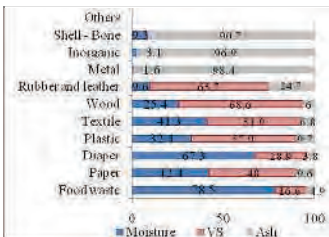
Figure 22 Correlation of moisture content, VS and ash of each physical composition in sample 3
