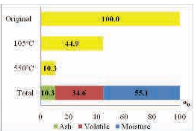
Figure 27 Correlation moisture content, VS and ash values by wet weight in sample 4
