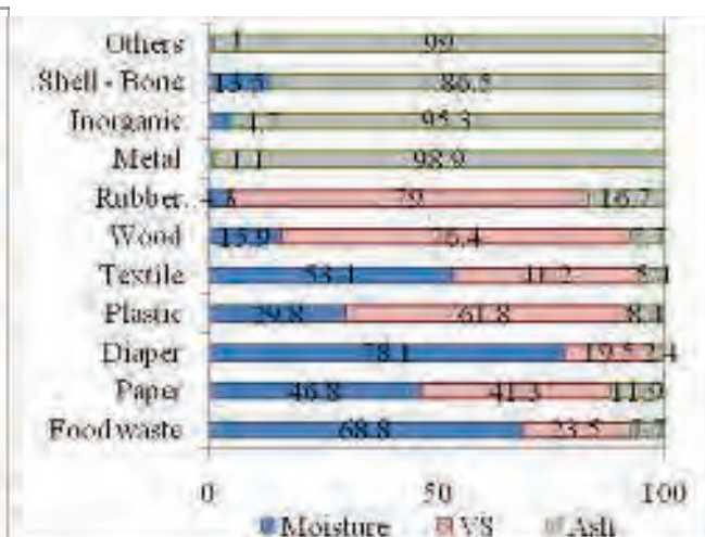
Figure 21 Correlation of moisture content, VS and ash of each physical composition in sample 2
