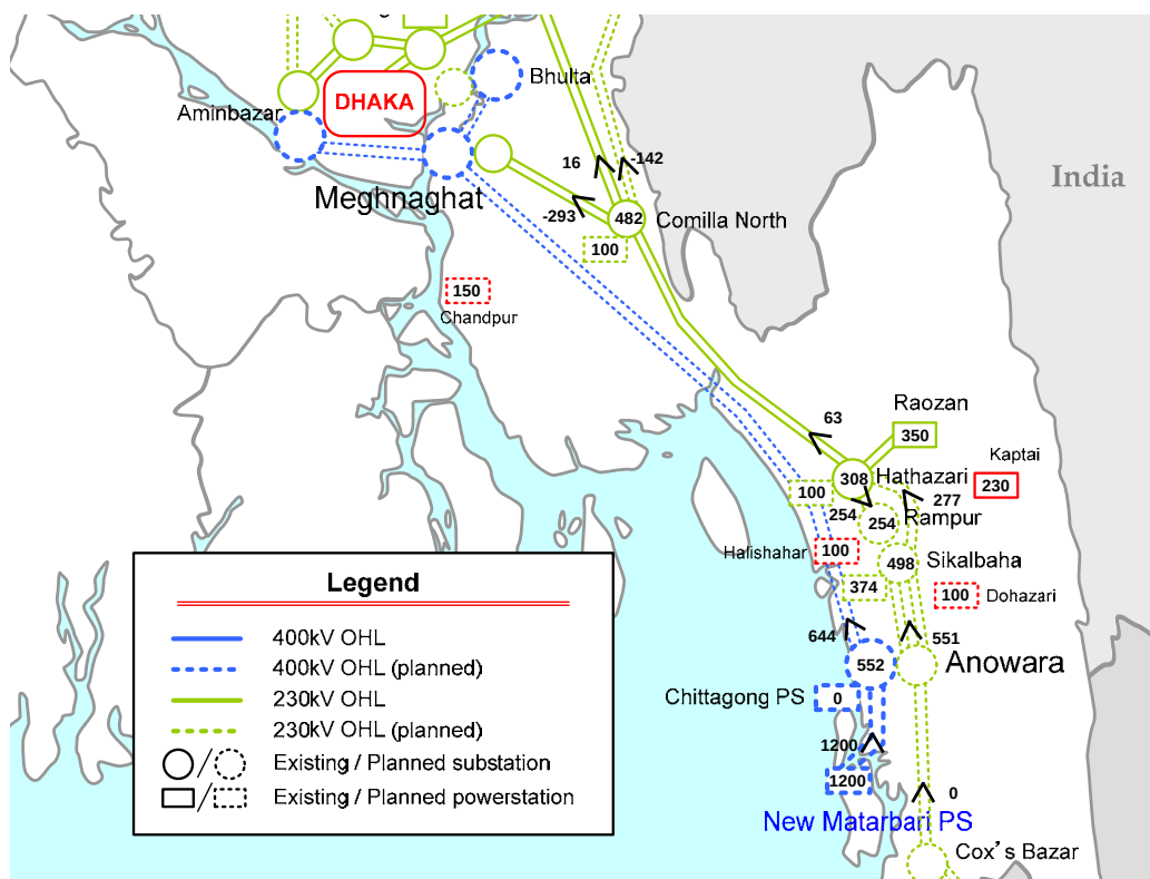
Figure 9.1-6 Power Flow Diagram of Pattern 2 (Mtbr: 1200, Chttgn: 0MW Peak)
