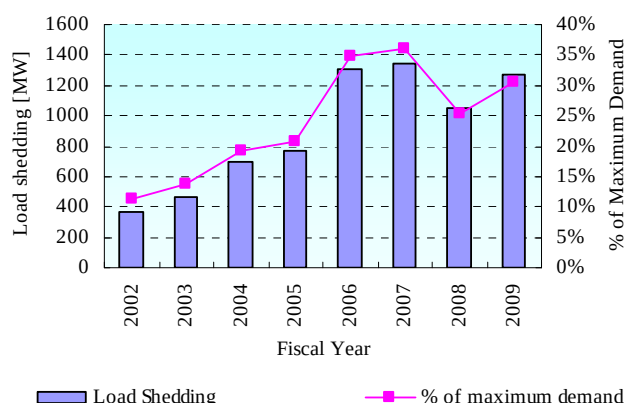
Figure 3.3-2 Annual Load Shedding/Restriction [MW]
