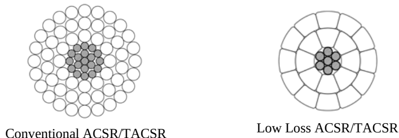
Figure 9.1-1 Configuration of Conventional and Low Loss Type ACSRs
