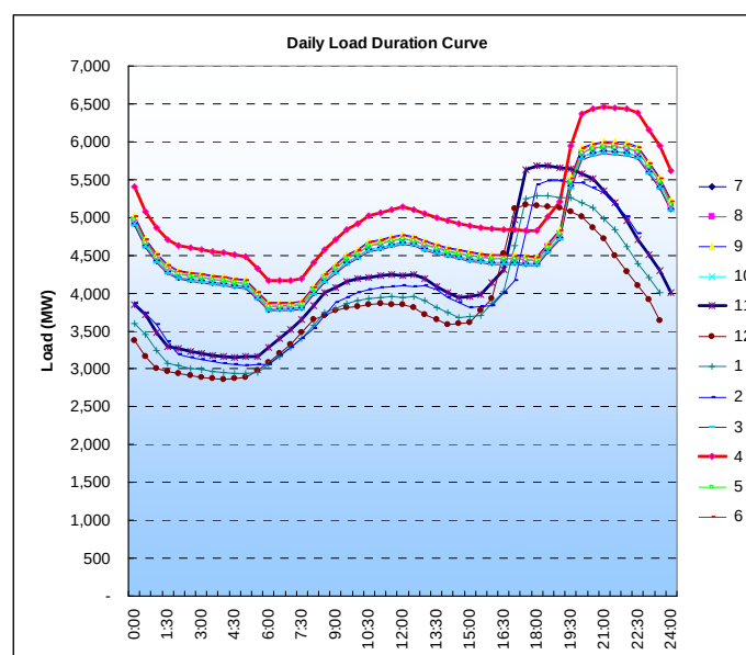
Figure 3.7-1 Daily Load Curve (2010)
