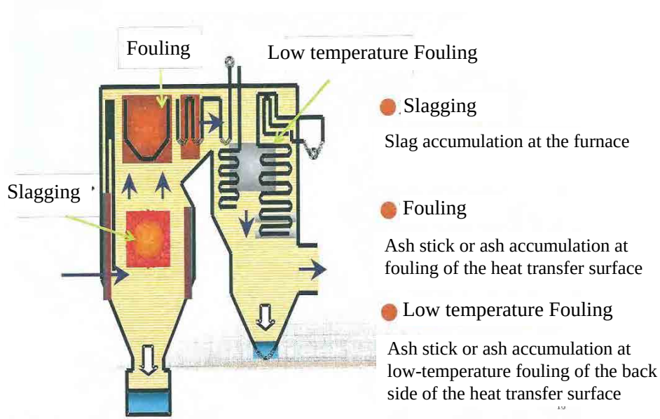
Figure 13.2-2 Ash Stain of Pulverize-coal-fired Boiler
