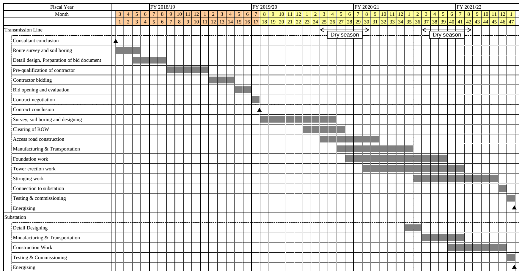
Figure 10.4-1 Assumed Implementation Schedule for the Transmission Line and Substation Construction
