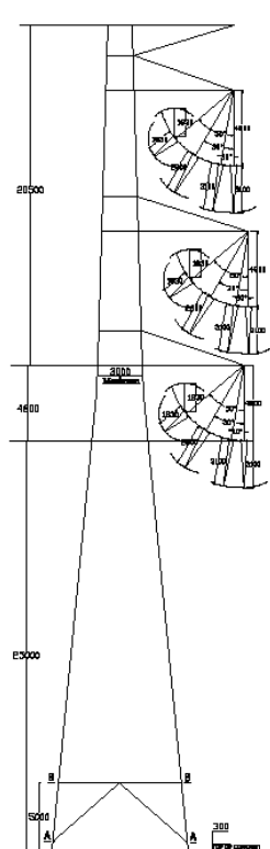
Figure 9.2-4 4DL Type Tower
