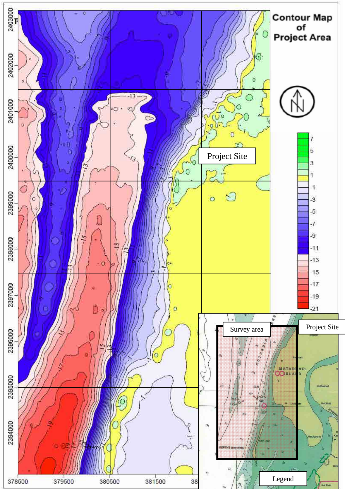
Figure 5.6-1 (2) Bathymetric Survey Map (Dry Season)
