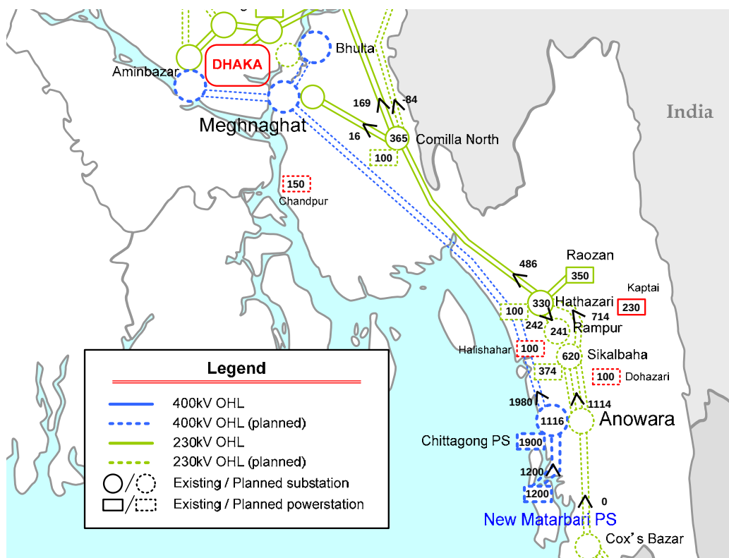
Figure 9.1-5 Power Flow Diagram of Pattern 1 (Mtbr: 1200, Chttgn: 1900MW Peak)
