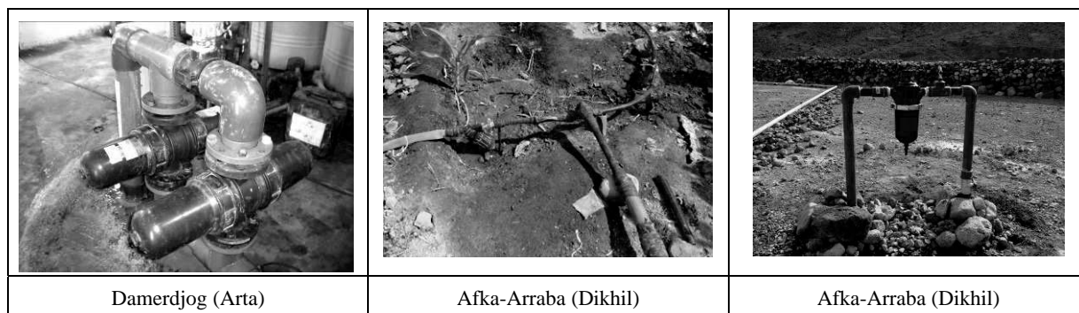
Figure 7.4.3 Case examples of the screen filter installed in Djibouti
