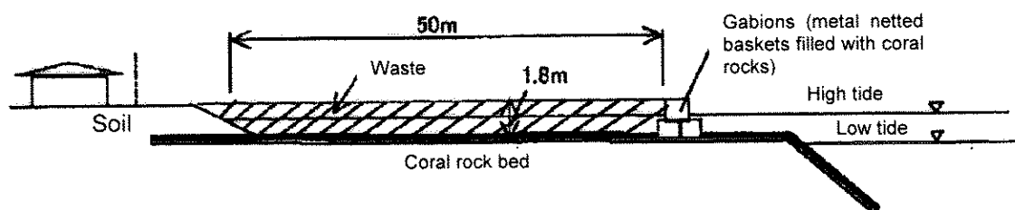
Figure 5-1 Cross-sectional View of Landfill Site
