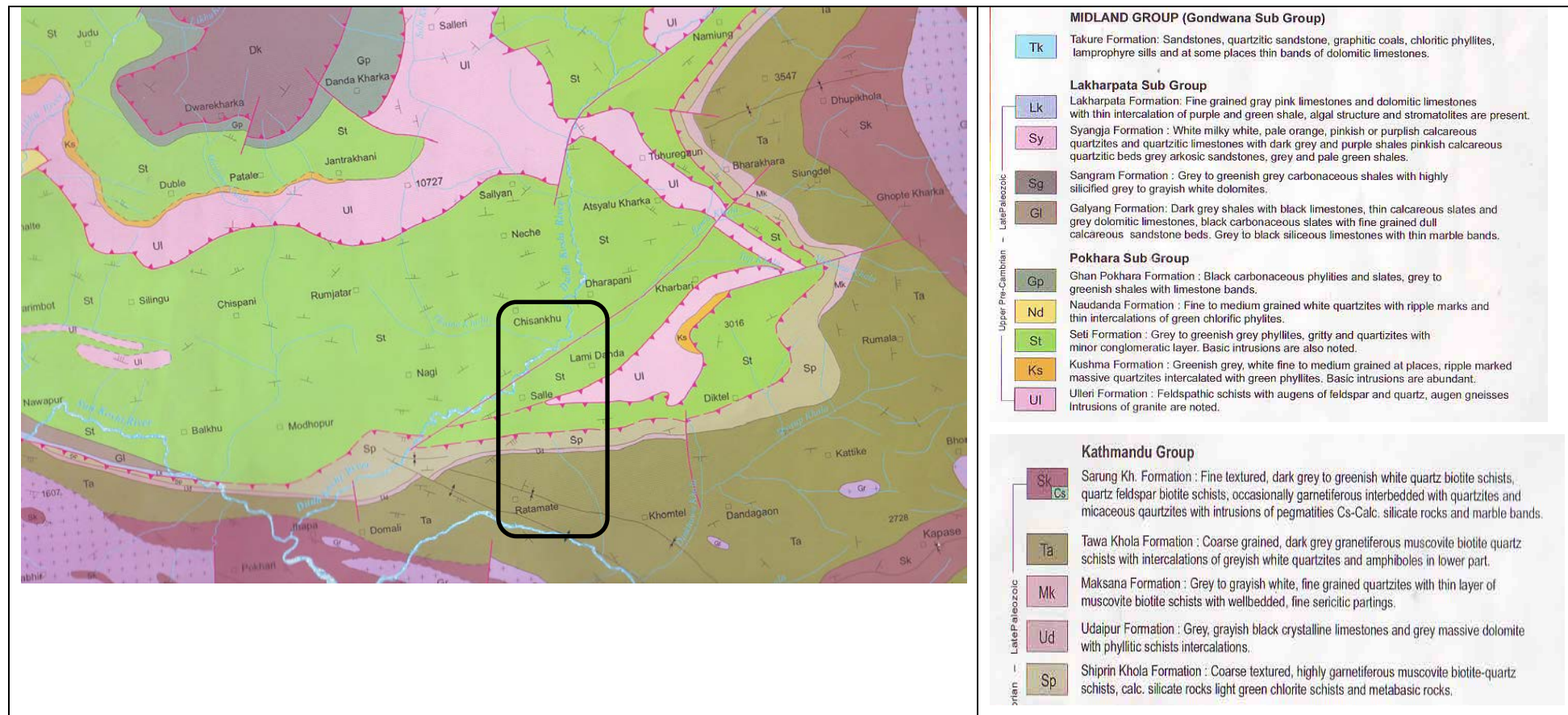
Figure 2.1: Regional Geological Map (DMG, 2011)
