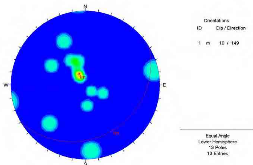
Figure 1.9: Stereographic projection of discontinuities at the dam axis around WPT 27. The major concentration represents foliation.
