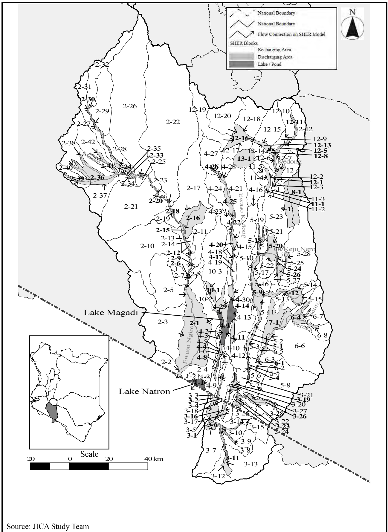
Figure 5.2.12 Surface Blocks of SHER Model RV-1
