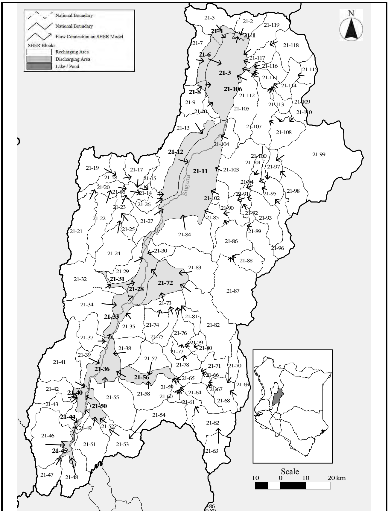
Figure 5.2.15 Surface Blocks of SHER Model RV-4
