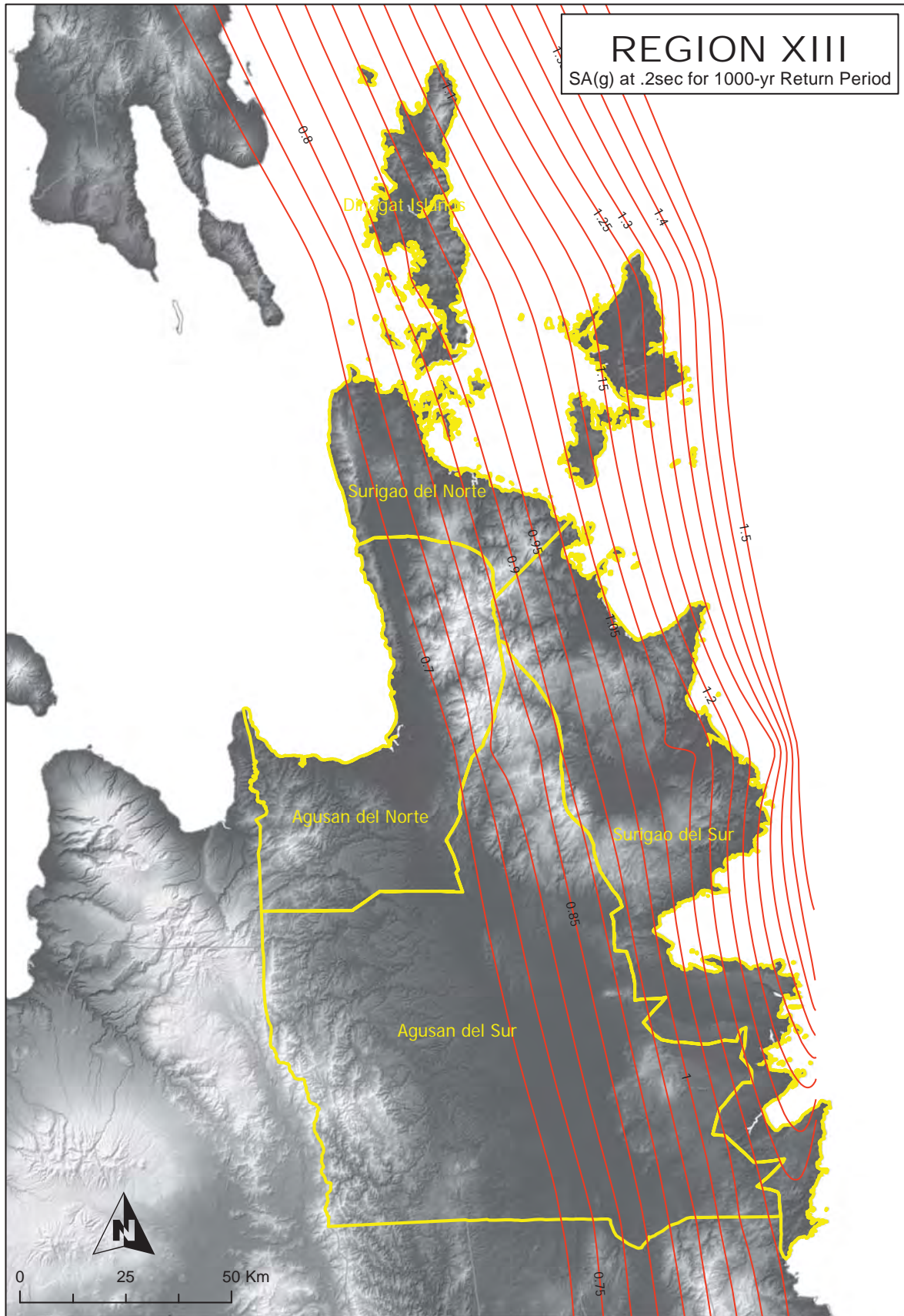
Figure 2A-49 Region XIII map of spectral acceleration at 0.2 sec. for 1,000-year return period
