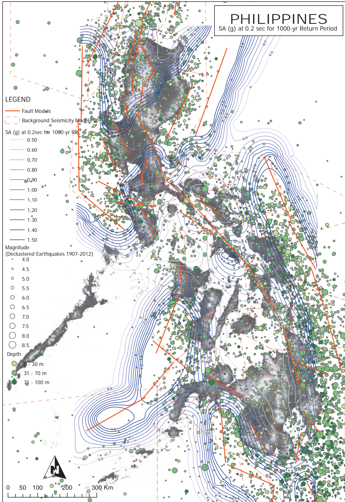
Figure 2A-5 Contoured result of S_a at 0.2 sec. for 1,000-year return period superimposed on seismic source models and declustered earthquake plots used in analysis
