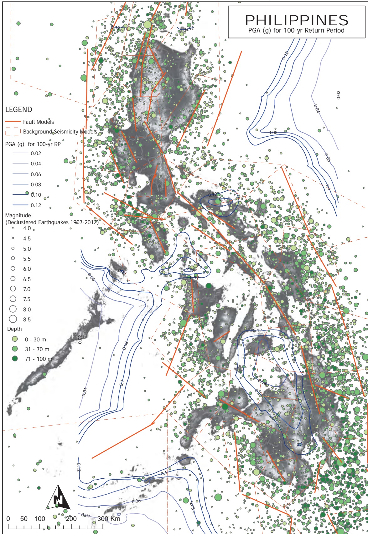
Figure 2A-10 Contoured result of PGA for 100-year return period superimposed on seismic source models and declustered earthquake plots used in analysis
