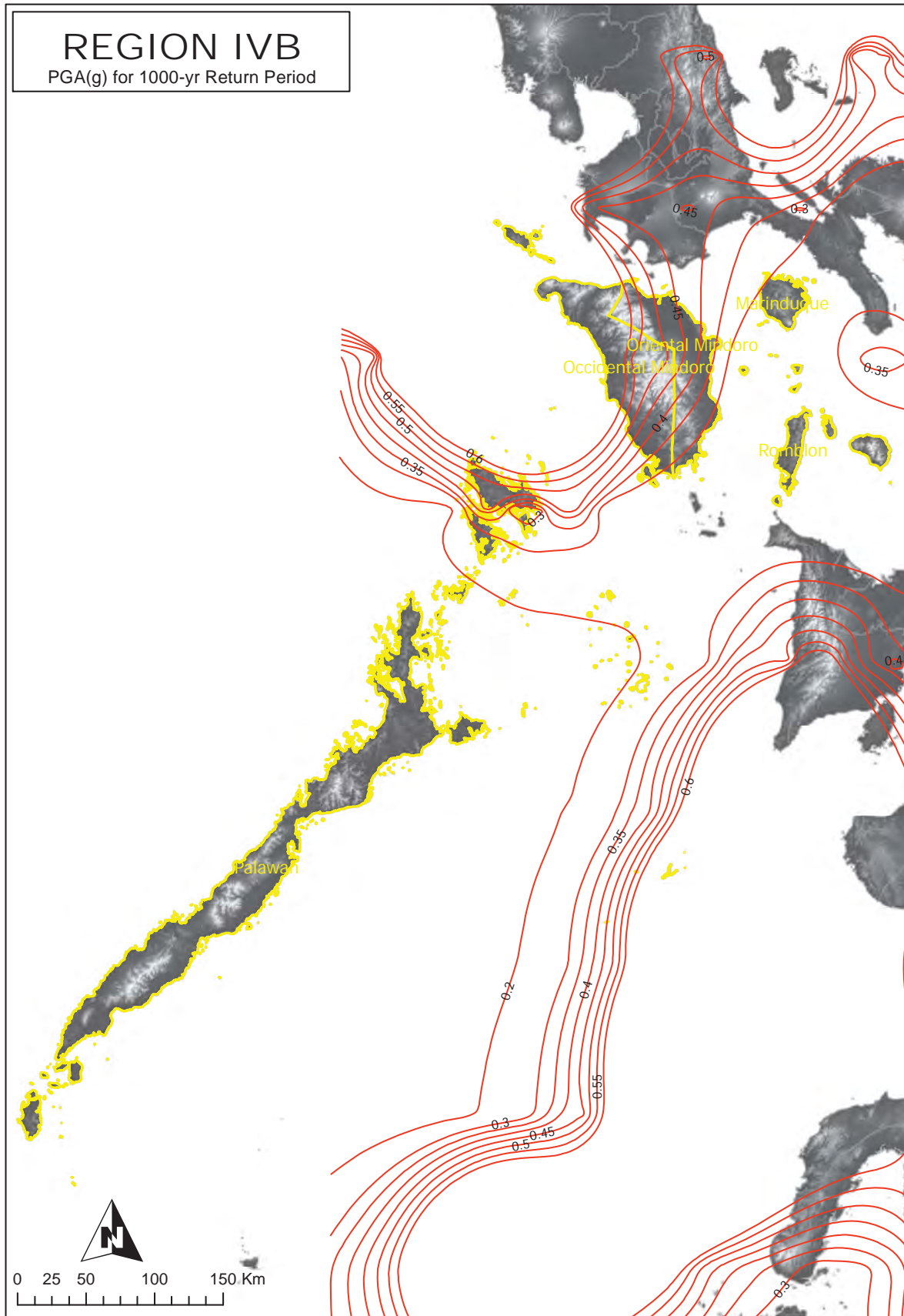
Figure 2A-24 Region IV-B map of peak ground acceleration for 1,000-year return period
