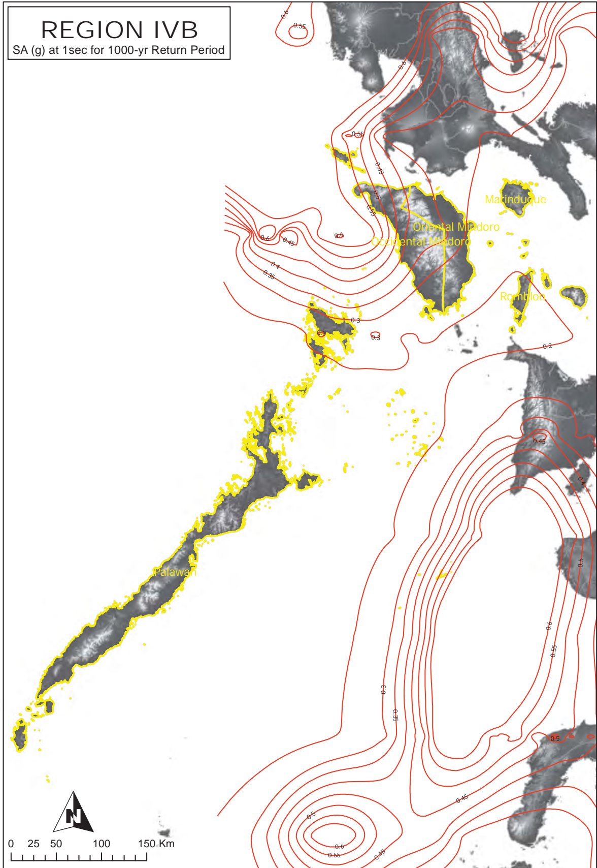
Figure 2A-60 Region IV-B map of spectral acceleration at 1. sec. for 1,000-year return period
