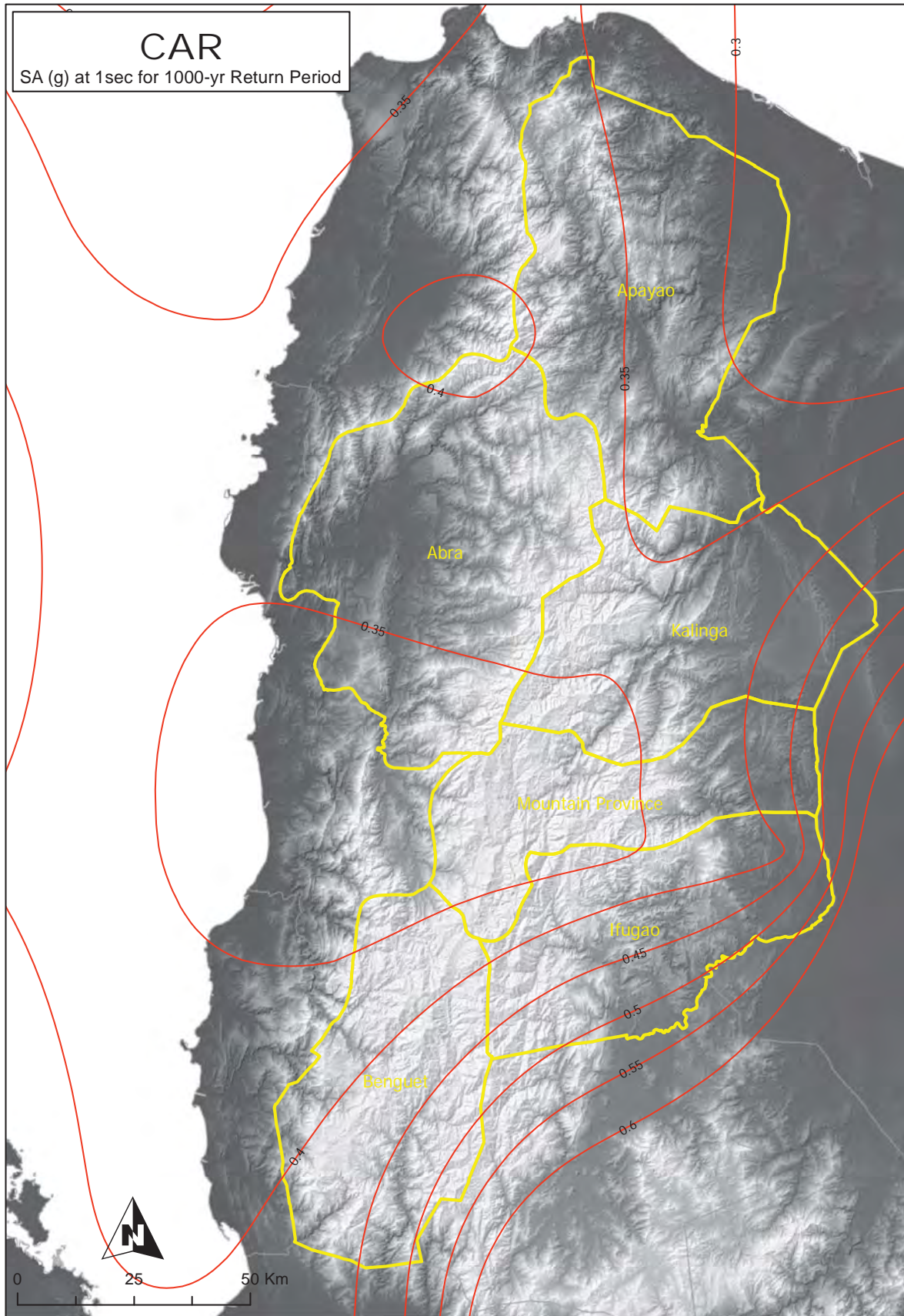
Figure 2A-55 CAR map of spectral acceleration at 1. sec. for 1,000-year return period
