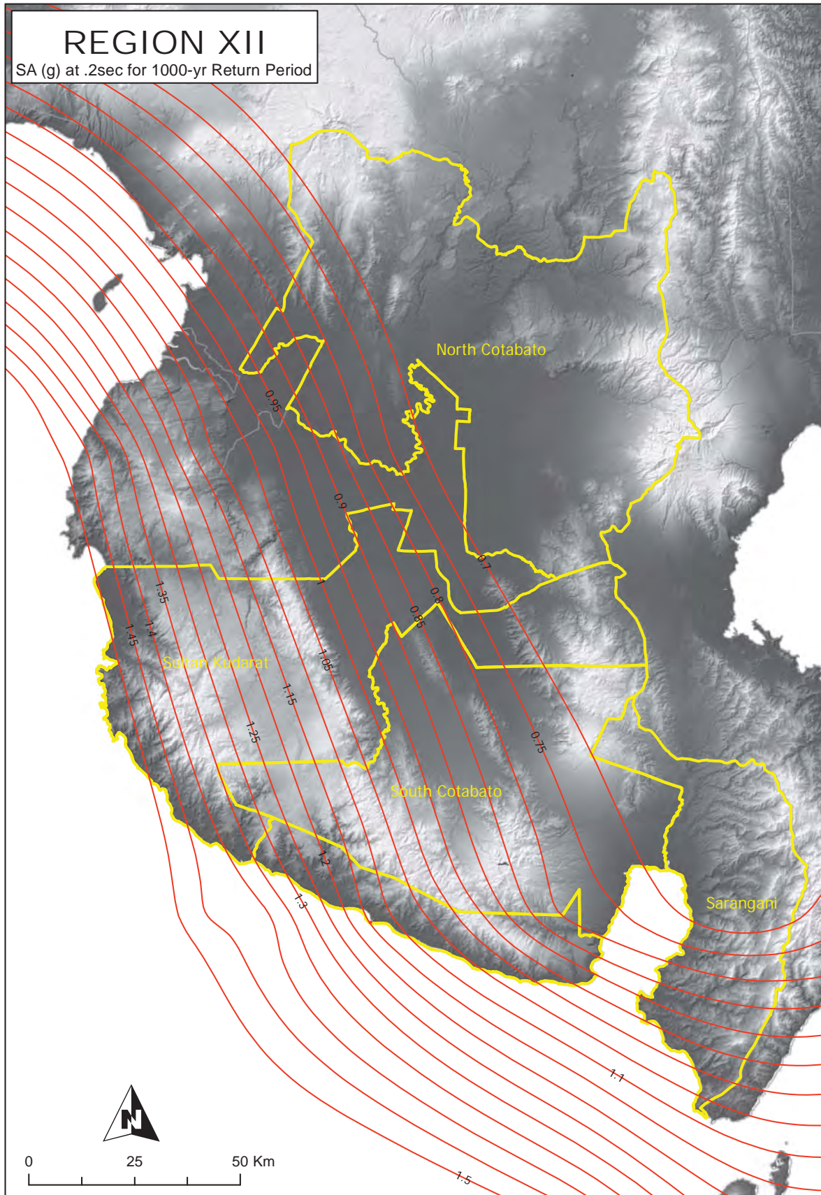
Figure 2A-51 Region XII map of spectral acceleration at 0.2 sec. for 1,000-year return period
