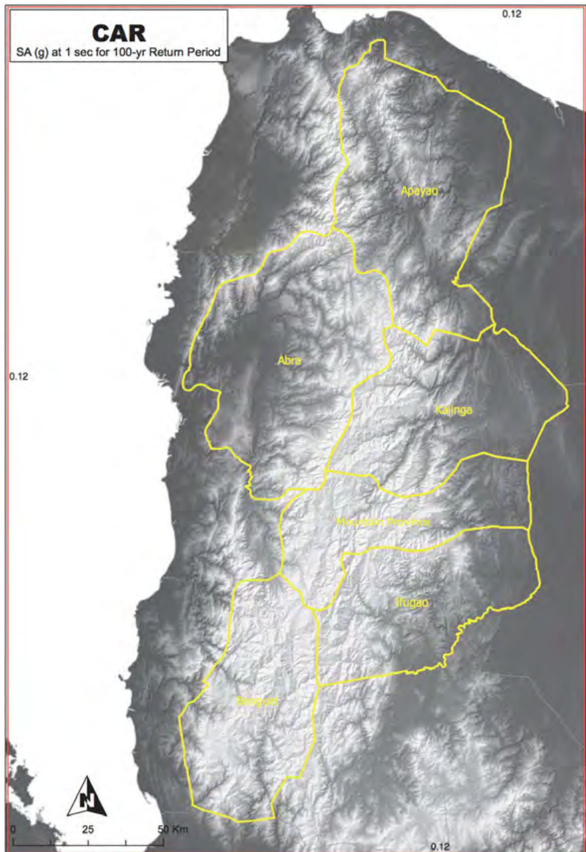
Figure 2A-163 CAR map of spectral acceleration at 1. sec. for 100-year return period
