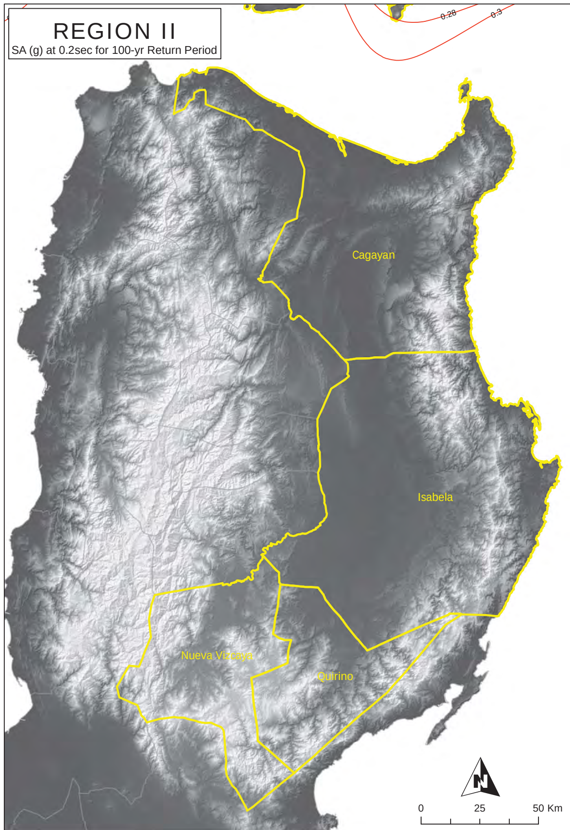
Figure 2A-144 Region II map of spectral acceleration at 0.2 sec. for 100-year return period
