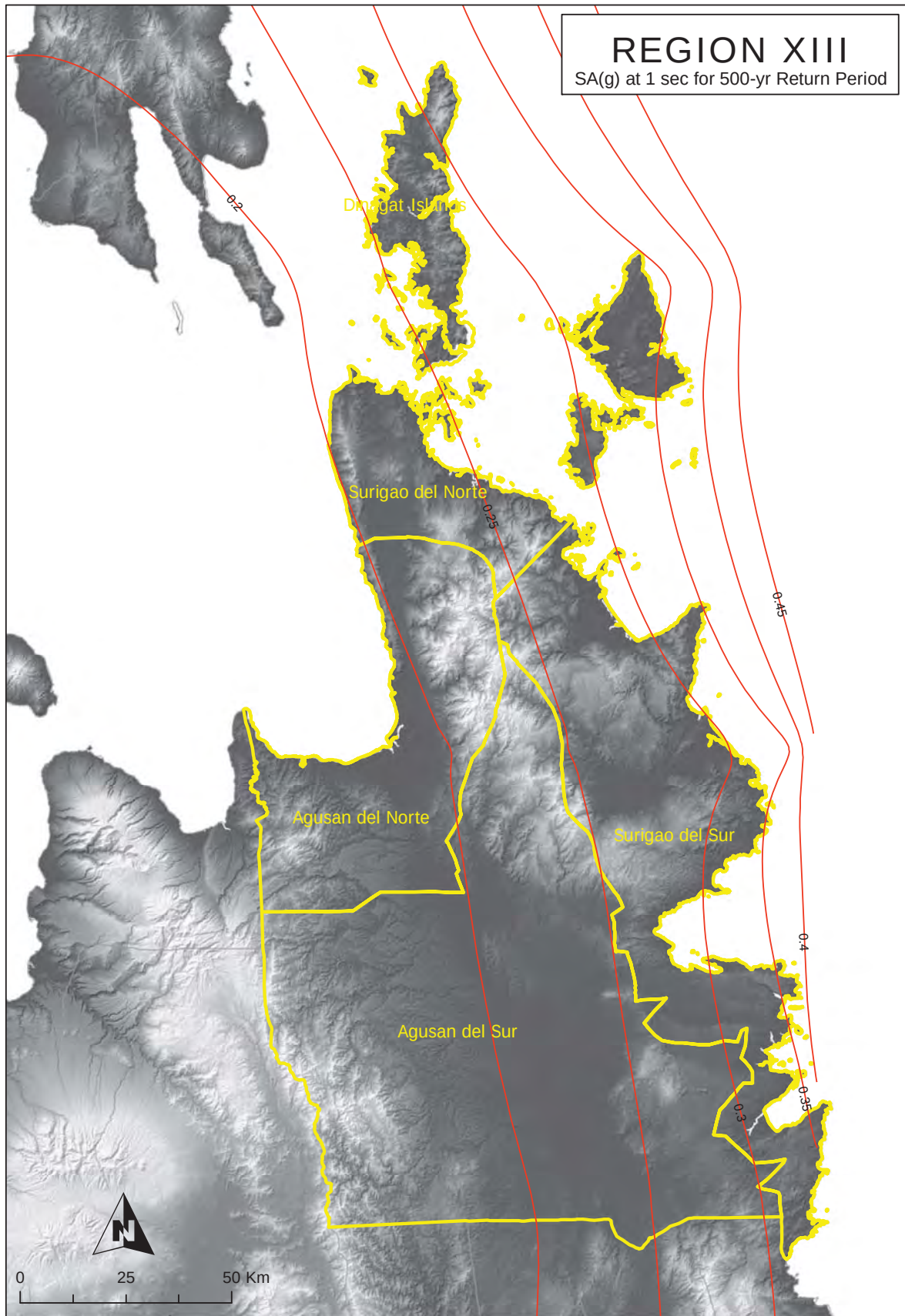
Figure 2A-121 Region XIII map of spectral acceleration at 1. sec. for 500-year return period
