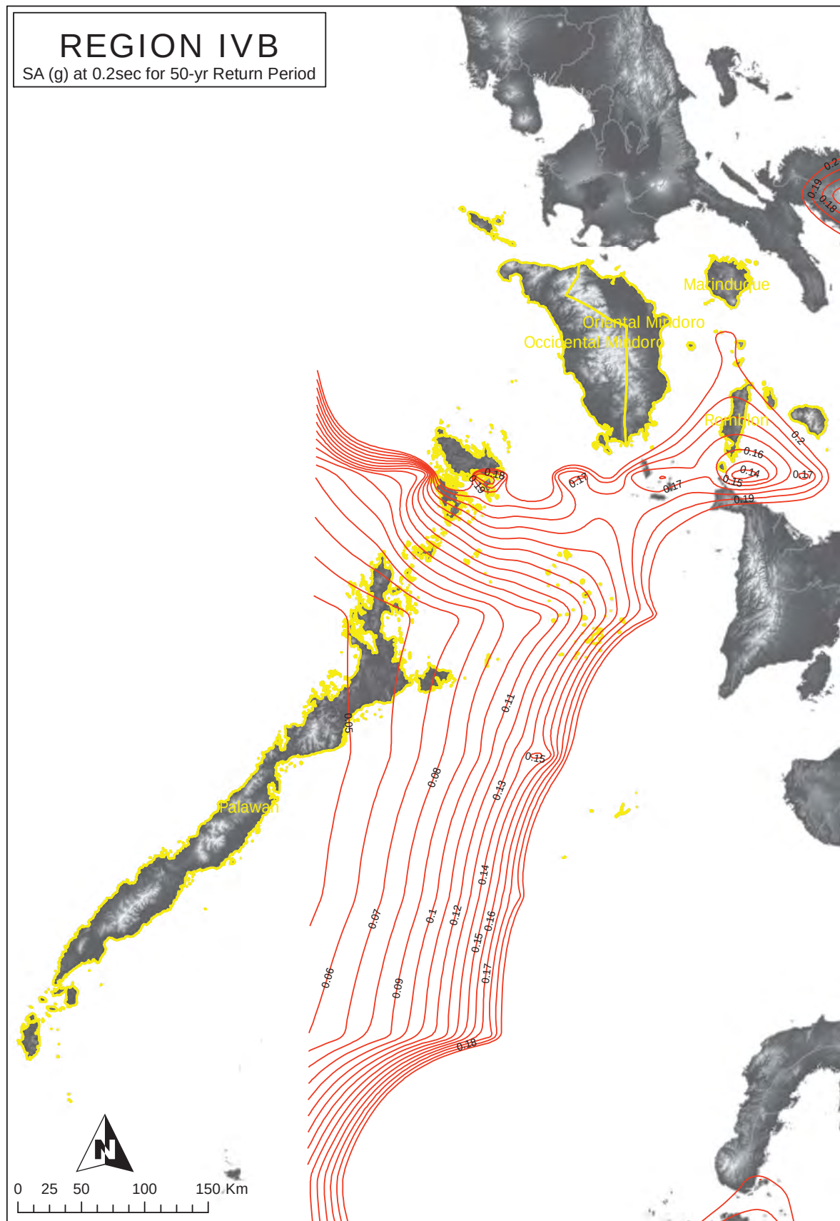
Figure 2A-204 Region IV-B map of spectral acceleration at 0.2 sec. for 50-year return period
