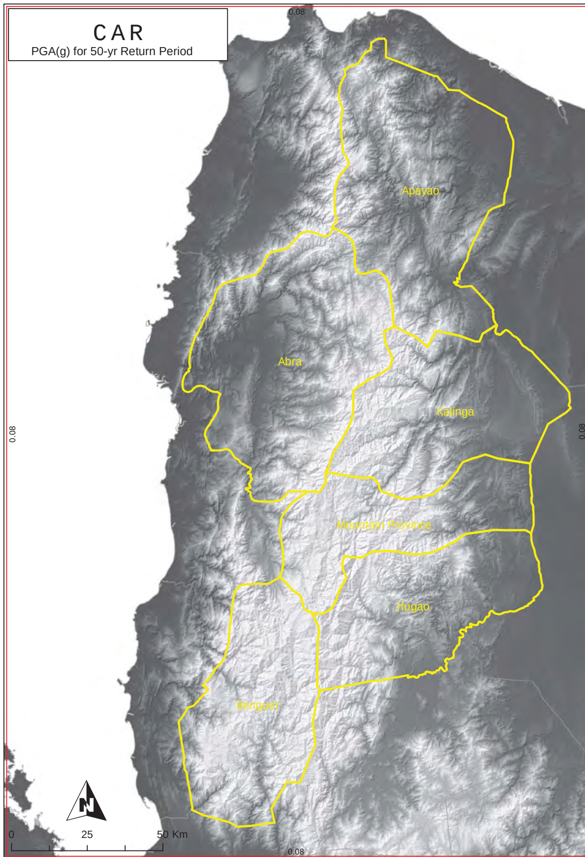
Figure 2A-181 CAR map of peak ground acceleration for 50-year return period
