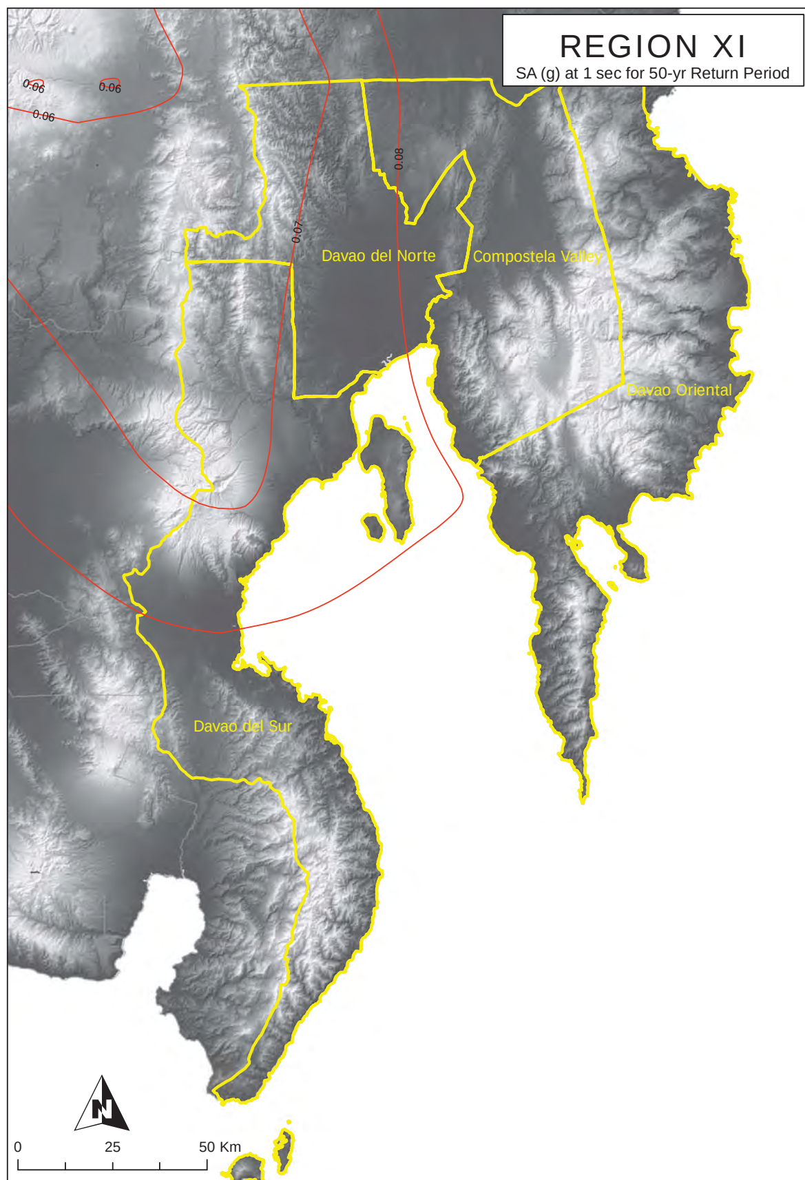
Figure 2A-228 Region XI map of spectral acceleration at 1. sec. for 50-year return period
