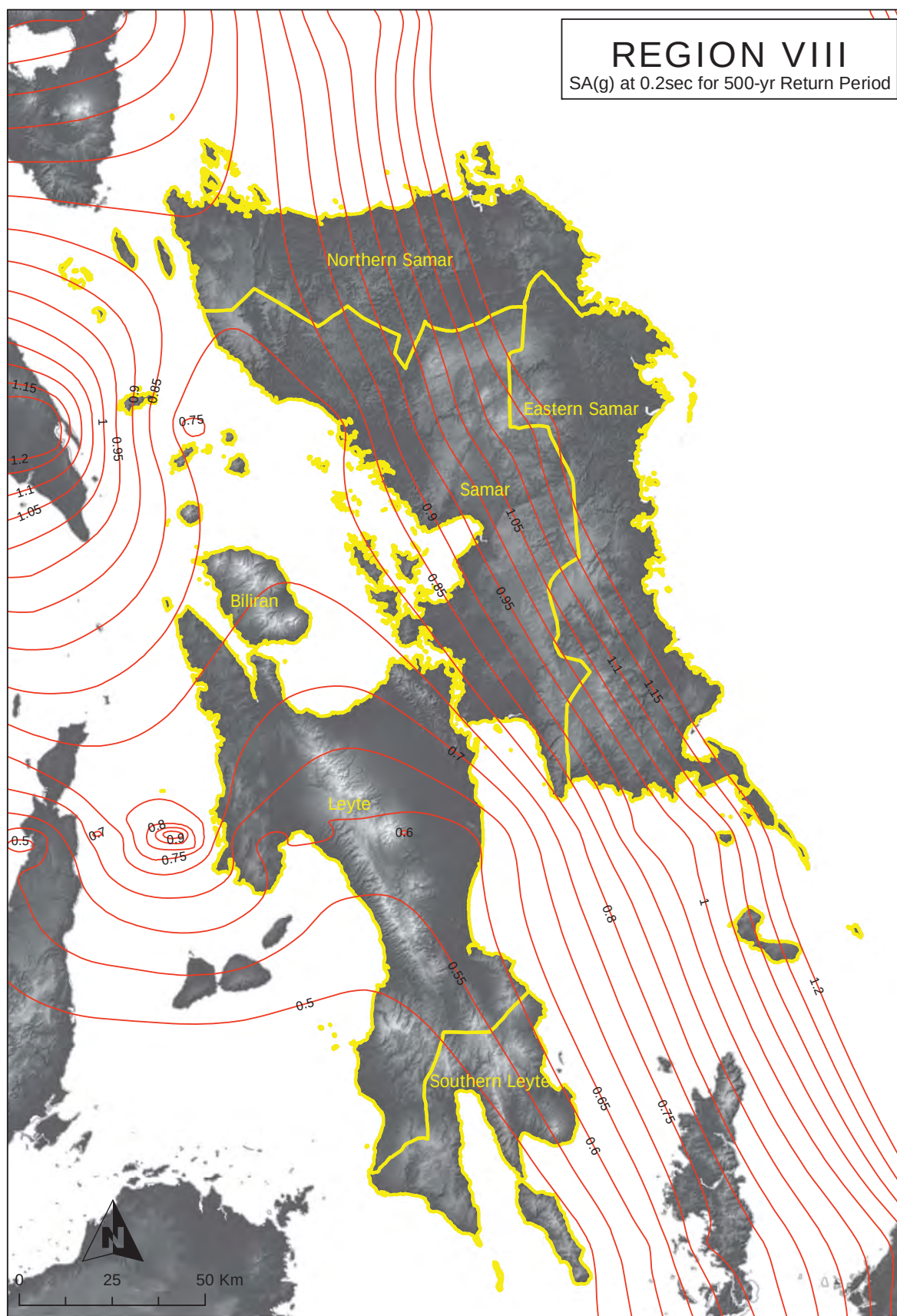
Figure 2A-99 Region VIII map of spectral acceleration at 0.2 sec. for 500-year return period
