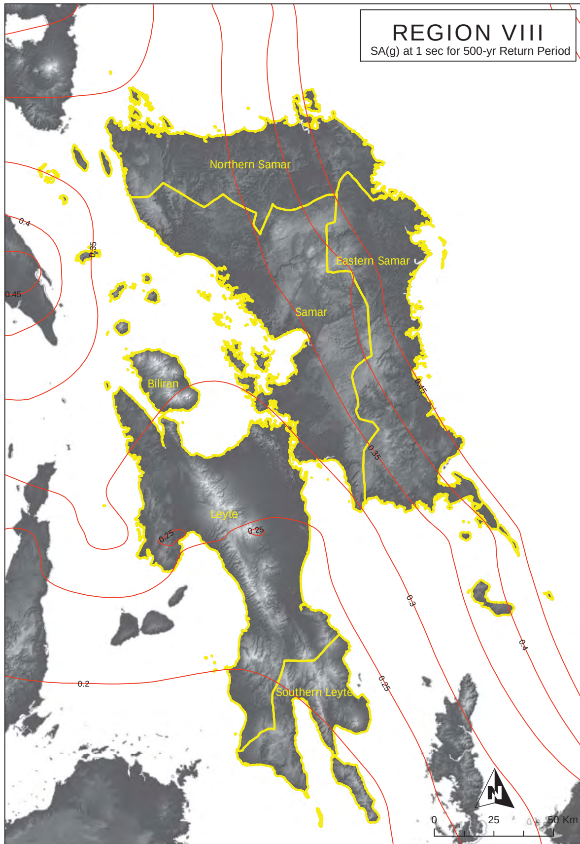
Figure 2A-117 Region VIII map of spectral acceleration at 1. sec. for 500-year return period
