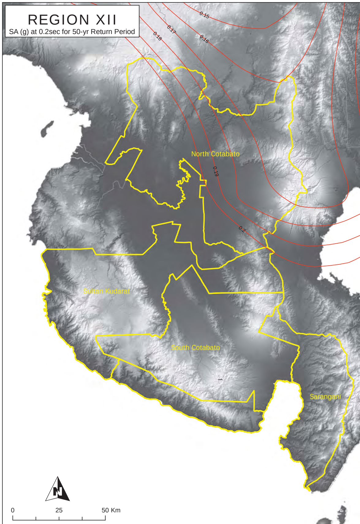
Figure 2A-213 Region XII map of spectral acceleration at 0.2 sec. for 50-year return period
