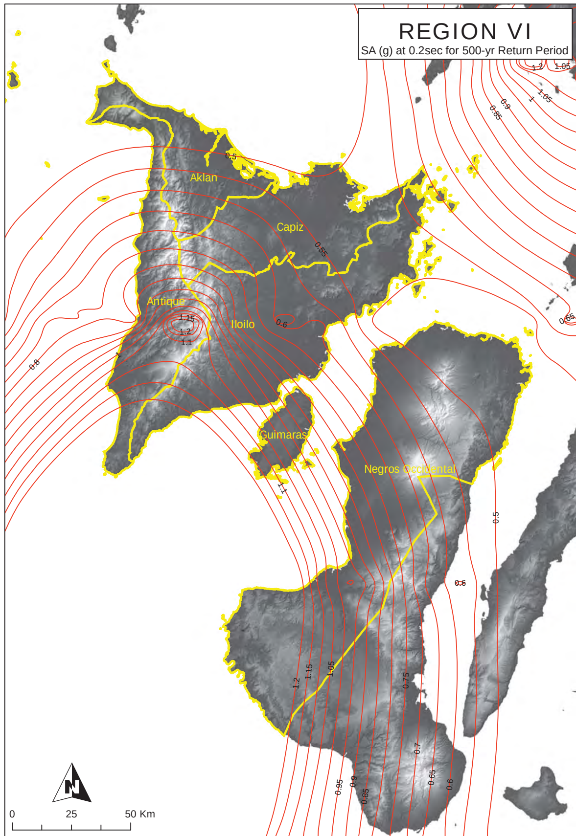
Figure 2A-97 Region VI map of spectral acceleration at 0.2 sec. for 500-year return period
