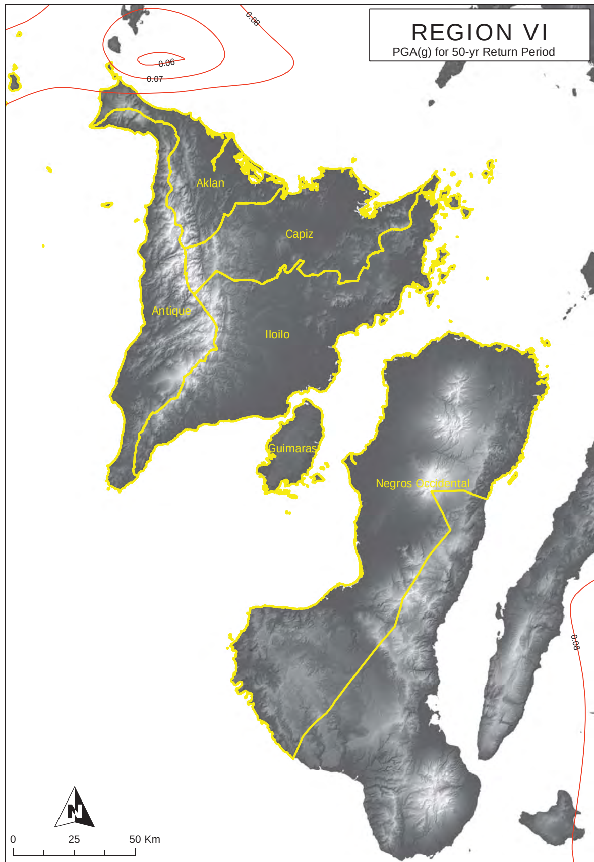
Figure 2A-187 Region VI map of peak ground acceleration for 50-year return period
