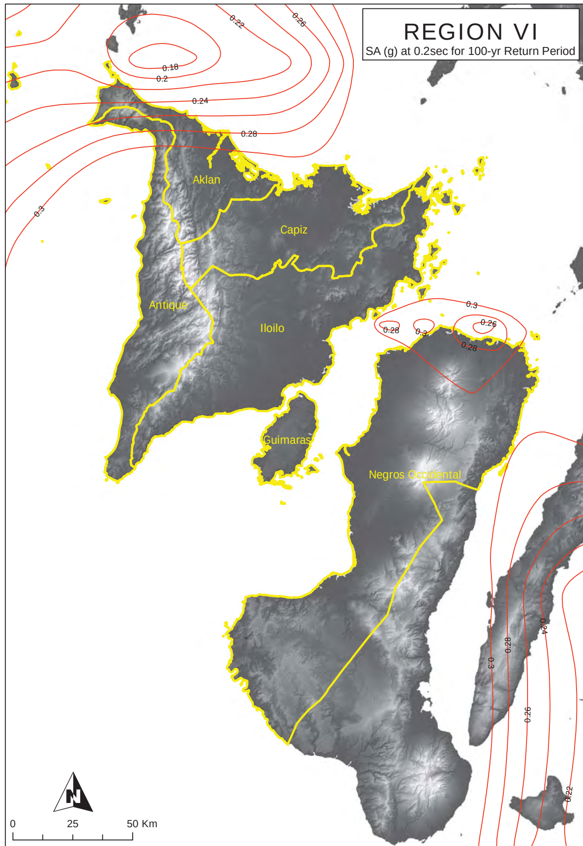
Figure 2A-151 Region VI map of spectral acceleration at 0.2 sec. for 100-year return period
