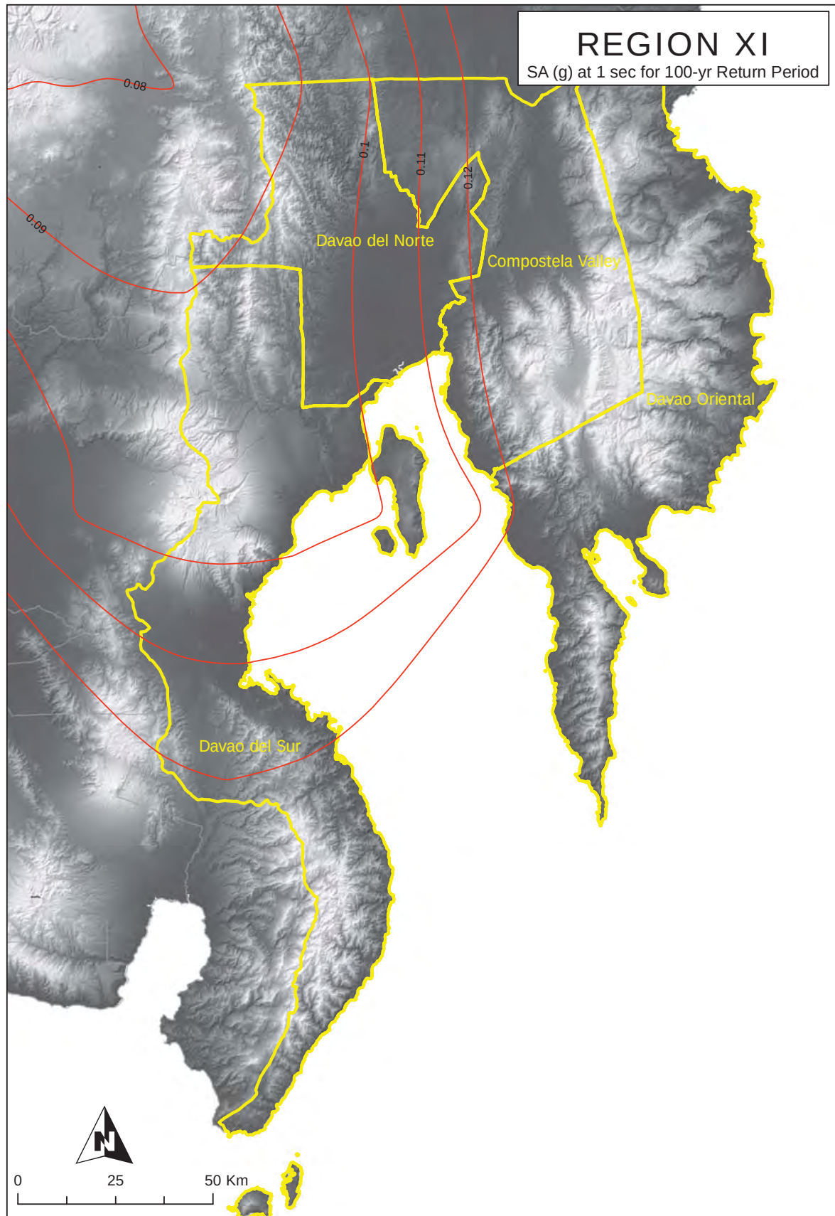
Figure 2A-174 Region XI map of spectral acceleration at 1. sec. for 100-year return period
