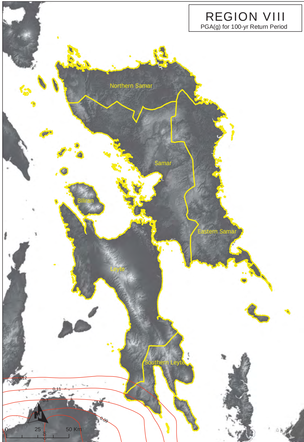
Figure 2A-135 Region VIII map of peak ground acceleration for 100-year return period
