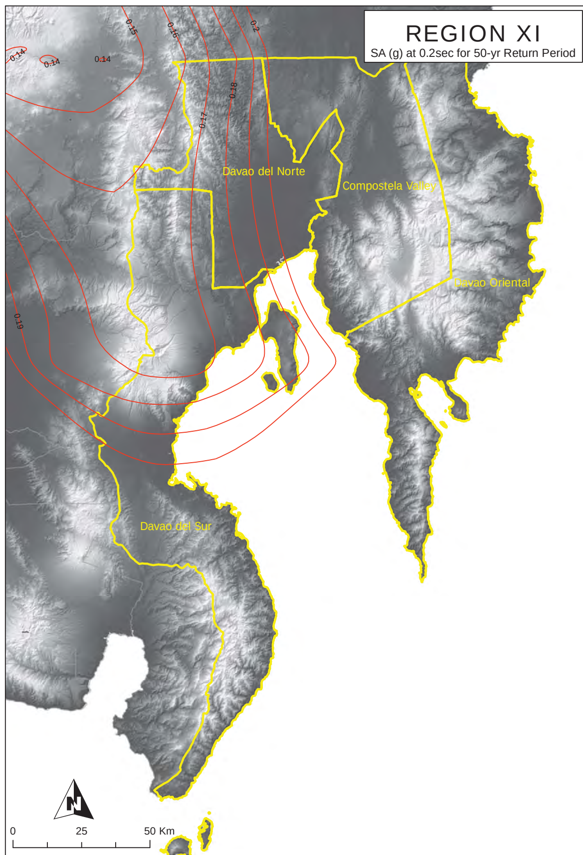
Figure 2A-210 Region XI map of spectral acceleration at 0.2 sec. for 50-year return period
