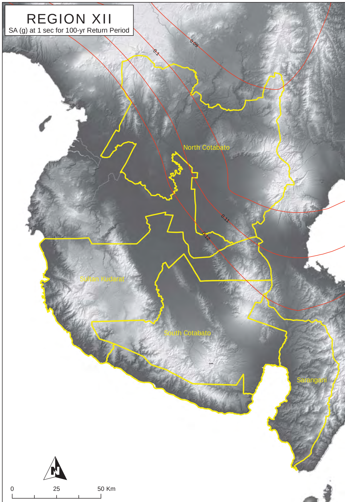
Figure 2A-177 Region XII map of spectral acceleration at 1. sec. for 100-year return period
