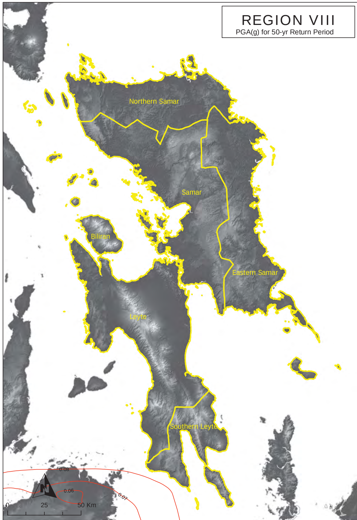
Figure 2A-189 Region VIII map of peak ground acceleration for 50-year return period
