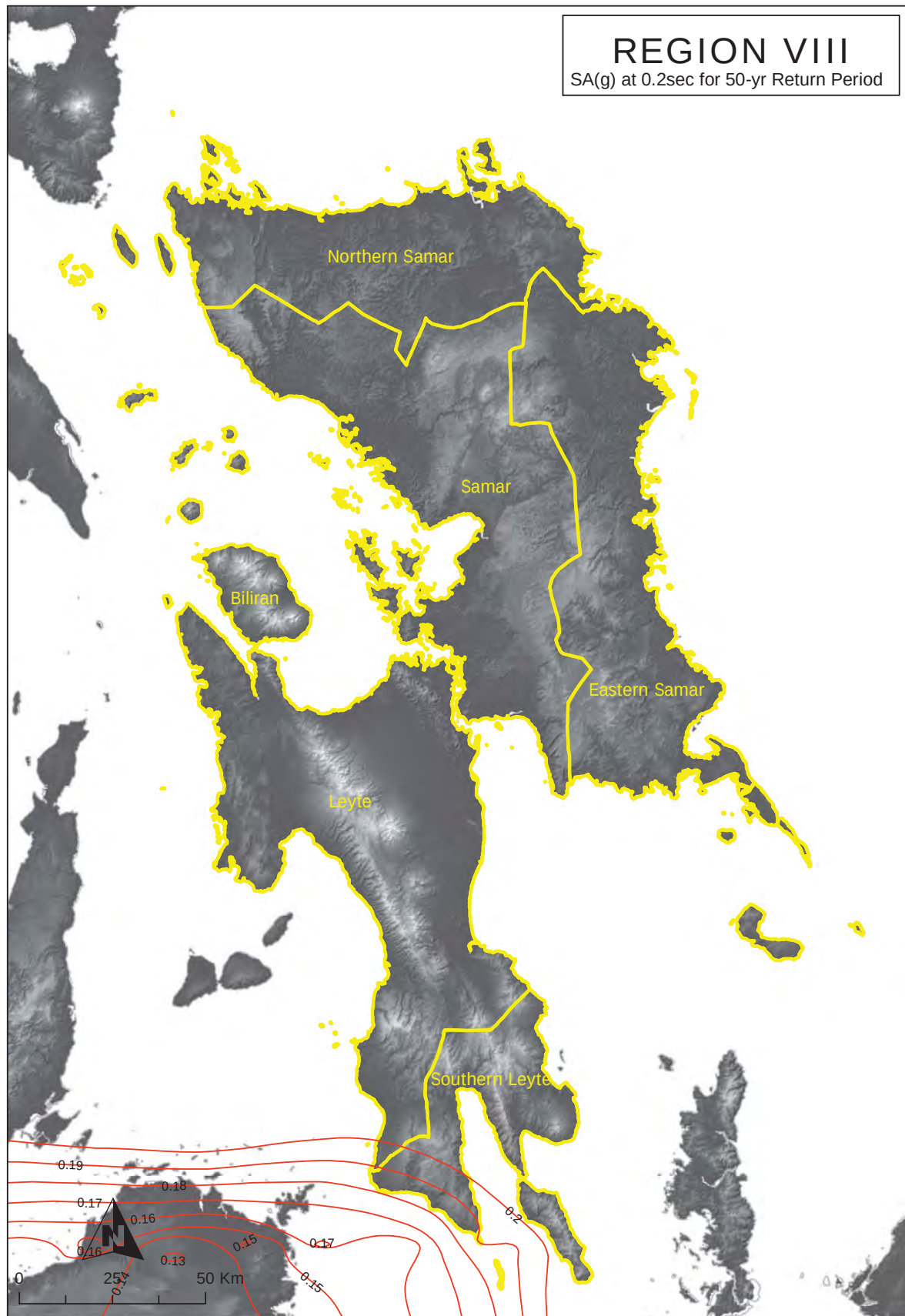
Figure 2A-207 Region VIII map of spectral acceleration at 0.2 sec. for 50-year return period
