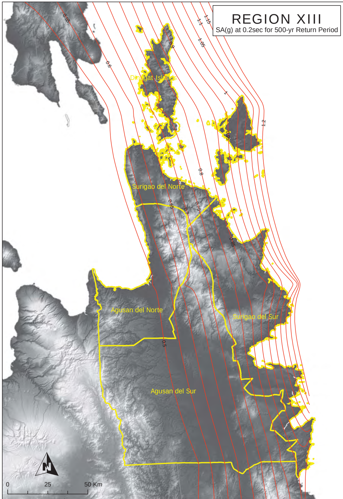
Figure 2A-103 Region XIII map of spectral acceleration at 0.2 sec. for 500-year return period
