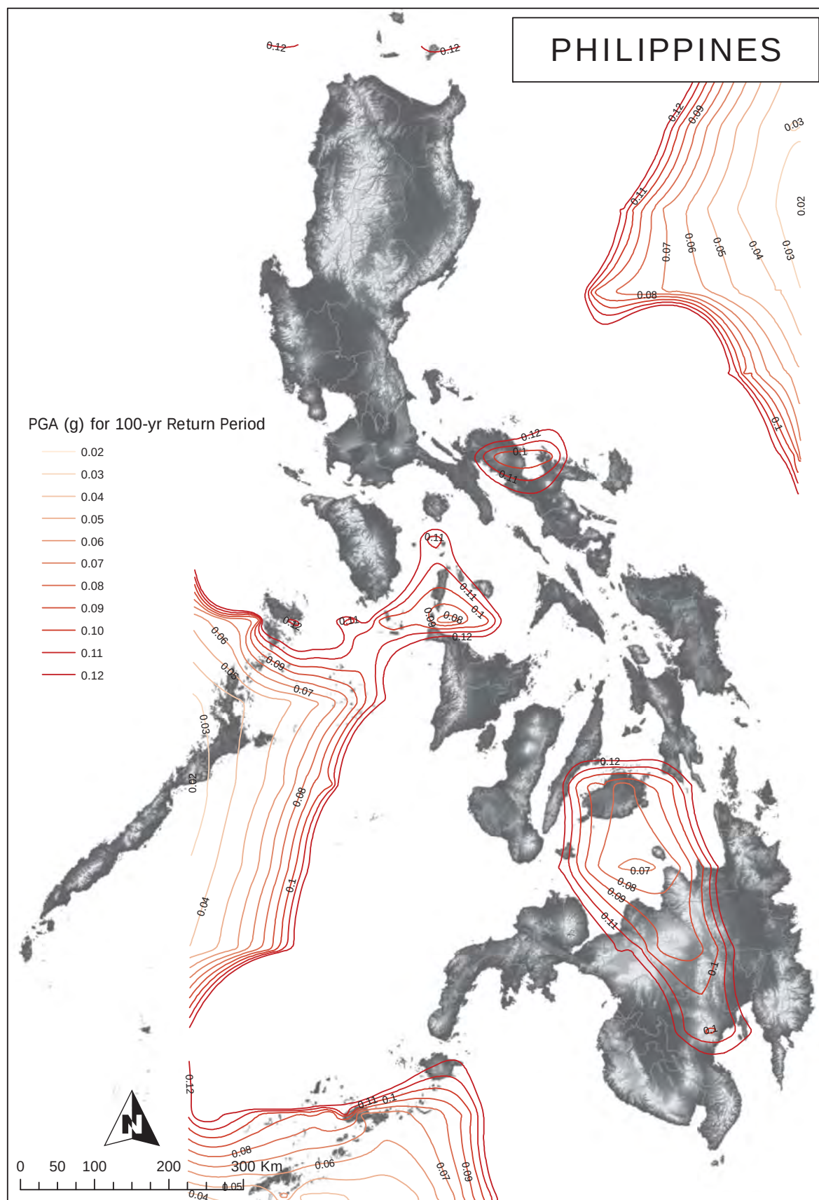
Figure 2A-124 Contour map of peak ground acceleration for 100-year return period
