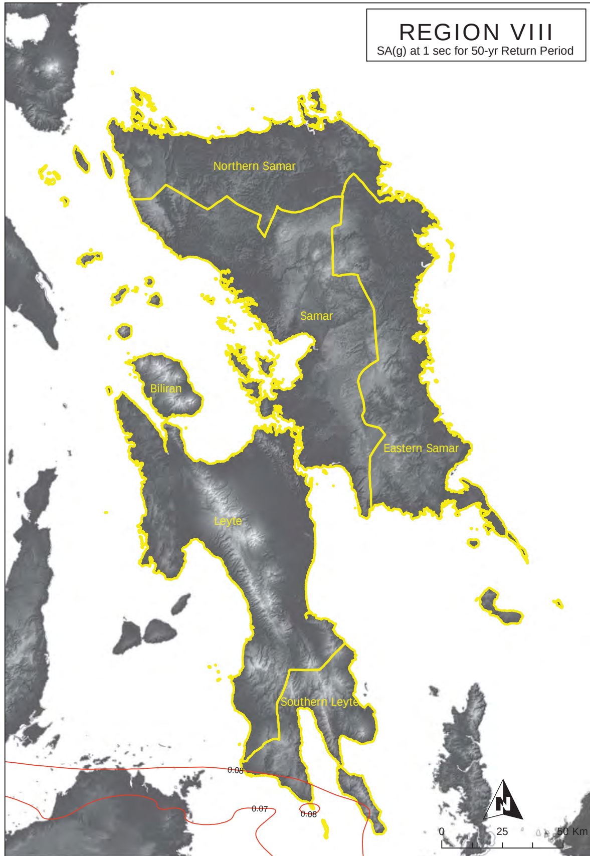
Figure 2A-225 Region VIII map of spectral acceleration at 1. sec. for 50-year return period
