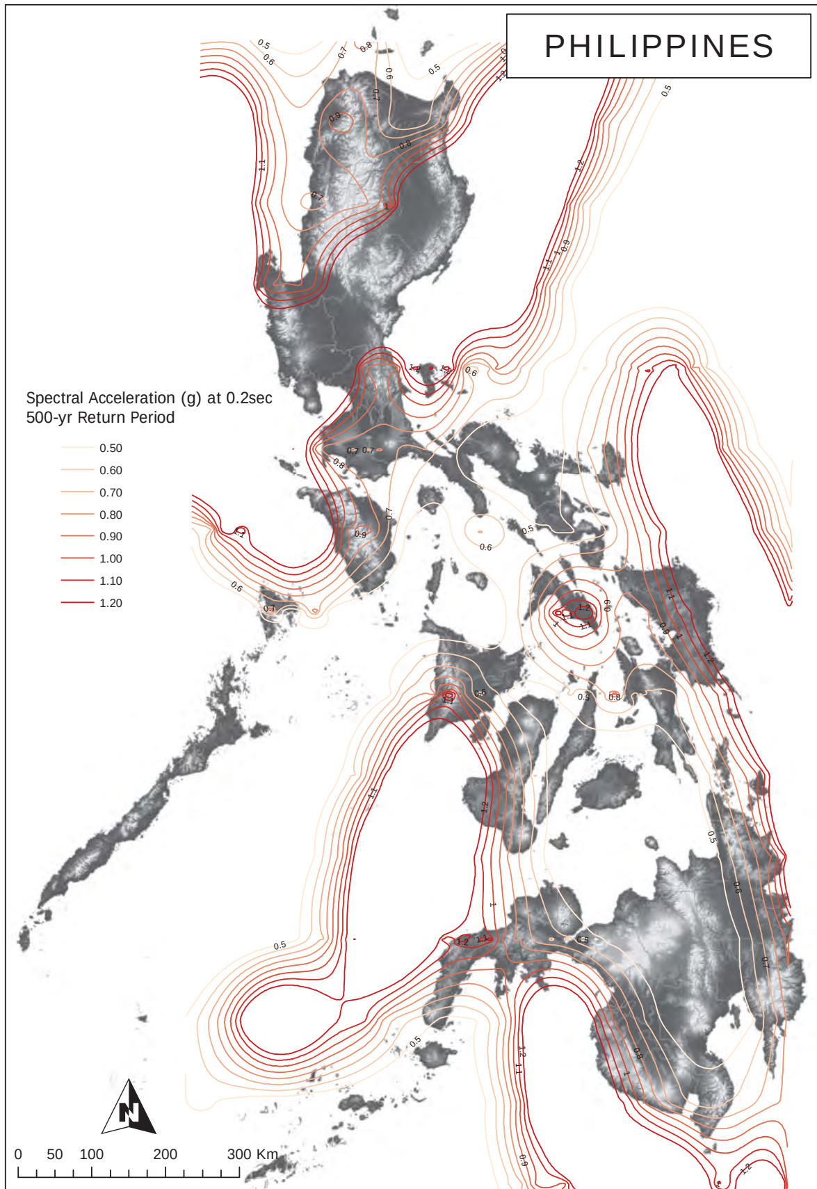
Figure 2A-88 Contour map of spectral acceleration at 0.2 sec. for 500-year return period
