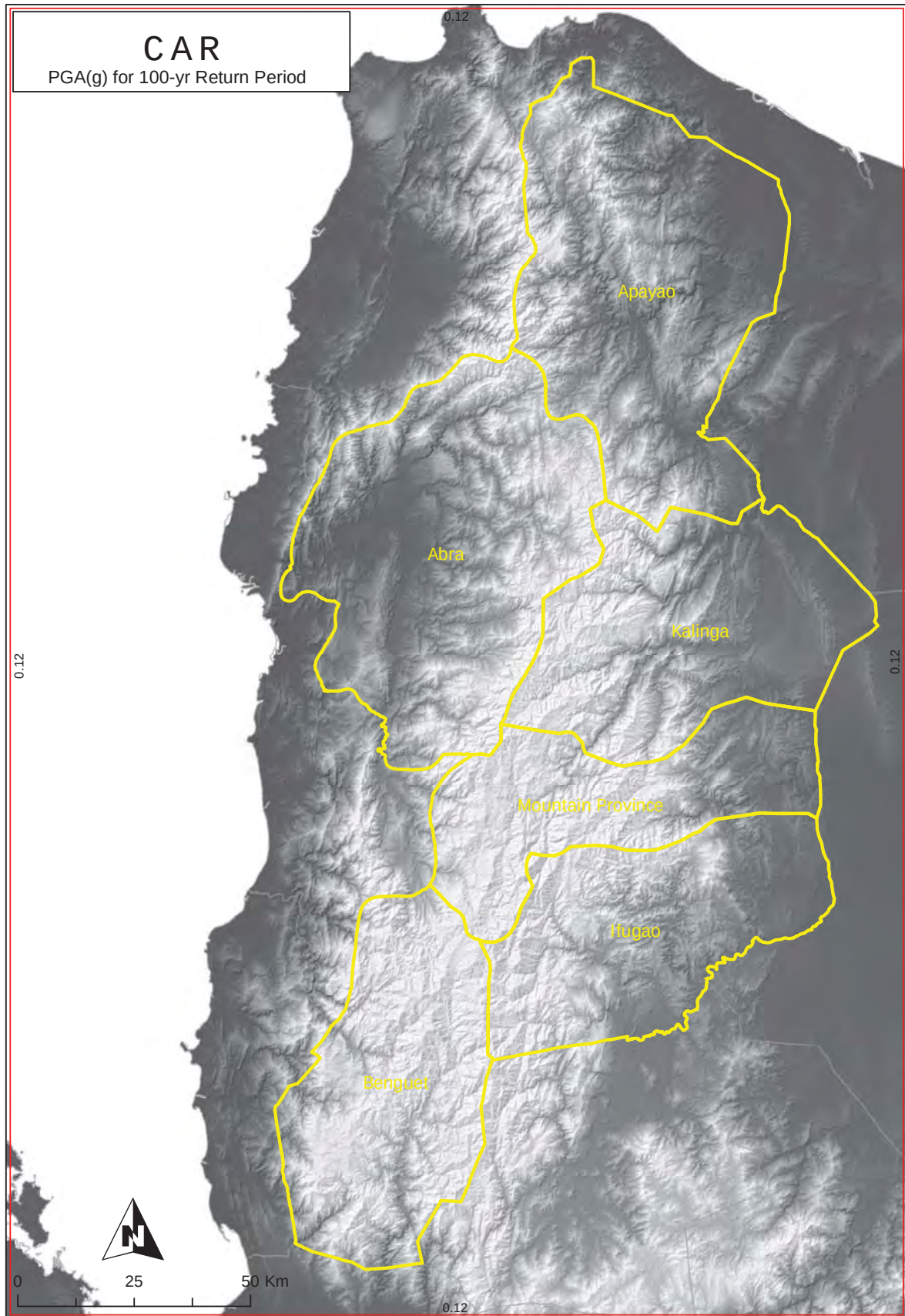
Figure 2A-127 CAR map of peak ground acceleration for 100-year return period
