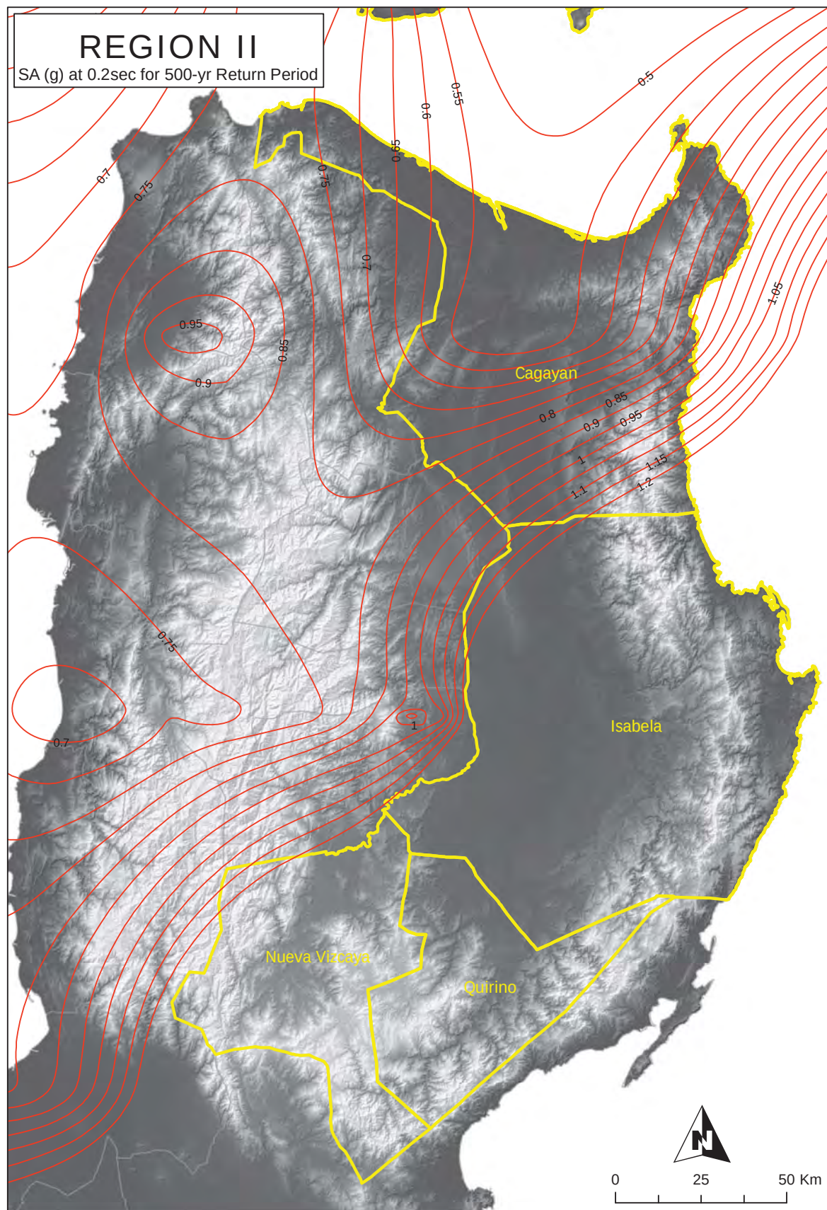
Figure 2A-90 Region II map of spectral acceleration at 0.2 sec. for 500-year return period
