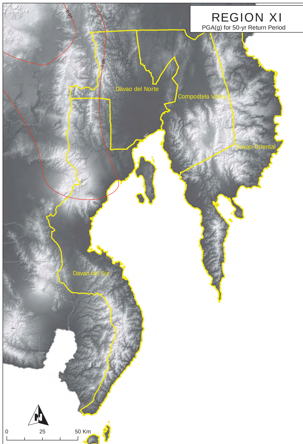
Figure 2A-192 Region XI map of peak ground acceleration for 50-year return period
