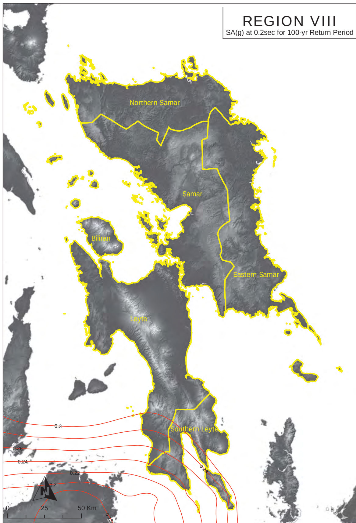
Figure 2A-153 Region VIII map of spectral acceleration at 0.2 sec. for 100-year return period
