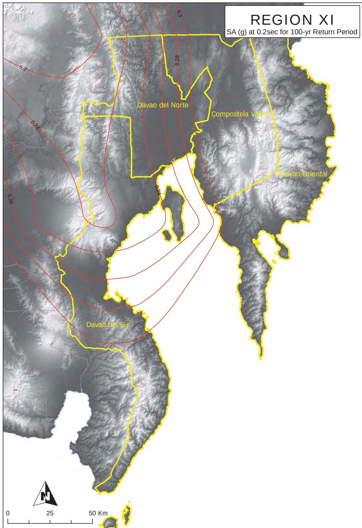
Figure 2A-156 Region XI map of spectral acceleration at 0.2 sec. for 100-year return period
