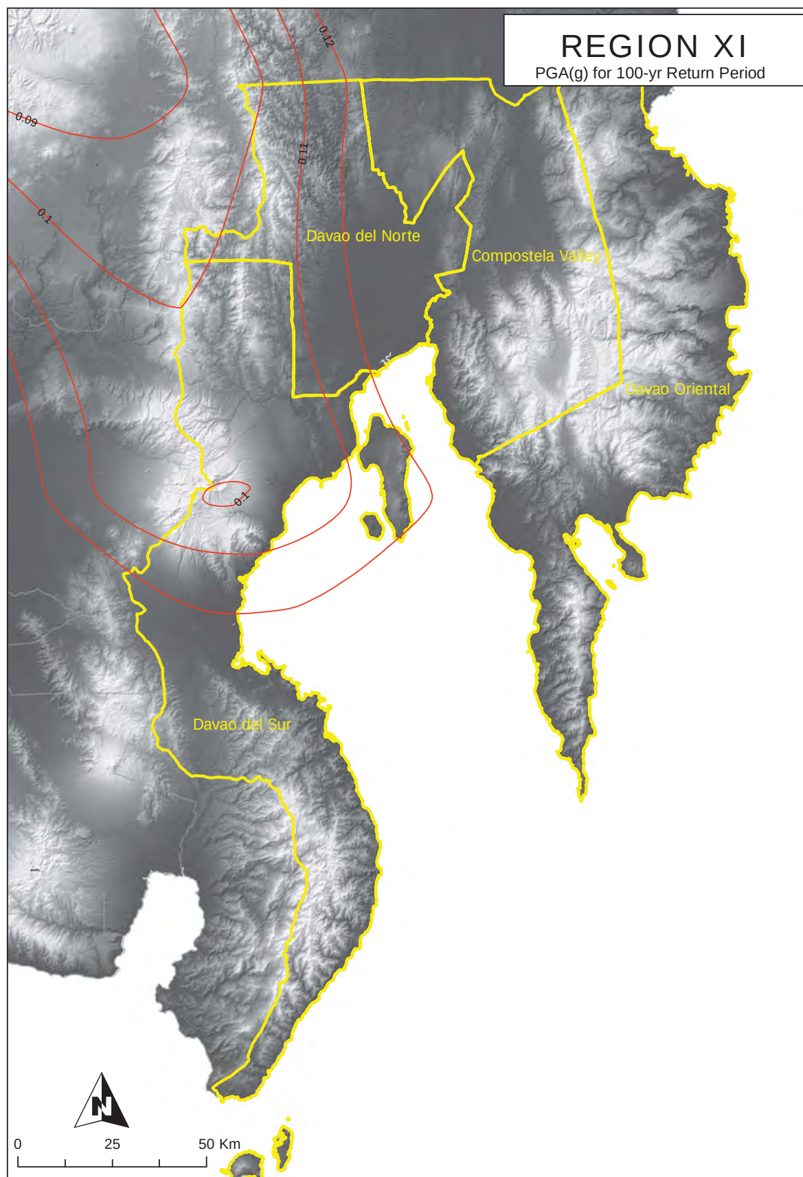
Figure 2A-138 Region XI map of peak ground acceleration for 100-year return period
