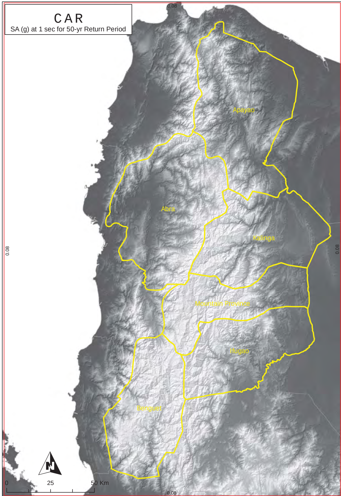
Figure 2A-217 CAR map of spectral acceleration at 1. sec. for 50-year return period
