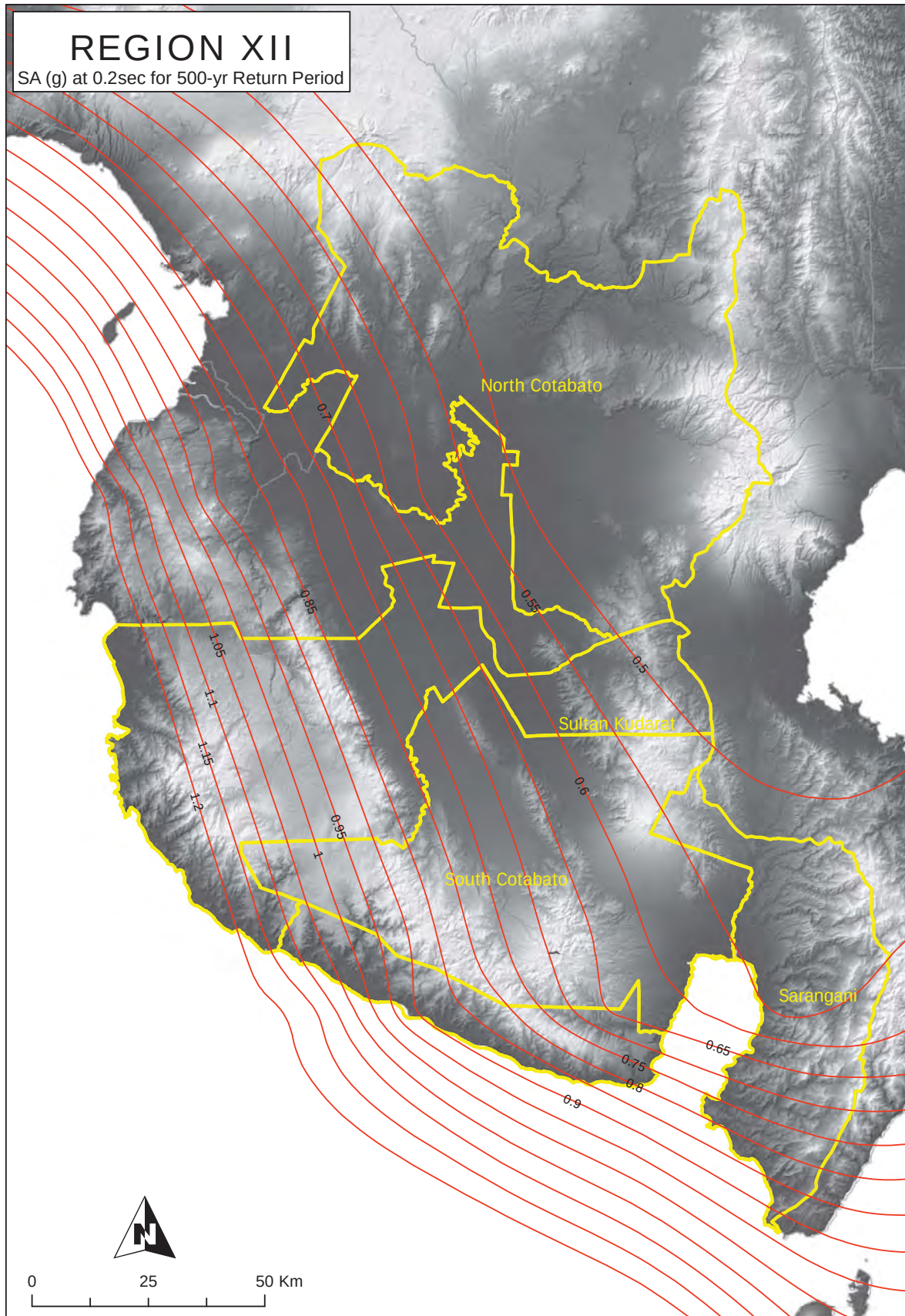
Figure 2A-105 Region XII map of spectral acceleration at 0.2 sec. for 500-year return period
