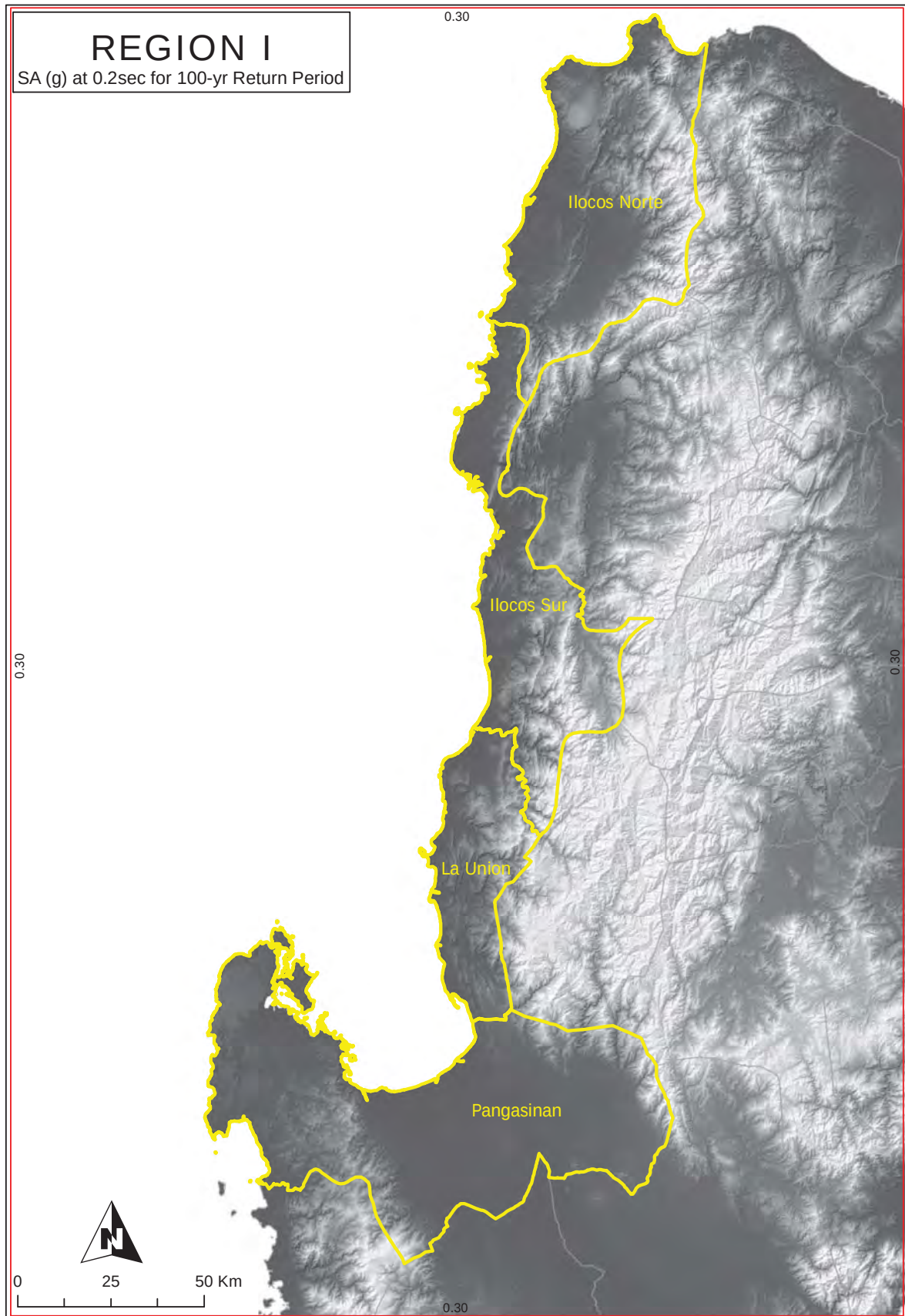
Figure 2A-143 Region I map of spectral acceleration at 0.2 sec. for 100-year return period
