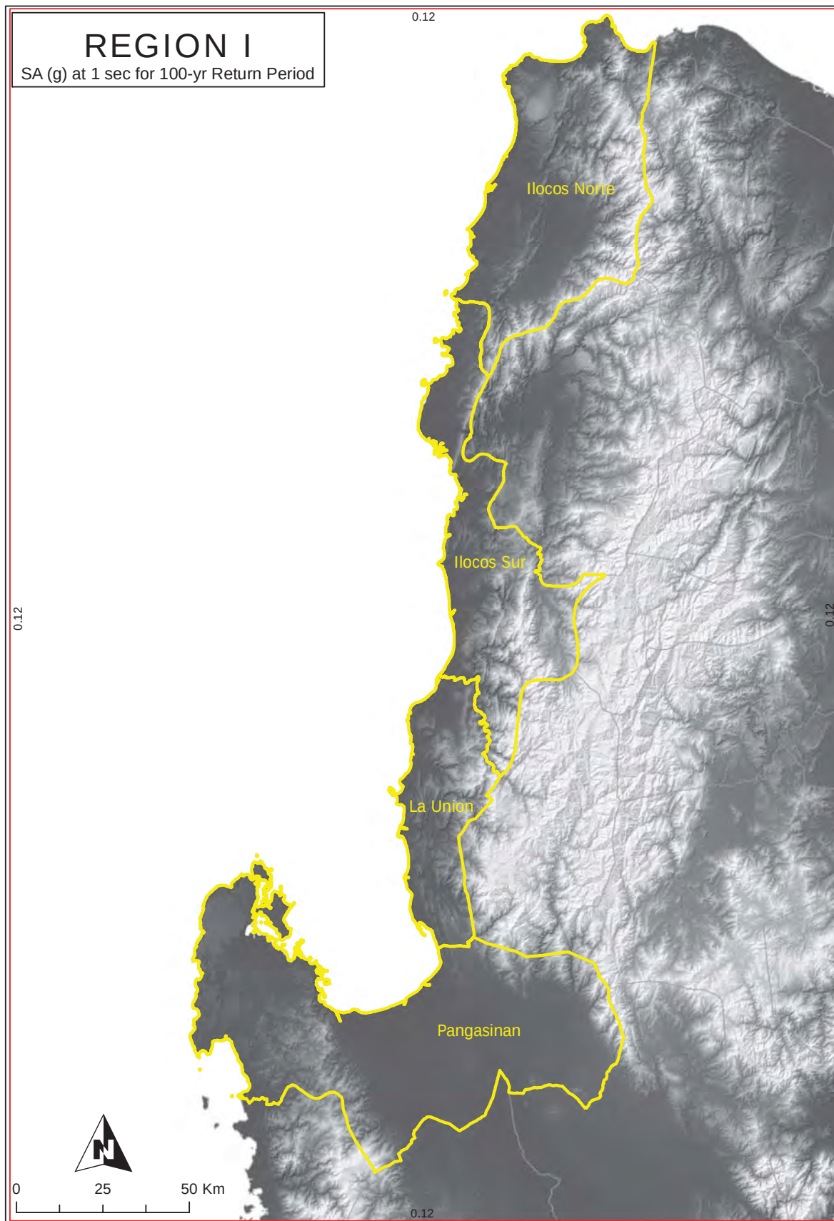
Figure 2A-161 Region I map of spectral acceleration at 1. sec. for 100-year return period
