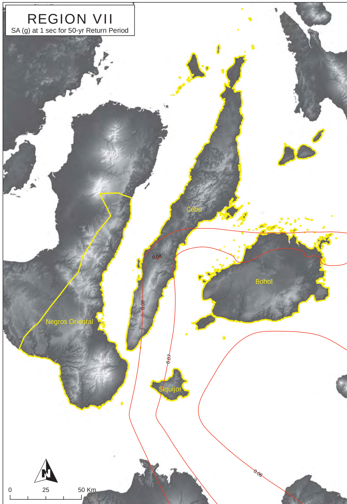
Figure 2A-224 Region VII map of spectral acceleration at 1. sec. for 50-year return period
