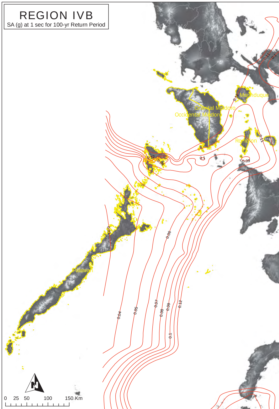
Figure 2A-168 Region IV-B map of spectral acceleration at 1. sec. for 100-year return period
