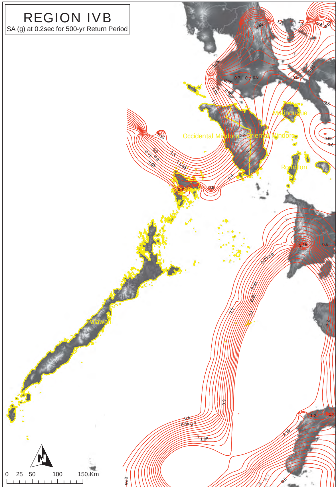
Figure 2A-96 Region IV-B map of spectral acceleration at 0.2 sec. for 500-year return period
