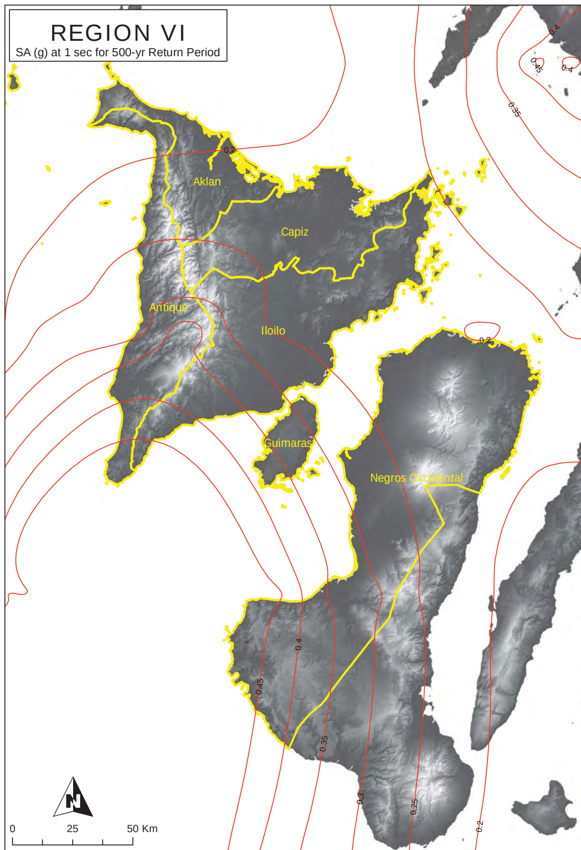
Figure 2A-115 Region VI map of spectral acceleration at 1. sec. for 500-year return period
