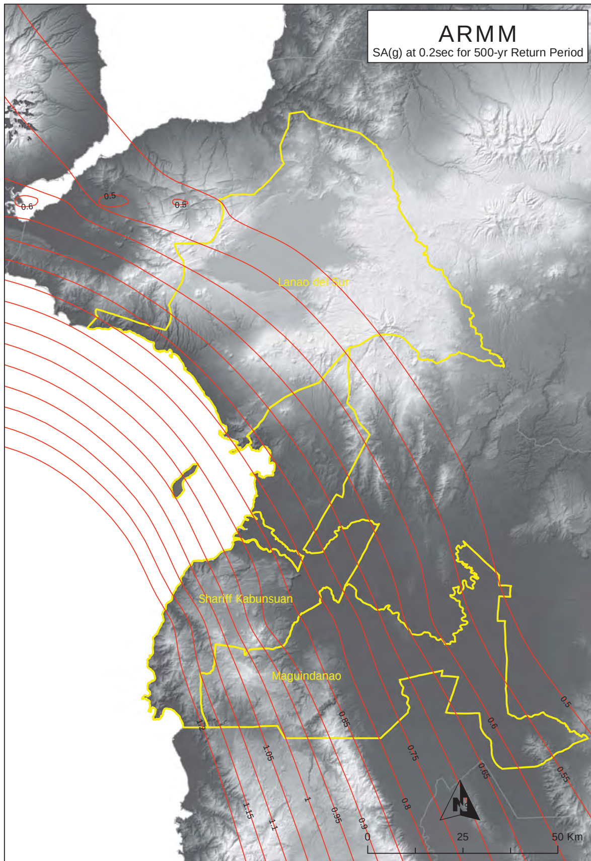
Figure 2A-104 ARMM map of spectral acceleration at 0.2 sec. for 500-year return period
