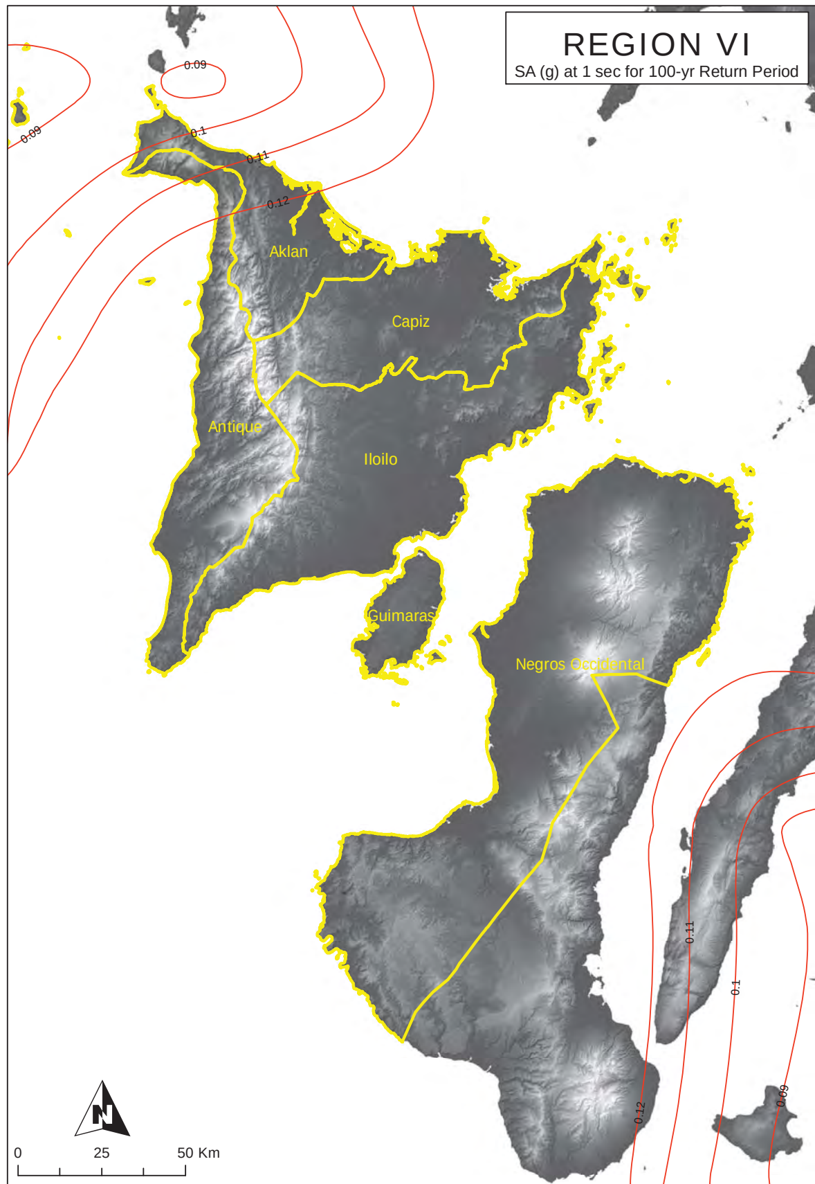
Figure 2A-169 Region VI map of spectral acceleration at 1. sec. for 100-year return period
