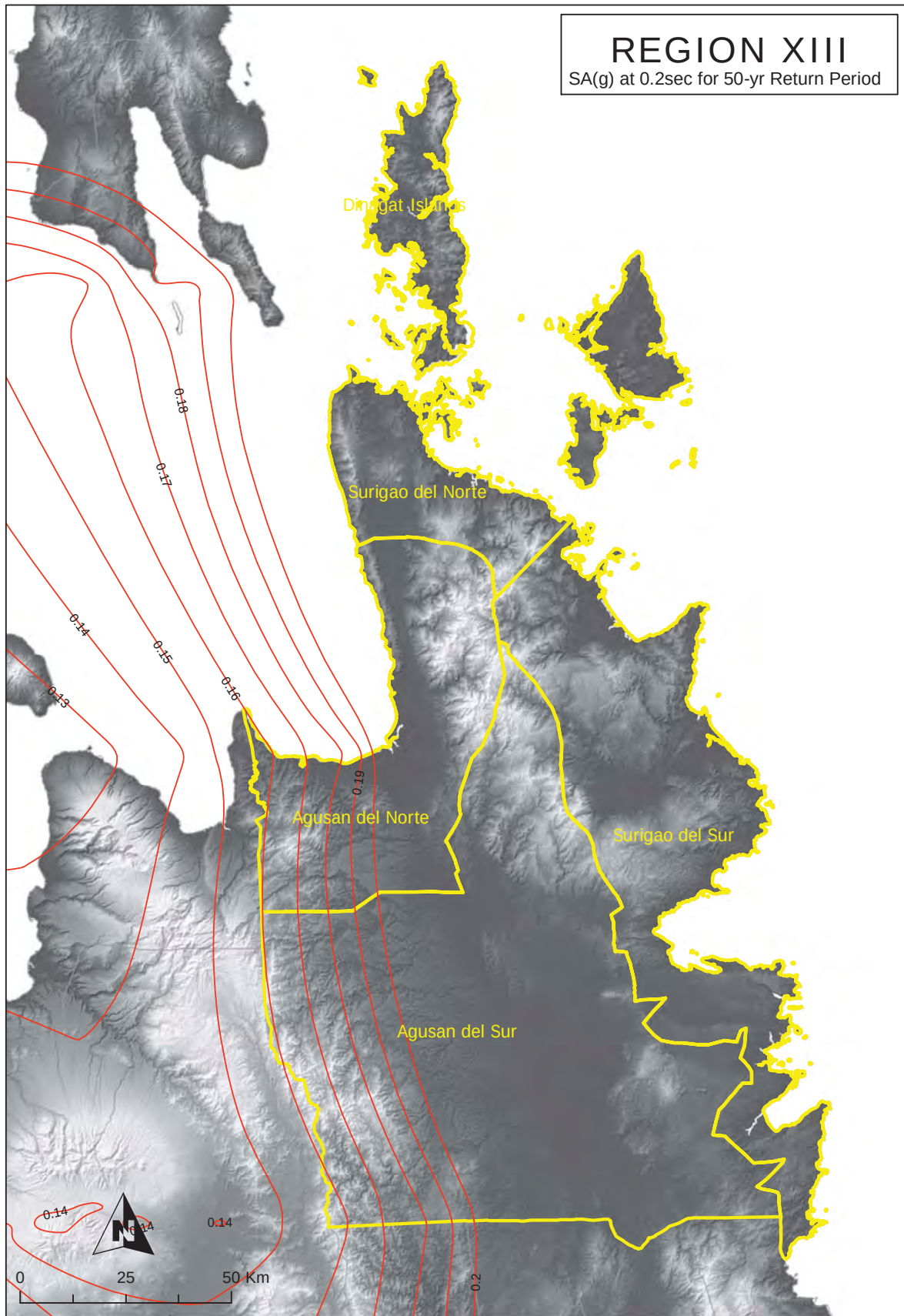
Figure 2A-211 Region XIII map of spectral acceleration at 0.2 sec. for 50-year return period
