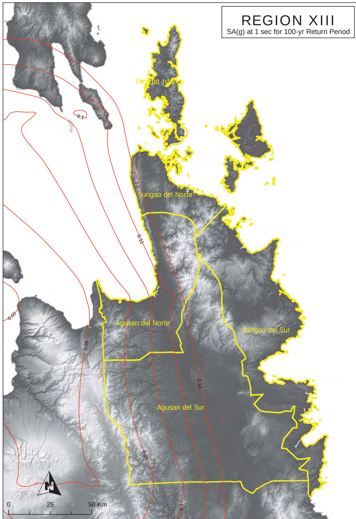
Figure 2A-175 Region XIII map of spectral acceleration at 1. sec. for 100-year return period
