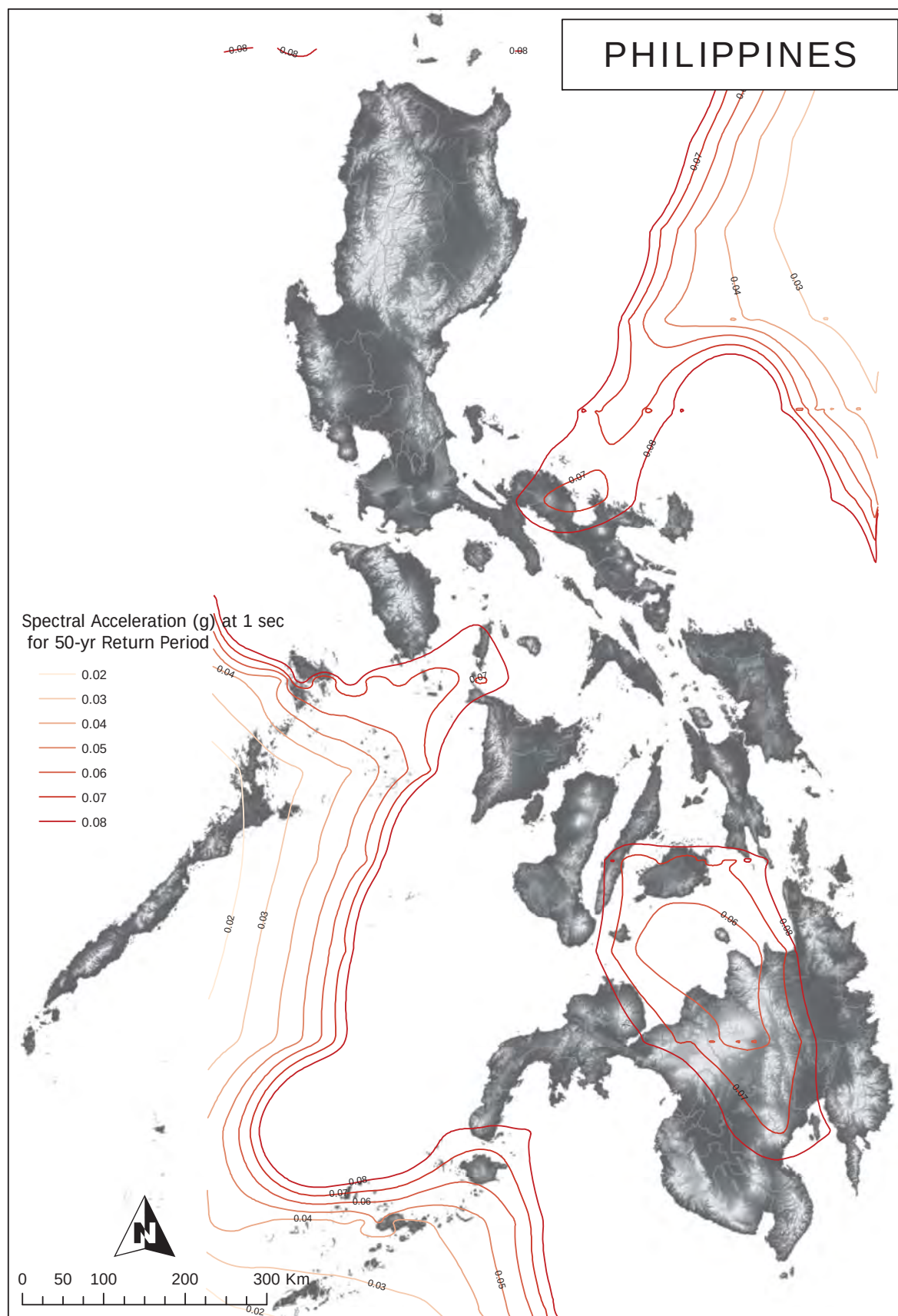
Figure 2A-214 Contour map of spectral acceleration at 1. sec. for 50-year return period
