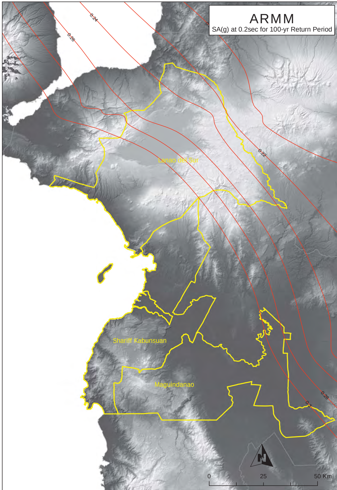
Figure 2A-158 ARMM map of spectral acceleration at 0.2 sec. for 100-year return period
