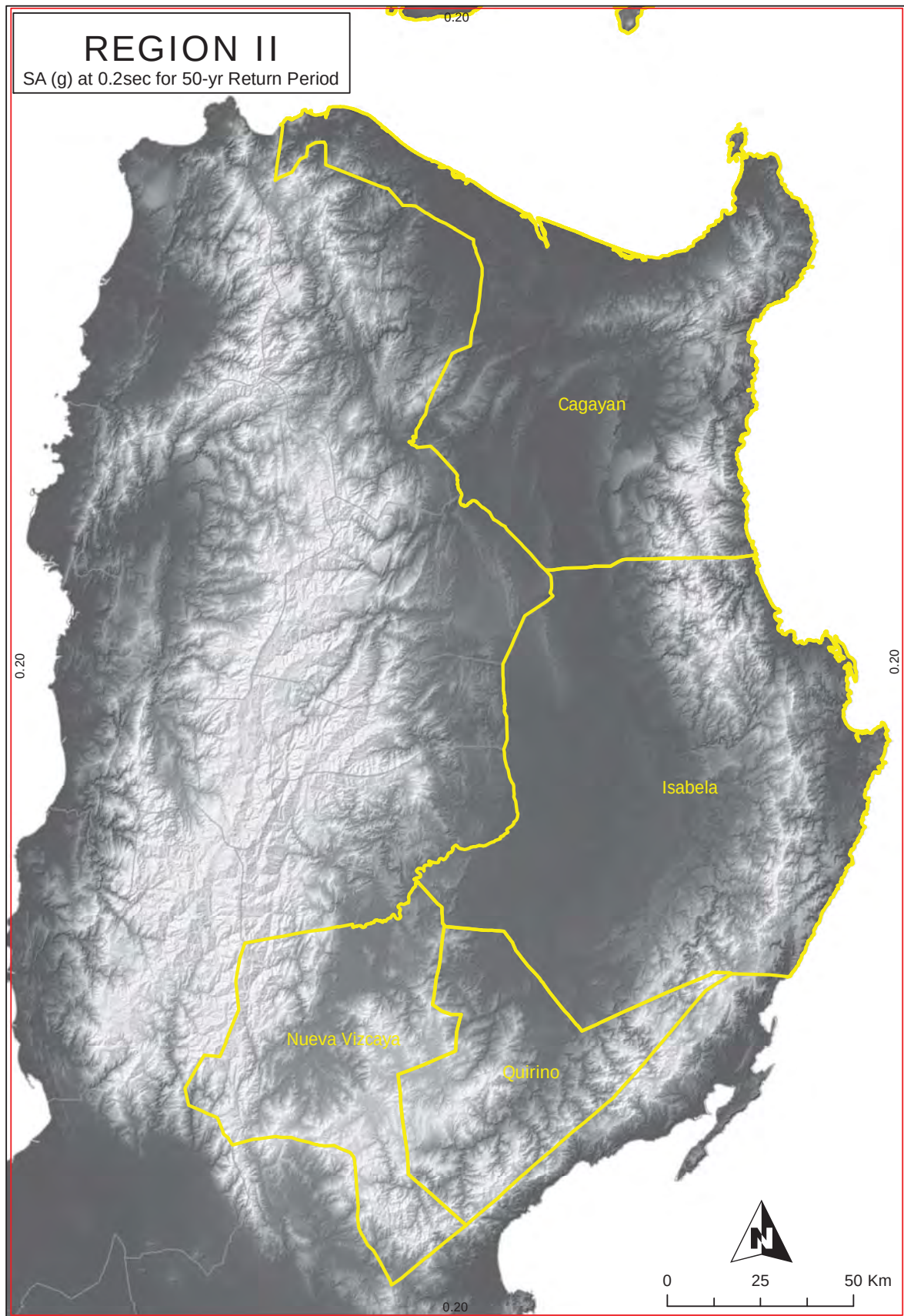
Figure 2A-198 Region II map of spectral acceleration at 0.2 sec. for 50-year return period
