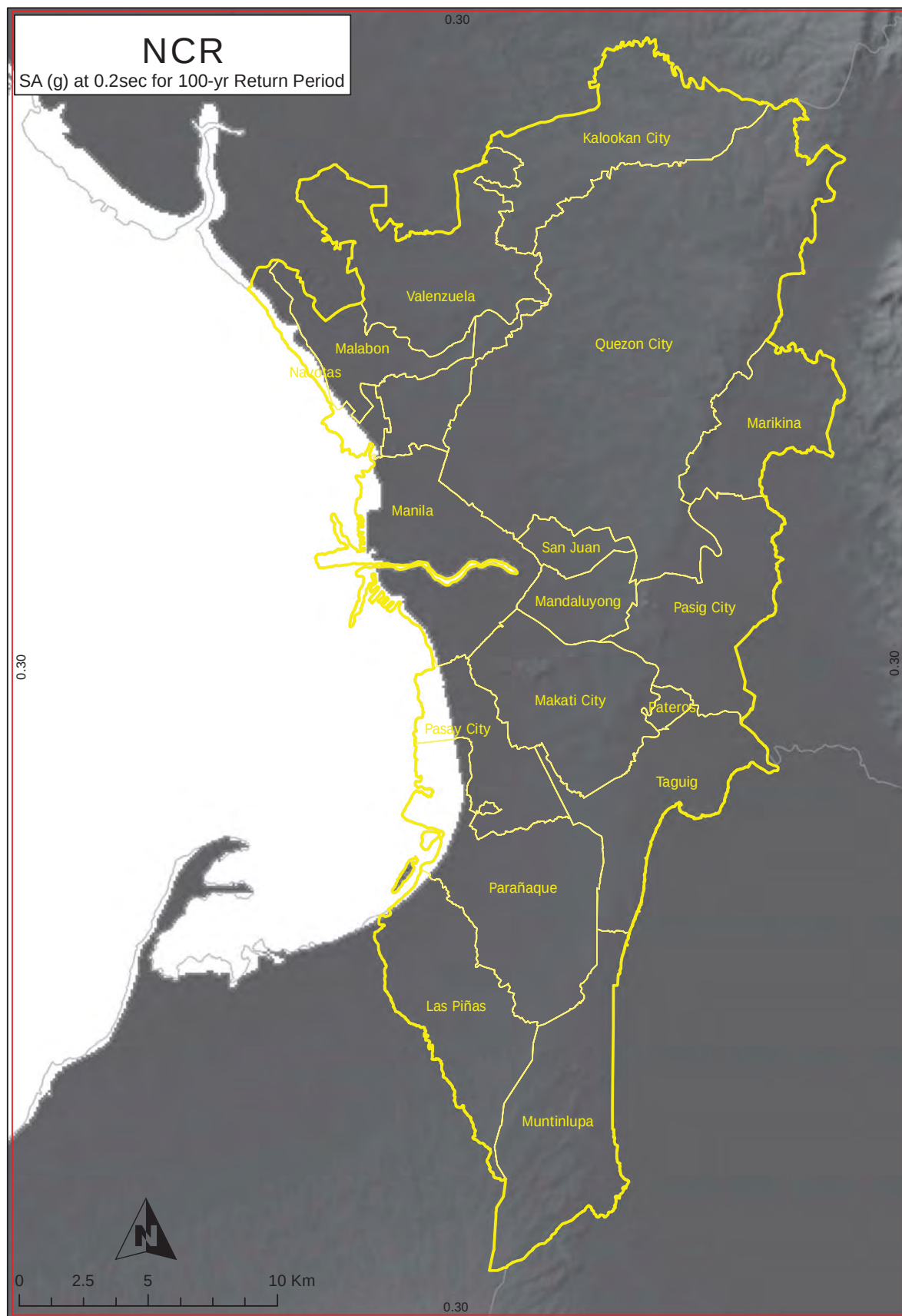
Figure 2A-147 NCR map of spectral acceleration at 0.2 sec. for 100-year return period
